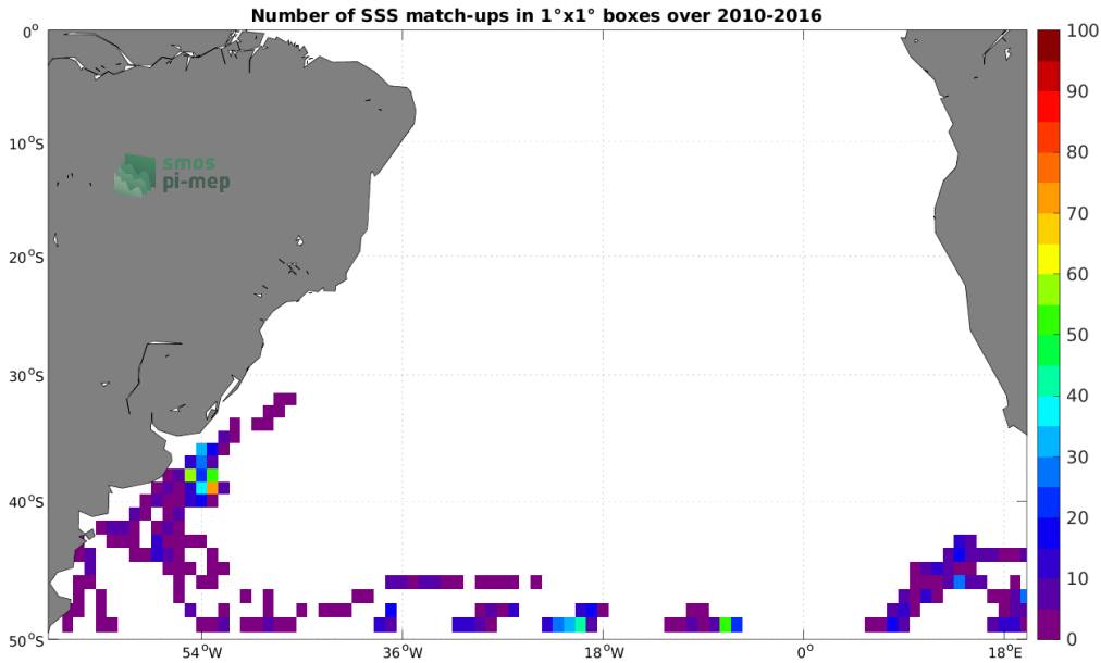
Figure 4: Number of SSS match-ups between Marine mammals SSS and the SMOS SSS L4 v1 - Monthly (CMEMS-CNR) SSS product for the South Atlantic Ocean Pi-MEP region over 1^\circ \times 1^\circ boxes and for the full satellite product period.
