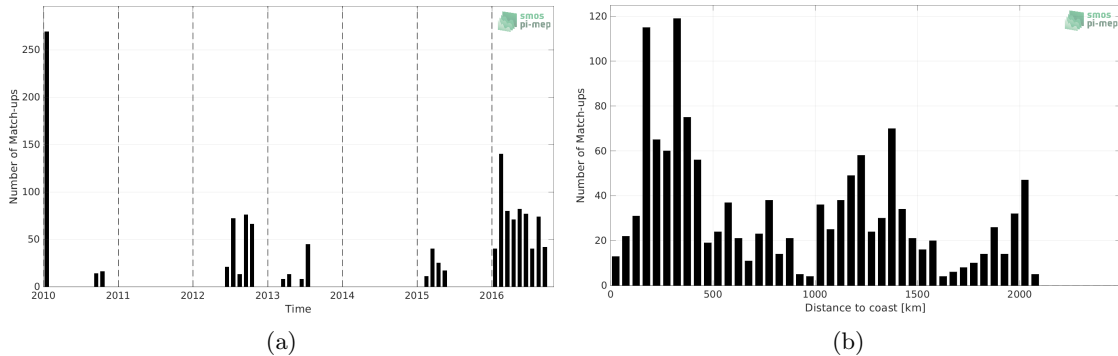
Figure 1: Number of match-ups between Marine mammals and SMOS SSS L4 v1 - Monthly (CMEMS-CNR) SSS as a function of time (a) and as function of the distance to coast (b) over the South Atlantic Ocean Pi-MEP region and for the full satellite product period.
