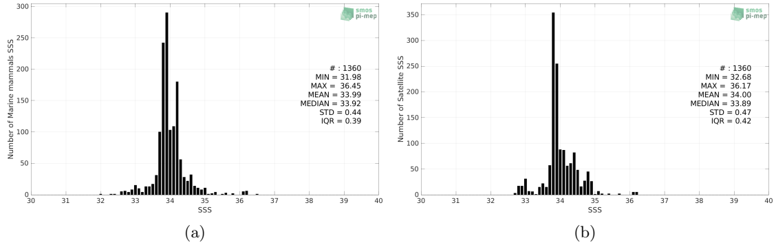
Figure 2: Histograms of SSS from Marine mammals (a) and SMOS SSS L4 v1 - Monthly (CMEMS-CNR) (b) considering all match-up pairs per bins of 0.1 over the South Atlantic Ocean Pi-MEP region and for the full satellite product period.
