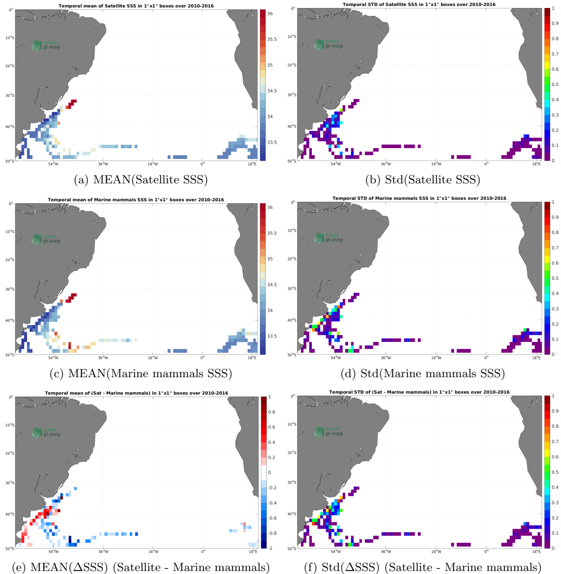
Figure 6: Temporal mean (left) and Std (right) of SSS from SMOS SSS L4 v1 - Monthly (CMEMS-CNR) (top), Marine mammals (middle), and of \Delta SSS (Satellite - Marine mammals). Only match-up pairs are used to generate these maps.
