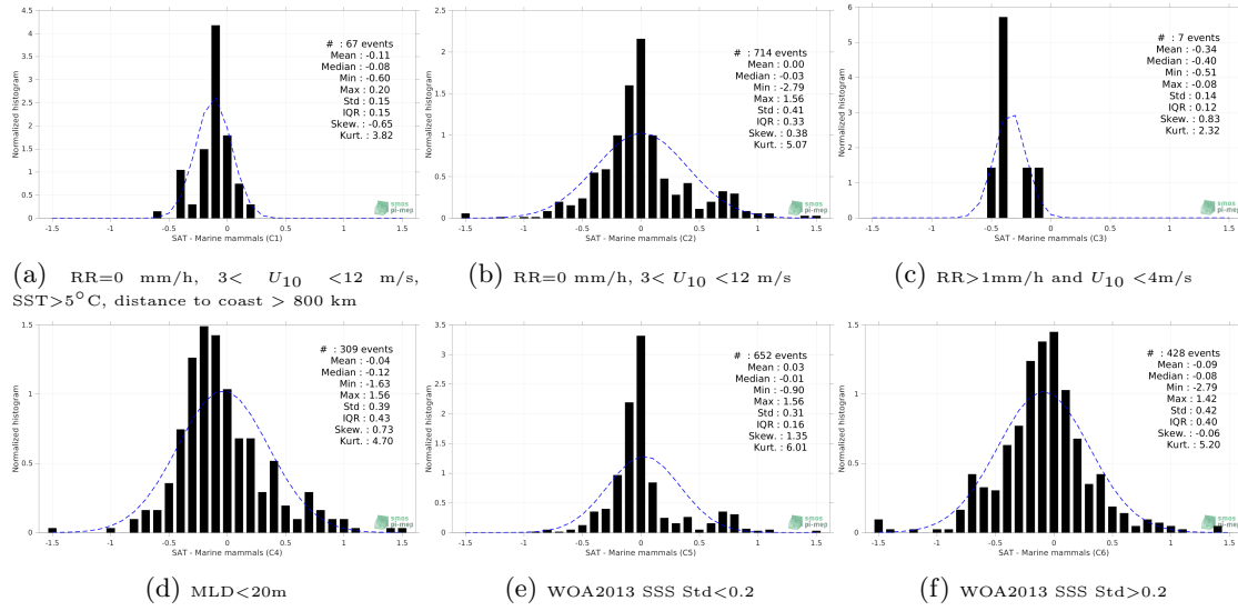
Figure 13: Normalized histogram of \Delta\text{SSS} (SMOS SSS L4 v1 - Monthly (CMEMS-CNR) - Marine mammals) for 6 different subdatasets corresponding to: RR=0 mm/h, 3 < U_{10} < 12 m/s, SST >5^{\circ}\text{C} , distance to coast > 800 km (a), RR=0 mm/h, 3 < U_{10} < 12 m/s (b), RR>1\text{mm/h} and U_{10} < 4\text{m/s} (c), MLD<20\text{m} (d), WOA2013 SSS Std <0.2 (e), WOA2013 SSS Std >0.2 (f).
