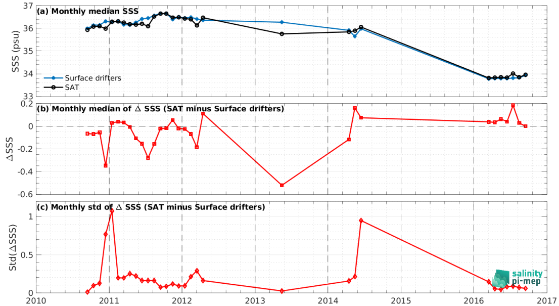
Figure 7: Time series of the monthly median SSS (top), median of \Delta\text{SSS} (Satellite - Surface drifters) and Std of \Delta\text{SSS} (Satellite - Surface drifters) over the South Atlantic Ocean Pi-MEP region considering all match-ups collected by the Pi-MEP.
