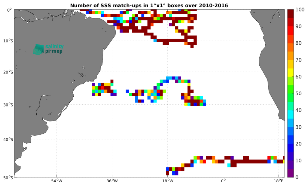
Figure 4: Number of SSS match-ups between Surface drifters SSS and the SMOS SSS L4 v1 - Monthly (CMEMS-CNR) SSS product for the South Atlantic Ocean Pi-MEP region over 1^\circ \times 1^\circ boxes and for the full satellite product period.
