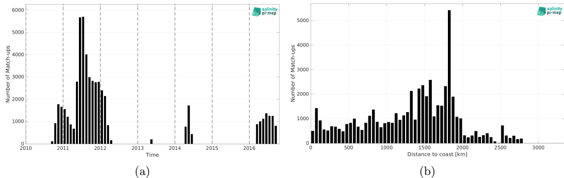
Figure 2: Number of match-ups between Surface drifters and SMOS SSS L4 v1 - Monthly (CMEMS-CNR) SSS as a function of time (a) and as function of the distance to coast (b) over the South Atlantic Ocean Pi-MEP region and for the full satellite product period.
