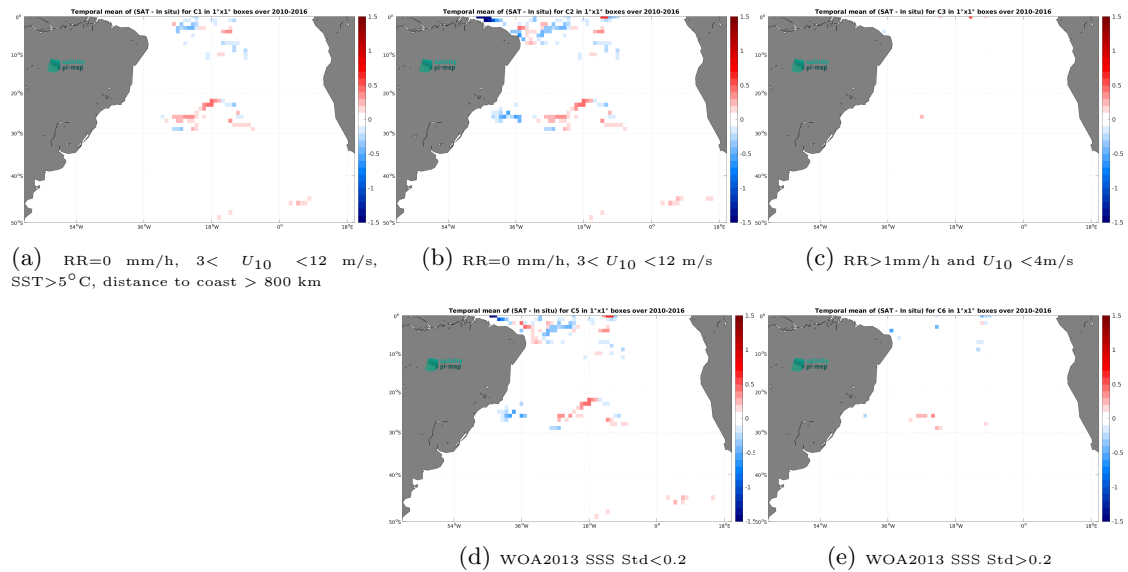
Figure 13: Temporal mean gridded over spatial boxes of size 1^\circ \times 1^\circ of \Delta SSS (SMOS SSS L4 v1 - Monthly (CMEMS-CNR) - Surface drifters) for 5 different subdatasets corresponding to: RR=0 mm/h, 3 < U_{10} < 12 m/s, SST > 5^\circ C , distance to coast > 800 km (a), RR=0 mm/h, 3 < U_{10} < 12 m/s (b), RR > 1 mm/h and U_{10} < 4 m/s (c), WOA2013 SSS Std < 0.2 (d), WOA2013 SSS Std > 0.2 (e).
