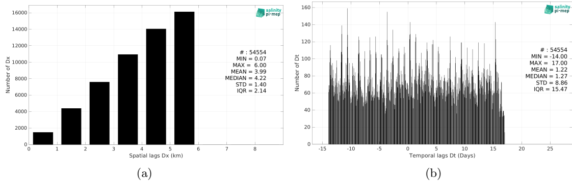
Figure 5: Histograms of the spatial (a) and temporal (b) lags between the location/time of the Surface drifters measurement and the date of the corresponding SMOS SSS L4 v1 - Monthly (CMEMS-CNR) SSS pixel.
