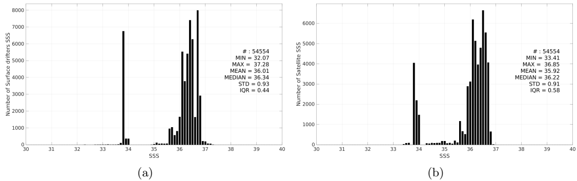
Figure 3: Histograms of SSS from Surface drifters (a) and SMOS SSS L4 v1 - Monthly (CMEMS-CNR) (b) considering all match-up pairs per bins of 0.1 over the South Atlantic Ocean Pi-MEP region and for the full satellite product period.
