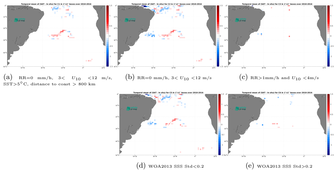
Figure 11: Temporal mean gridded over spatial boxes of size 1^\circ \times 1^\circ of \Delta\text{SSS} (SMOS SSS L4 v1 - Monthly (CMEMS-CNR) - Surface drifters) for 5 different subdatasets corresponding to:RR=0 mm/h, 3 < U_{10} < 12 m/s, SST >5^\circ\text{C} , distance to coast > 800 km (a), RR=0 mm/h, 3 < U_{10} < 12 m/s (b), RR >1 mm/h and U_{10} < 4 m/s (c), WOA2013 SSS Std <0.2 (d), WOA2013 SSS Std >0.2 (e).
