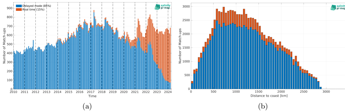
Figure 2: Number of match-ups between Argo and SMOS SSS L4 v1 - Monthly (CMEMS-CNR) SSS as a function of time (a) and as function of the distance to coast (b) over the South Atlantic Ocean Pi-MEP region and for the full satellite product period.
