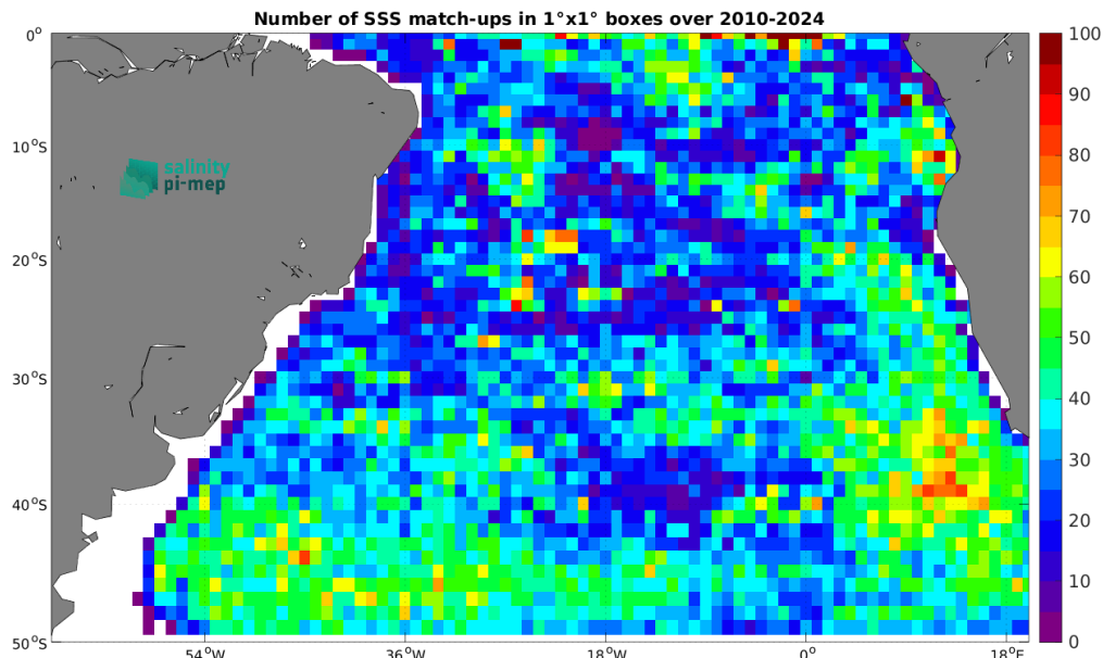
Figure 5: Number of SSS match-ups between Argo SSS and the SMOS SSS L4 v1 - Monthly (CMEMS-CNR) SSS product for the South Atlantic Ocean Pi-MEP region over 1^\circ \times 1^\circ boxes and for the full satellite product period.
