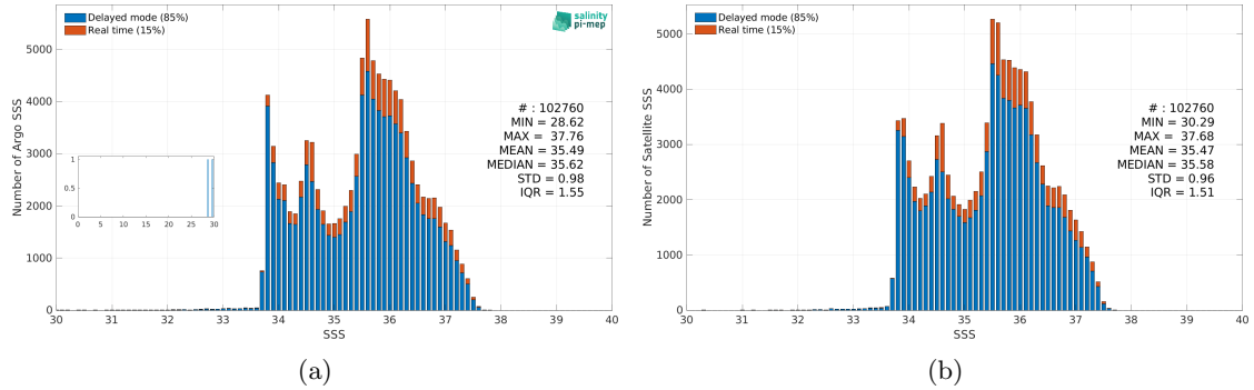
Figure 3: Histograms of SSS from Argo (a) and SMOS SSS L4 v1 - Monthly (CMEMS-CNR) (b) considering all match-up pairs per bins of 0.1 over the South Atlantic Ocean Pi-MEP region and for the full satellite product period.
