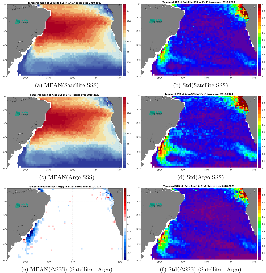
Figure 6: Temporal mean (left) and Std (right) of SSS from SMOS SSS L4 v1 - Monthly (CMEMS-CNR) (top), Argo in situ dataset (middle), and of \Delta SSS (Satellite - Argo). Only match-up pairs are used to generate these maps.
