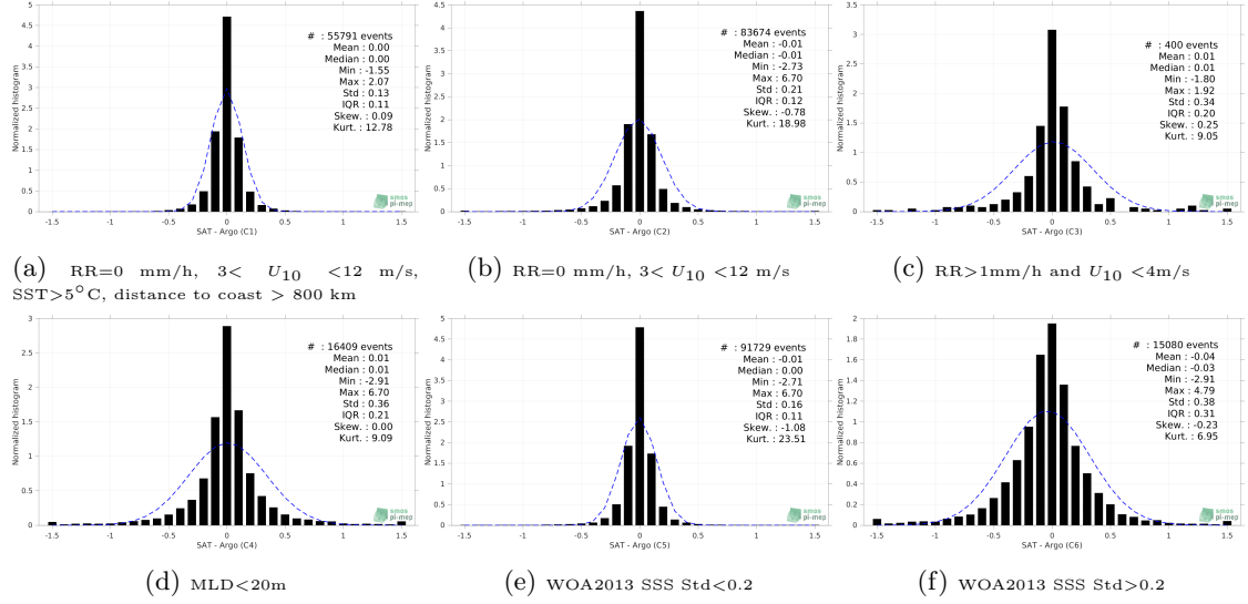
Figure 13: Normalized histogram of \Delta SSS (SMOS SSS L4 v1 - Monthly (CMEMS-CNR) - Argo) for 6 different subdatasets corresponding to: RR=0 mm/h, 3 < U_{10} < 12 m/s, SST>5°C, distance to coast > 800 km (a), RR=0 mm/h, 3 < U_{10} < 12 m/s (b), RR>1mm/h and U_{10} < 4 m/s (c), MLD<20m (d), WOA2013 SSS Std<0.2 (e), WOA2013 SSS Std>0.2 (f).
