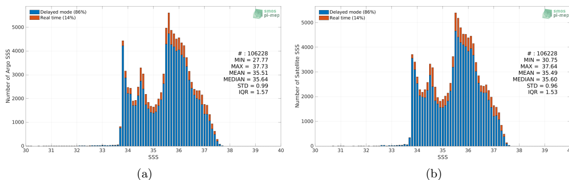
Figure 2: Histograms of SSS from Argo (a) and SMOS SSS L4 v1 - Monthly (CMEMS-CNR) (b) considering all match-up pairs per bins of 0.1 over the South Atlantic Ocean Pi-MEP region and for the full satellite product period.
