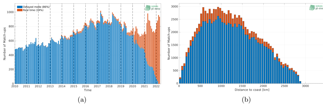
Figure 1: Number of match-ups between Argo and SMOS SSS L4 v1 - Monthly (CMEMS-CNR) SSS as a function of time (a) and as function of the distance to coast (b) over the South Atlantic Ocean Pi-MEP region and for the full satellite product period.
