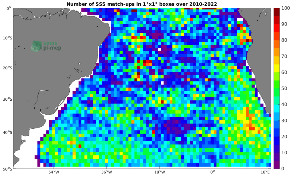
Figure 4: Number of SSS match-ups between Argo SSS and the SMOS SSS L4 v1 - Monthly (CMEMS-CNR) SSS product for the South Atlantic Ocean Pi-MEP region over 1^\circ \times 1^\circ boxes and for the full satellite product period.
