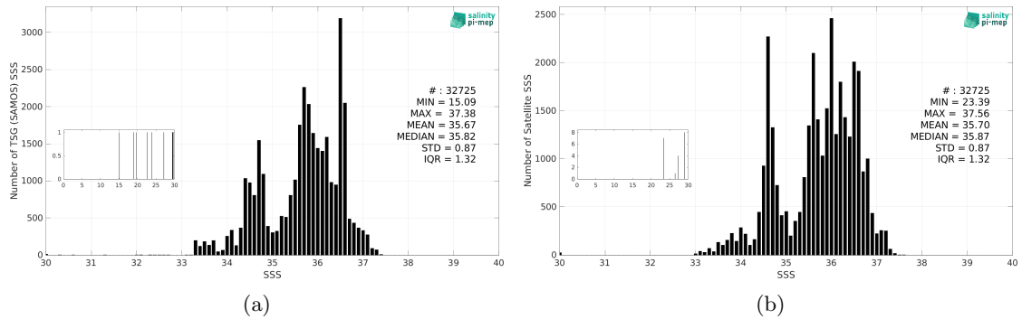
Figure 3: Histograms of SSS from TSG (SAMOS) (a) and SMOS SSS L4 v1 - Daily (CMEMS-CNR) (b) considering all match-up pairs per bins of 0.1 over the South Atlantic Ocean Pi-MEP region and for the full satellite product period.
