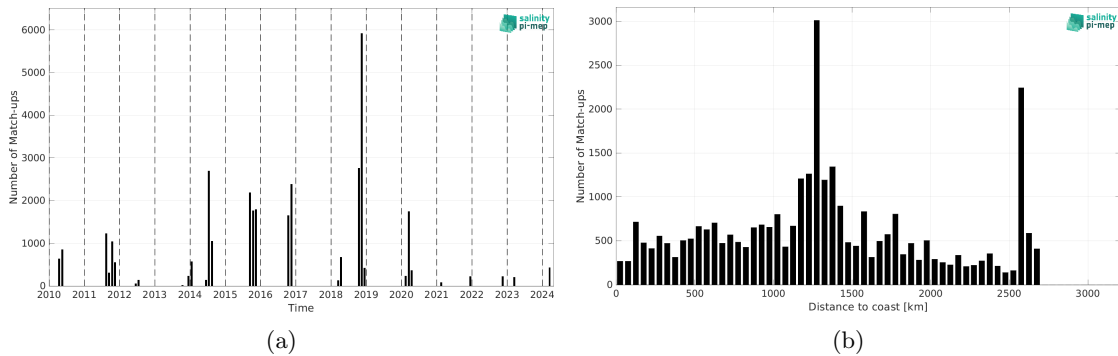
Figure 2: Number of match-ups between TSG (SAMOS) and SMOS SSS L4 v1 - Daily (CMEMS-CNR) SSS as a function of time (a) and as function of the distance to coast (b) over the South Atlantic Ocean Pi-MEP region and for the full satellite product period.
