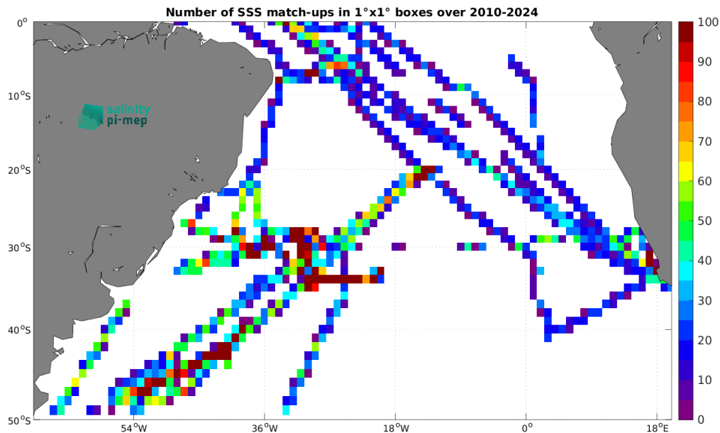
Figure 5: Number of SSS match-ups between TSG (SAMOS) SSS and the SMOS SSS L4 v1 - Daily (CMEMS-CNR) SSS product for the South Atlantic Ocean Pi-MEP region over 1^\circ \times 1^\circ boxes and for the full satellite product period.
