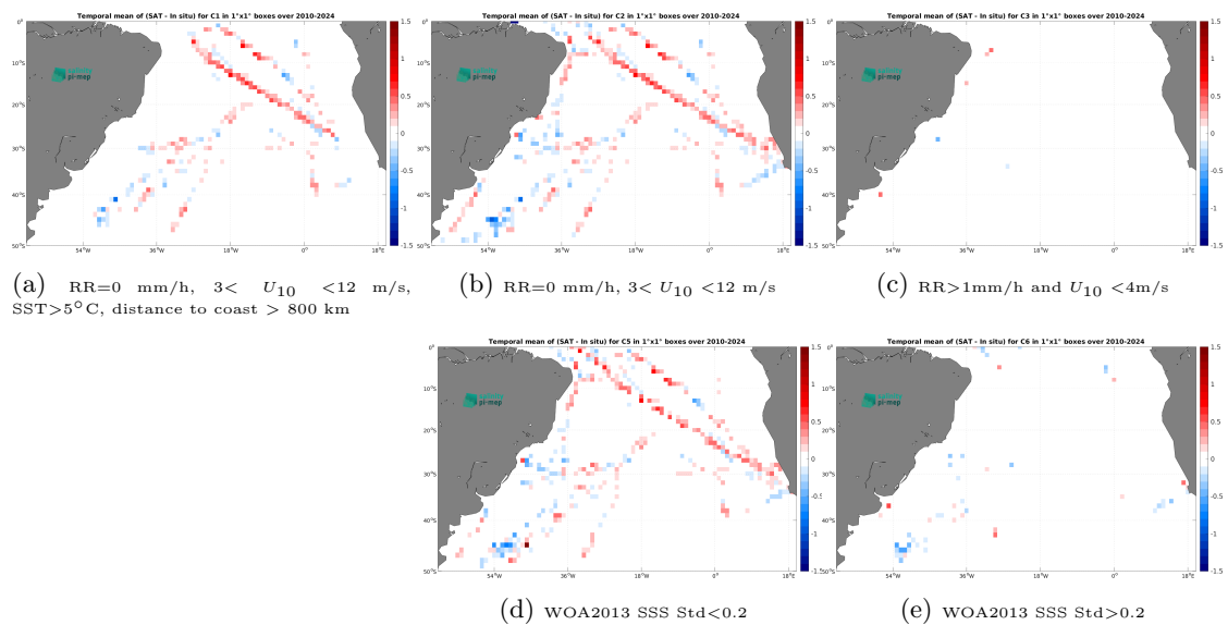
Figure 14: Temporal mean gridded over spatial boxes of size 1^\circ \times 1^\circ of \Delta SSS (SMOS SSS L4 v1 - Daily (CMEMS-CNR) - TSG (SAMOS)) for 5 different subdatasets corresponding to:RR=0 mm/h, 3 < U_{10} < 12 m/s, SST >5^\circ\text{C} , distance to coast > 800 km (a), RR=0 mm/h, 3 < U_{10} < 12 m/s (b), RR >1 mm/h and U_{10} < 4 m/s (c), WOA2013 SSS Std <0.2 (d), WOA2013 SSS Std >0.2 (e).
