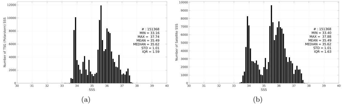
Figure 3: Histograms of SSS from TSG (Polarstern) (a) and SMOS SSS L4 v1 - Daily (CMEMS-CNR) (b) considering all match-up pairs per bins of 0.1 over the South Atlantic Ocean Pi-MEP region and for the full satellite product period.
