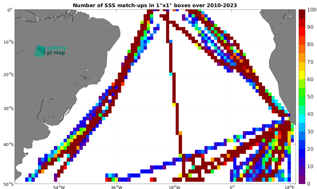
Figure 5: Number of SSS match-ups between TSG (Polarstern) SSS and the SMOS SSS L4 v1 - Daily (CMEMS-CNR) SSS product for the South Atlantic Ocean Pi-MEP region over 1^\circ \times 1^\circ boxes and for the full satellite product period.
