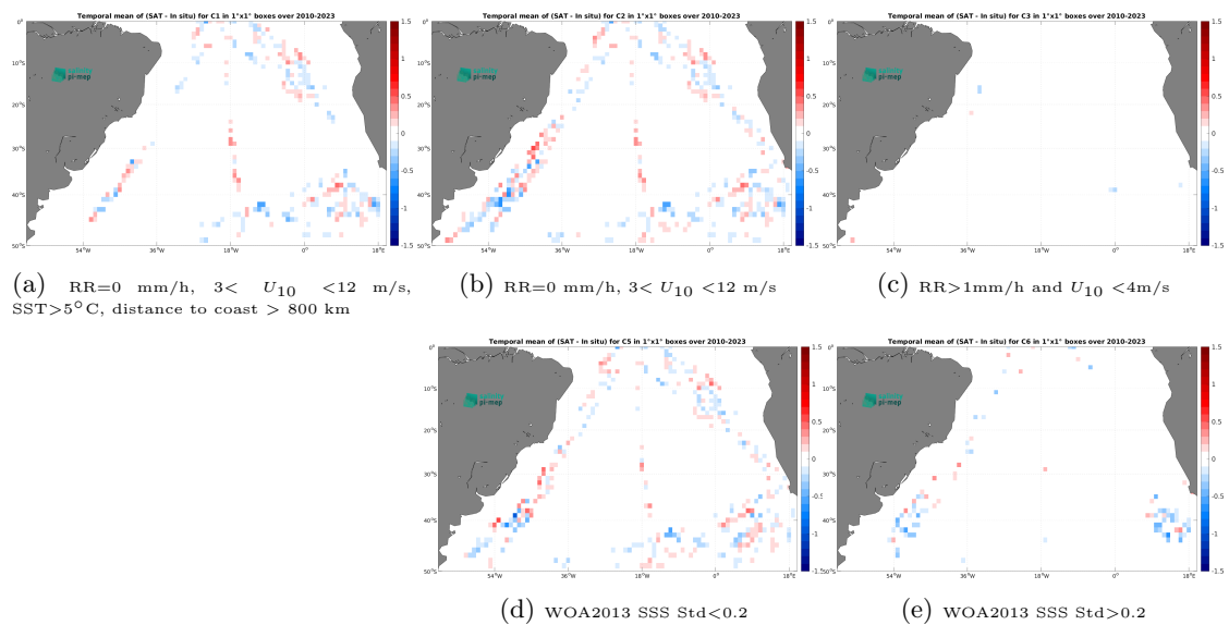
Figure 14: Temporal mean gridded over spatial boxes of size 1^\circ \times 1^\circ of \Delta SSS (SMOS SSS L4 v1 - Daily (CMEMS-CNR) - TSG (Polarstern)) for 5 different subdatasets corresponding to:RR=0 mm/h, 3 < U_{10} < 12 m/s, SST >5^\circ\text{C} , distance to coast > 800 km (a), RR=0 mm/h, 3 < U_{10} < 12 m/s (b), RR >1 mm/h and U_{10} < 4 m/s (c), WOA2013 SSS Std <0.2 (d), WOA2013 SSS Std >0.2 (e).
