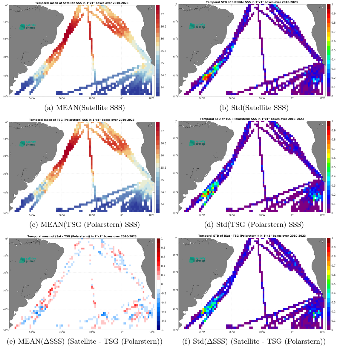
Figure 7: Temporal mean (left) and Std (right) of SSS from SMOS SSS L4 v1 - Daily (CMEMS-CNR) (top), TSG (Polarstern) (middle), and of \Delta SSS (Satellite - TSG (Polarstern)). Only match-up pairs are used to generate these maps.
