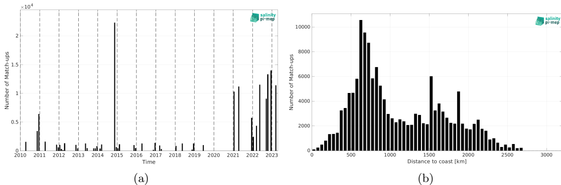
Figure 2: Number of match-ups between TSG (Polarstern) and SMOS SSS L4 v1 - Daily (CMEMS-CNR) SSS as a function of time (a) and as function of the distance to coast (b) over the South Atlantic Ocean Pi-MEP region and for the full satellite product period.
