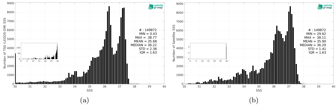
Figure 3: Histograms of SSS from TSG (LEGOS-DM) (a) and SMOS SSS L4 v1 - Daily (CMEMS-CNR) (b) considering all match-up pairs per bins of 0.1 over the South Atlantic Ocean Pi-MEP region and for the full satellite product period.
