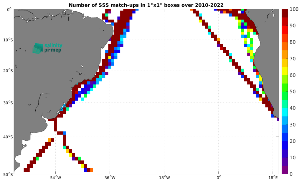
Figure 5: Number of SSS match-ups between TSG (LEGOS-DM) SSS and the SMOS SSS L4 v1 - Daily (CMEMS-CNR) SSS product for the South Atlantic Ocean Pi-MEP region over 1^\circ \times 1^\circ boxes and for the full satellite product period.
