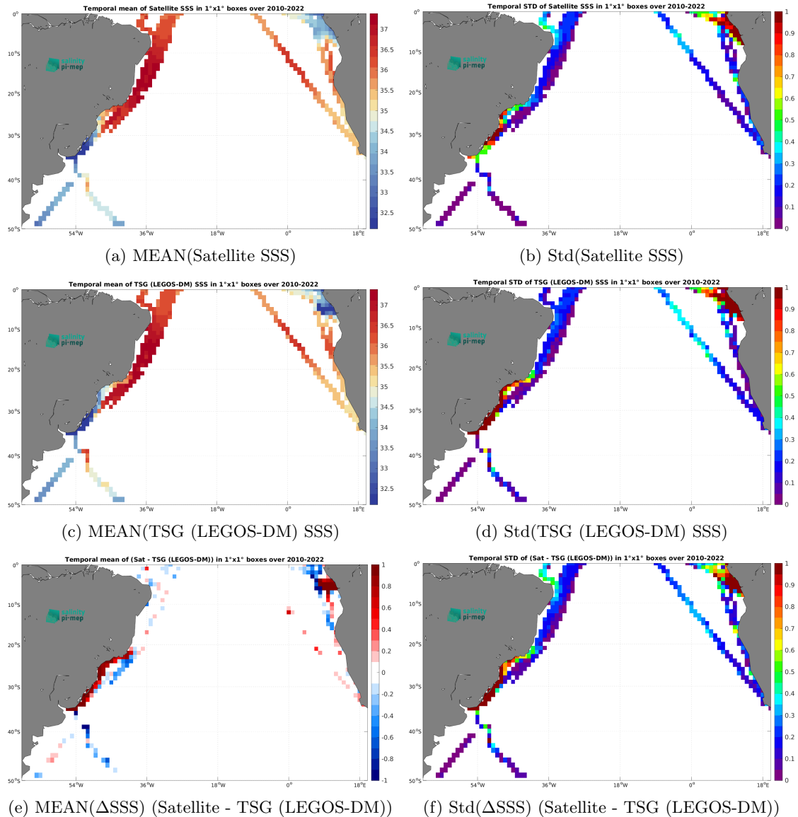
Figure 7: Temporal mean (left) and Std (right) of SSS from SMOS SSS L4 v1 - Daily (CMEMS-CNR) (top), TSG (LEGOS-DM) (middle), and of \Delta SSS (Satellite - TSG (LEGOS-DM)). Only match-up pairs are used to generate these maps.
