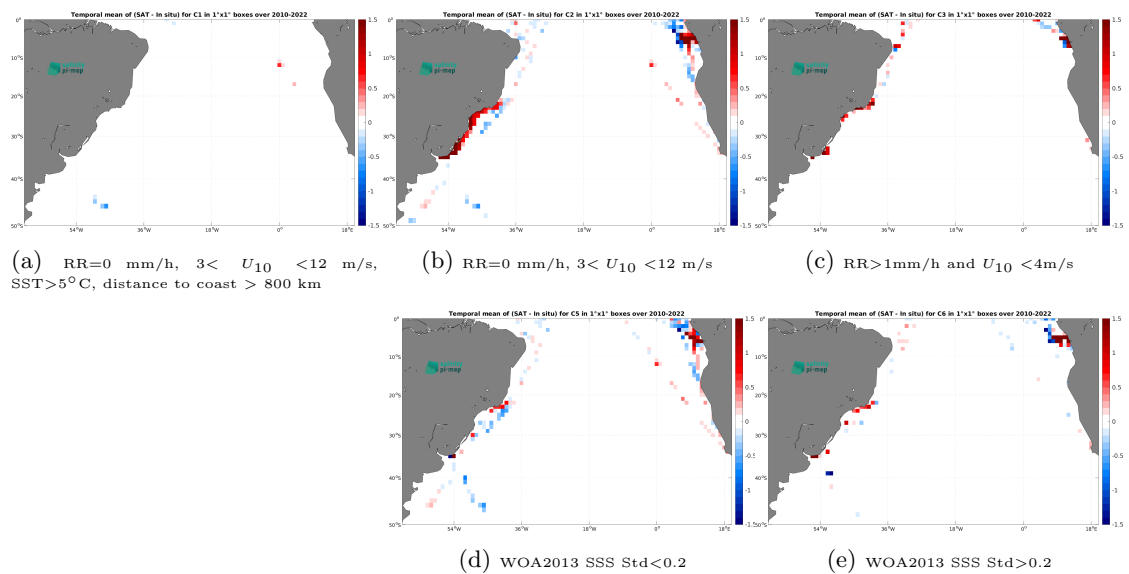
Figure 14: Temporal mean gridded over spatial boxes of size 1^\circ \times 1^\circ of \Delta SSS (SMOS SSS L4 v1 - Daily (CMEMS-CNR) - TSG (LEGOS-DM)) for 5 different subdatasets corresponding to:RR=0 mm/h, 3 < U_{10} < 12 m/s, SST > 5°C, distance to coast > 800 km (a), RR=0 mm/h, 3 < U_{10} < 12 m/s (b), RR > 1mm/h and U_{10} < 4 m/s (c), WOA2013 SSS Std < 0.2 (d), WOA2013 SSS Std > 0.2 (e).
