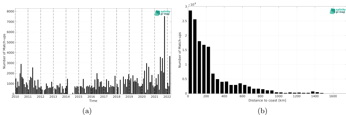
Figure 2: Number of match-ups between TSG (LEGOS-DM) and SMOS SSS L4 v1 - Daily (CMEMS-CNR) SSS as a function of time (a) and as function of the distance to coast (b) over the South Atlantic Ocean Pi-MEP region and for the full satellite product period.
