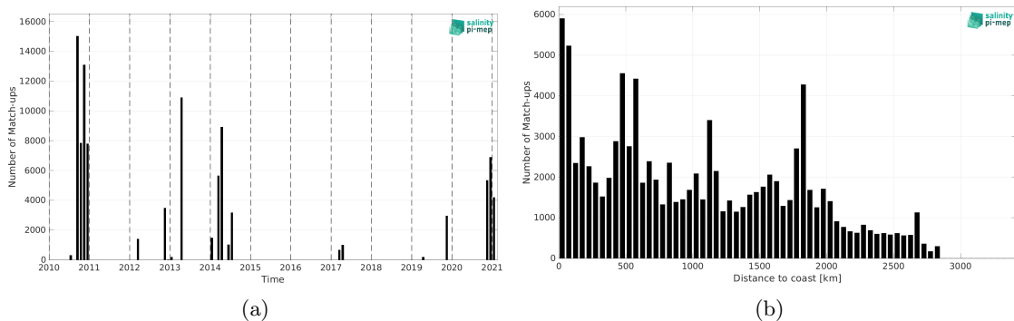
Figure 2: Number of match-ups between TSG (GOSUD-Sailing-ship) and SMOS SSS L4 v1 - Daily (CMEMS-CNR) SSS as a function of time (a) and as function of the distance to coast (b) over the South Atlantic Ocean Pi-MEP region and for the full satellite product period.
