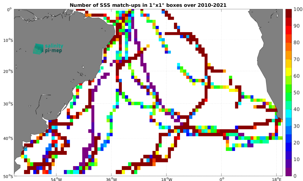
Figure 5: Number of SSS match-ups between TSG (GOSUD-Sailing-ship) SSS and the SMOS SSS L4 v1 - Daily (CMEMS-CNR) SSS product for the South Atlantic Ocean Pi-MEP region over 1^\circ \times 1^\circ boxes and for the full satellite product period.
