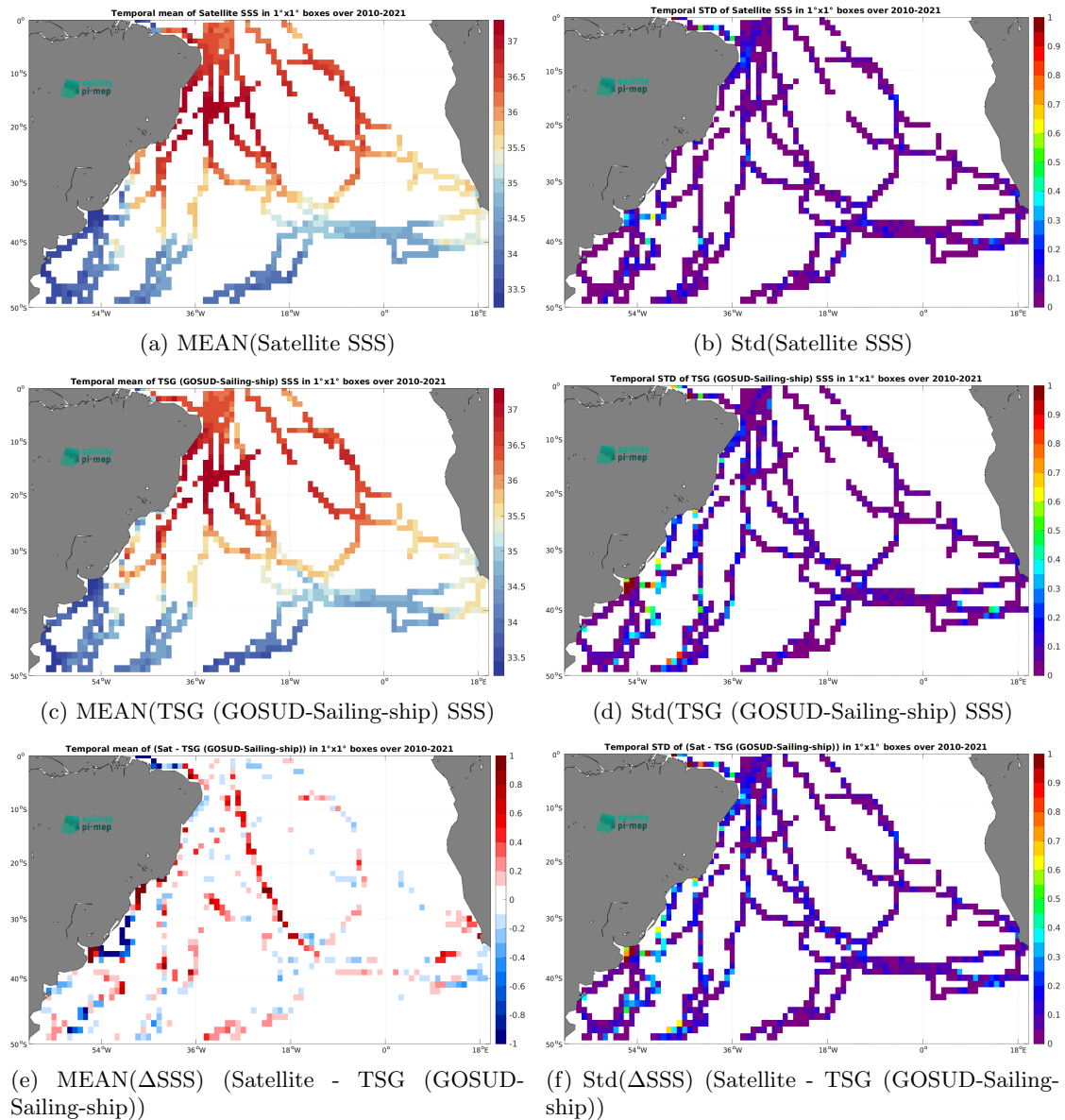
Figure 7: Temporal mean (left) and Std (right) of SSS from SMOS SSS L4 v1 - Daily (CMEMS-CNR) (top), TSG (GOSUD-Sailing-ship) (middle), and of \Delta SSS (Satellite - TSG (GOSUD-Sailing-ship)). Only match-up pairs are used to generate these maps.
