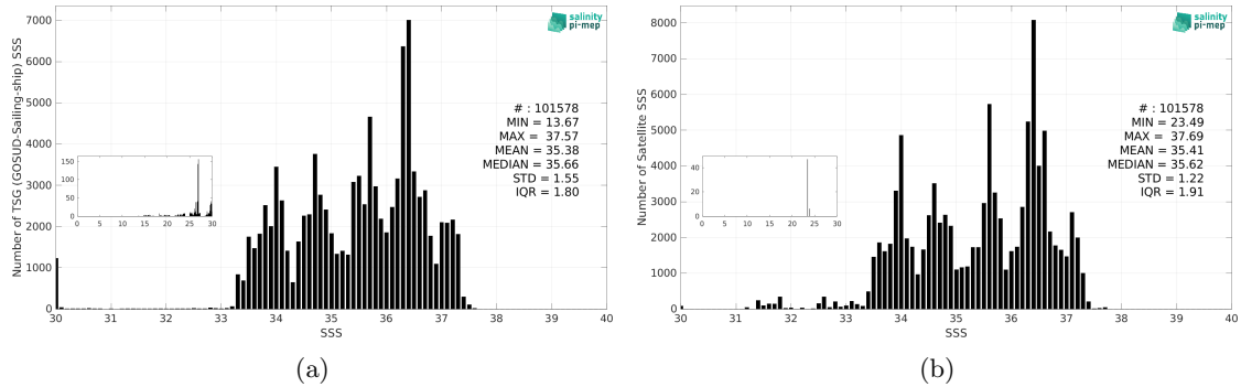
Figure 3: Histograms of SSS from TSG (GOSUD-Sailing-ship) (a) and SMOS SSS L4 v1 - Daily (CMEMS-CNR) (b) considering all match-up pairs per bins of 0.1 over the South Atlantic Ocean Pi-MEP region and for the full satellite product period.
