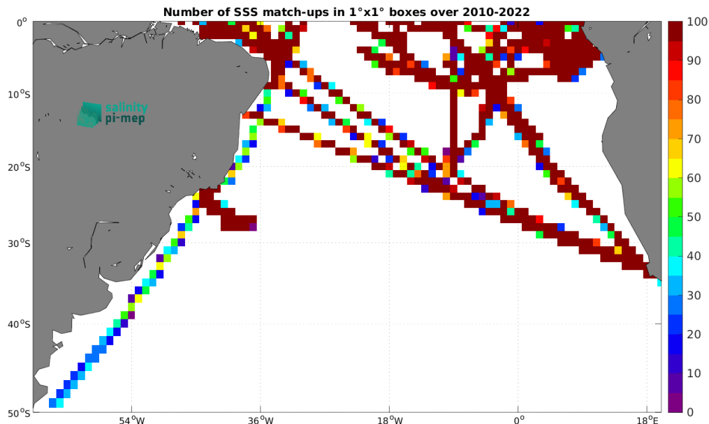
Figure 5: Number of SSS match-ups between TSG (GOSUD-Research-vessel) SSS and the SMOS SSS L4 v1 - Daily (CMEMS-CNR) SSS product for the South Atlantic Ocean Pi-MEP region over 1^\circ \times 1^\circ boxes and for the full satellite product period.
