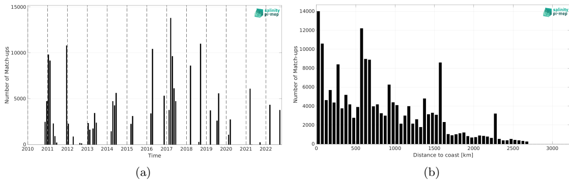
Figure 2: Number of match-ups between TSG (GOSUD-Research-vessel) and SMOS SSS L4 v1 - Daily (CMEMS-CNR) SSS as a function of time (a) and as function of the distance to coast (b) over the South Atlantic Ocean Pi-MEP region and for the full satellite product period.
