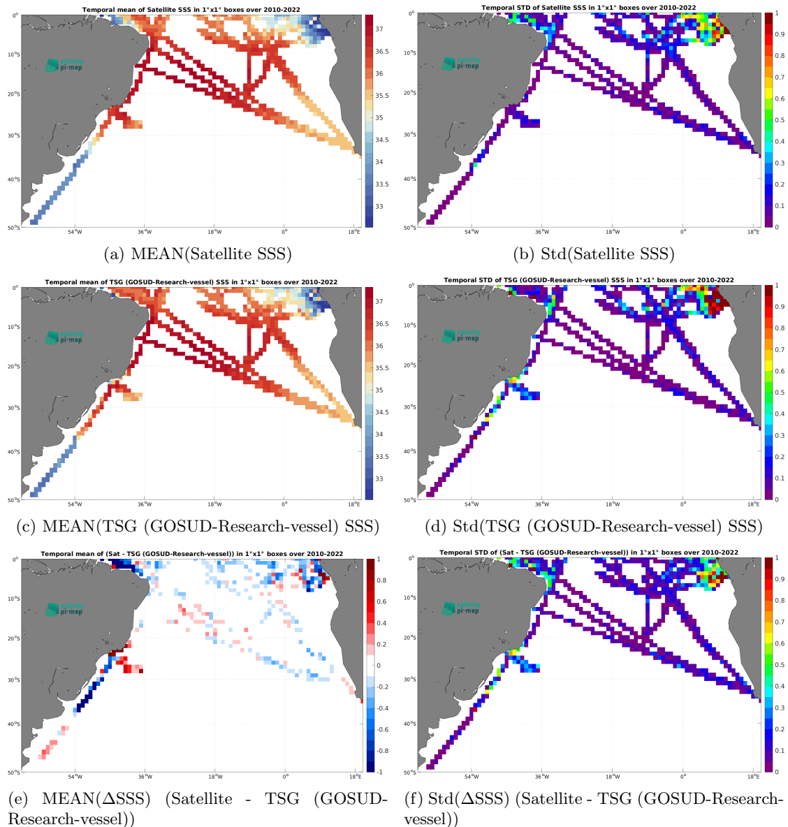
Figure 7: Temporal mean (left) and Std (right) of SSS from SMOS SSS L4 v1 - Daily (CMEMS-CNR) (top), TSG (GOSUD-Research-vessel) (middle), and of \Delta SSS (Satellite - TSG (GOSUD-Research-vessel)). Only match-up pairs are used to generate these maps.
