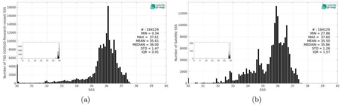
Figure 3: Histograms of SSS from TSG (GOSUD-Research-vessel) (a) and SMOS SSS L4 v1 - Daily (CMEMS-CNR) (b) considering all match-up pairs per bins of 0.1 over the South Atlantic Ocean Pi-MEP region and for the full satellite product period.
