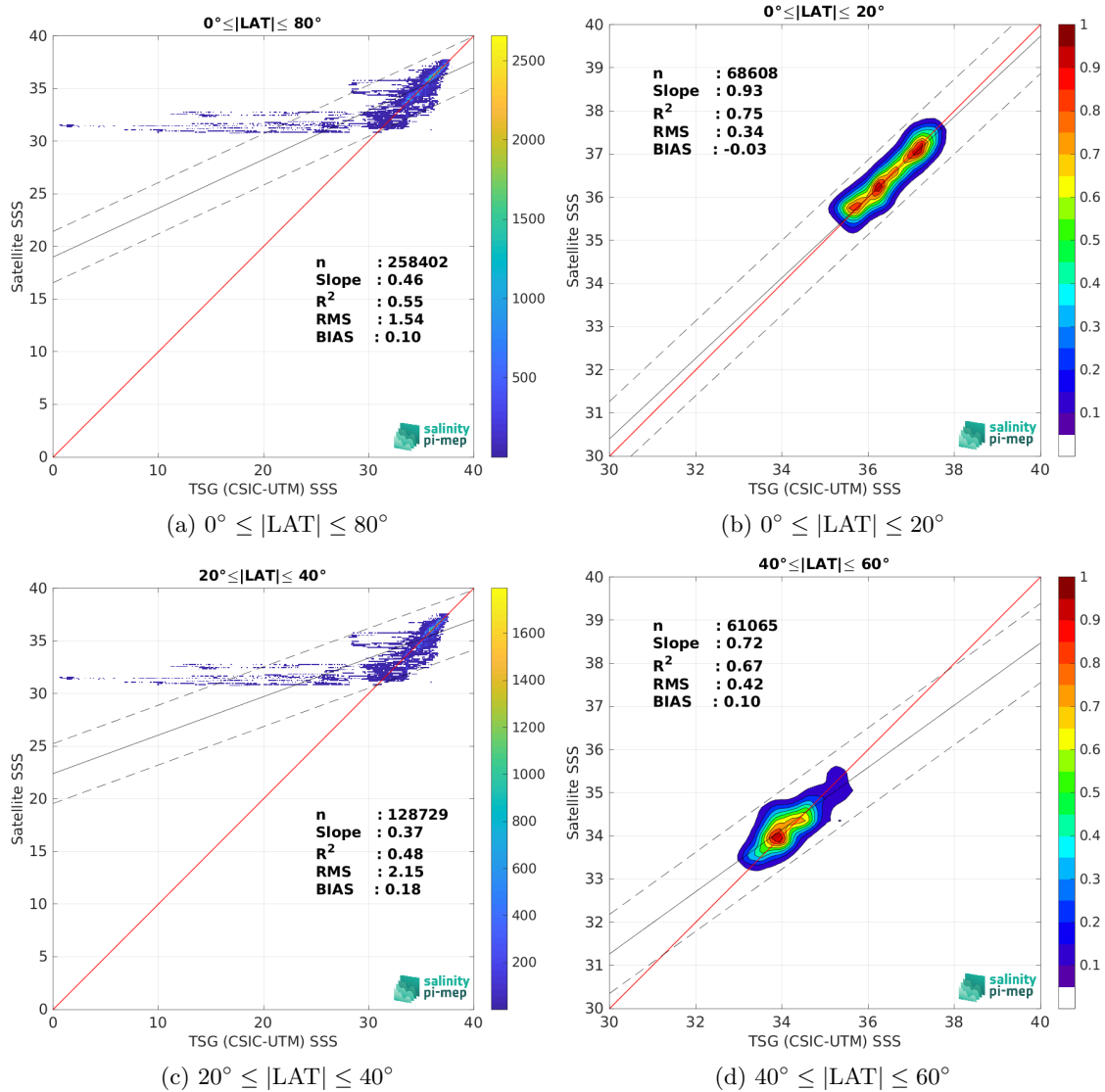
Figure 10: Contour maps of the concentration of SMOS SSS L4 v1 - Daily (CMEMS-CNR) SSS (y-axis) versus TSG (CSIC-UTM) SSS (x-axis) at match-up pairs for different latitude bands. For each plot, the red line shows x=y . The black thin and dashed lines indicate a linear fit through the data cloud and the \pm 95\% confidence levels, respectively. The number match-up pairs n , the slope and R^2 coefficient of the linear fit, the root mean square (RMS) and the mean bias between satellite and in situ data are indicated for each latitude band in each plots.
