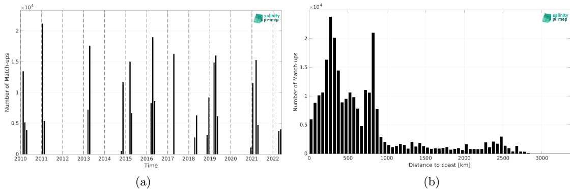
Figure 2: Number of match-ups between TSG (CSIC-UTM) and SMOS SSS L4 v1 - Daily (CMEMS-CNR) SSS as a function of time (a) and as function of the distance to coast (b) over the South Atlantic Ocean Pi-MEP region and for the full satellite product period.
