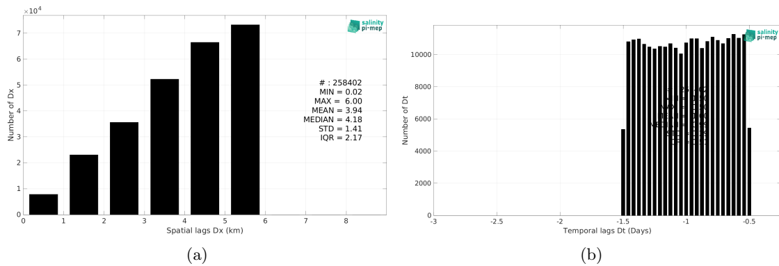
Figure 6: Histograms of the spatial (a) and temporal (b) lags between the location/time of the TSG (CSIC-UTM) measurement and the date of the corresponding SMOS SSS L4 v1 - Daily (CMEMS-CNR) SSS pixel.
