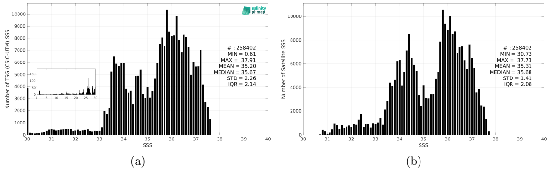
Figure 3: Histograms of SSS from TSG (CSIC-UTM) (a) and SMOS SSS L4 v1 - Daily (CMEMS-CNR) (b) considering all match-up pairs per bins of 0.1 over the South Atlantic Ocean Pi-MEP region and for the full satellite product period.
