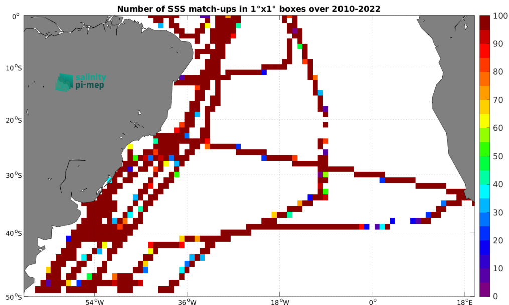
Figure 5: Number of SSS match-ups between TSG (CSIC-UTM) SSS and the SMOS SSS L4 v1 - Daily (CMEMS-CNR) SSS product for the South Atlantic Ocean Pi-MEP region over 1^\circ \times 1^\circ boxes and for the full satellite product period.
