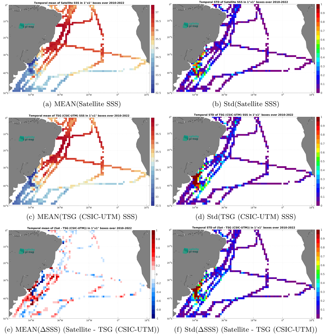
Figure 7: Temporal mean (left) and Std (right) of SSS from SMOS SSS L4 v1 - Daily (CMEMS-CNR) (top), TSG (CSIC-UTM) (middle), and of \Delta SSS (Satellite - TSG (CSIC-UTM)). Only match-up pairs are used to generate these maps.
