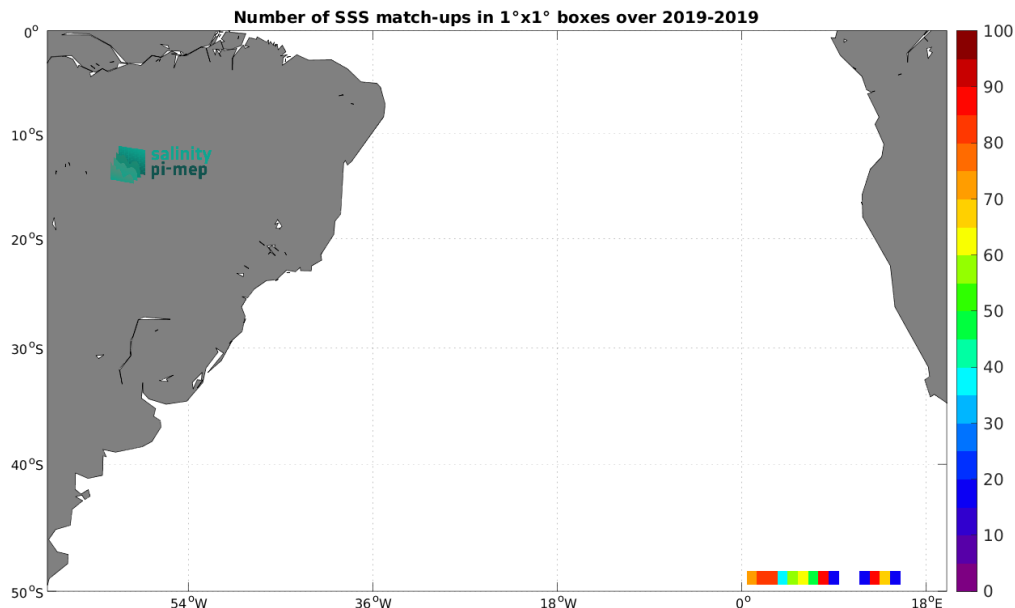
Figure 5: Number of SSS match-ups between Saildrone SSS and the SMOS SSS L4 v1 - Daily (CMEMS-CNR) SSS product for the South Atlantic Ocean Pi-MEP region over 1^\circ \times 1^\circ boxes and for the full satellite product period.
