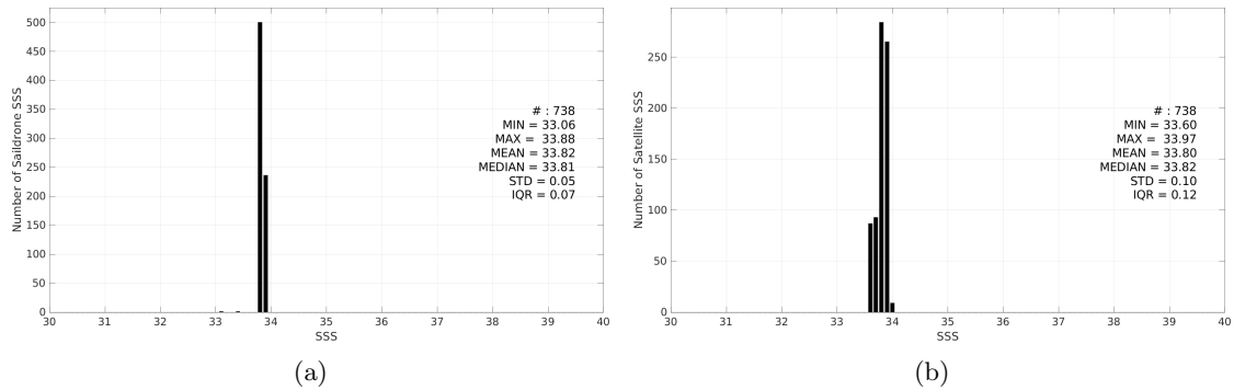
Figure 3: Histograms of SSS from Saildrone (a) and SMOS SSS L4 v1 - Daily (CMEMS-CNR) (b) considering all match-up pairs per bins of 0.1 over the South Atlantic Ocean Pi-MEP region and for the full satellite product period.
