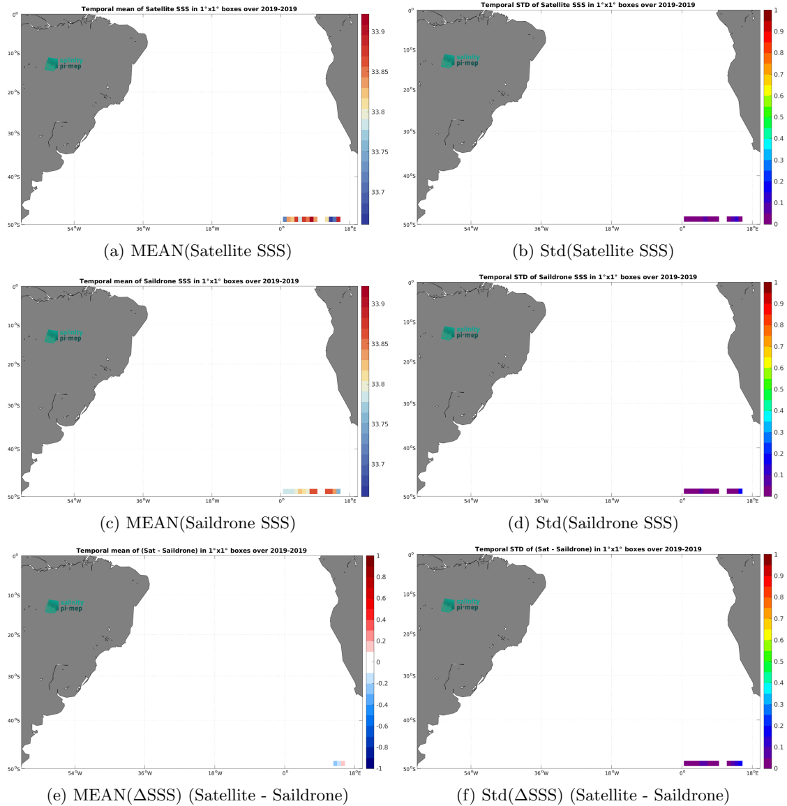
Figure 7: Temporal mean (left) and Std (right) of SSS from SMOS SSS L4 v1 - Daily (CMEMS-CNR) (top), Saildrone (middle), and of \Delta SSS (Satellite - Saildrone). Only match-up pairs are used to generate these maps.
