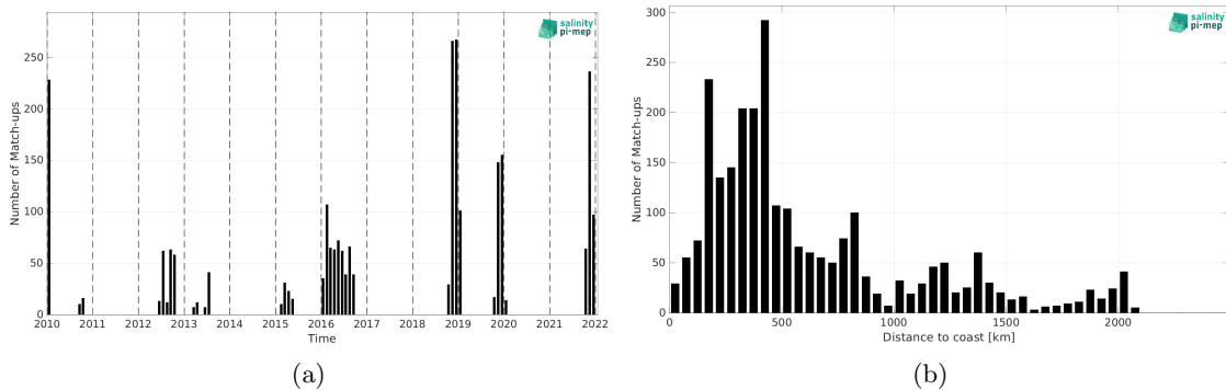
Figure 2: Number of match-ups between Marine mammals and SMOS SSS L4 v1 - Daily (CMEMS-CNR) SSS as a function of time (a) and as function of the distance to coast (b) over the South Atlantic Ocean Pi-MEP region and for the full satellite product period.
