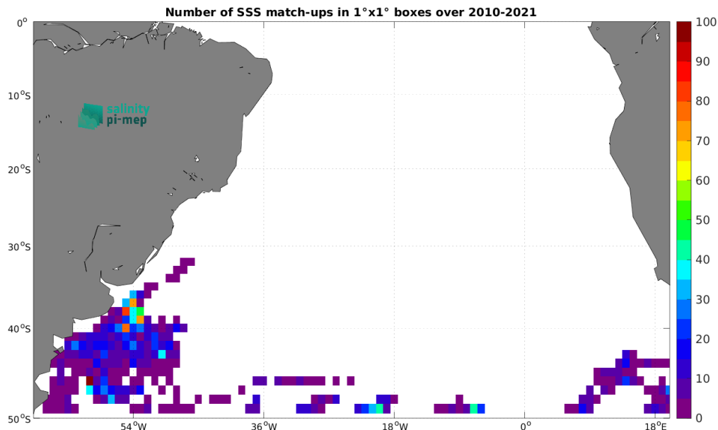
Figure 5: Number of SSS match-ups between Marine mammals SSS and the SMOS SSS L4 v1 - Daily (CMEMS-CNR) SSS product for the South Atlantic Ocean Pi-MEP region over 1^\circ \times 1^\circ boxes and for the full satellite product period.
