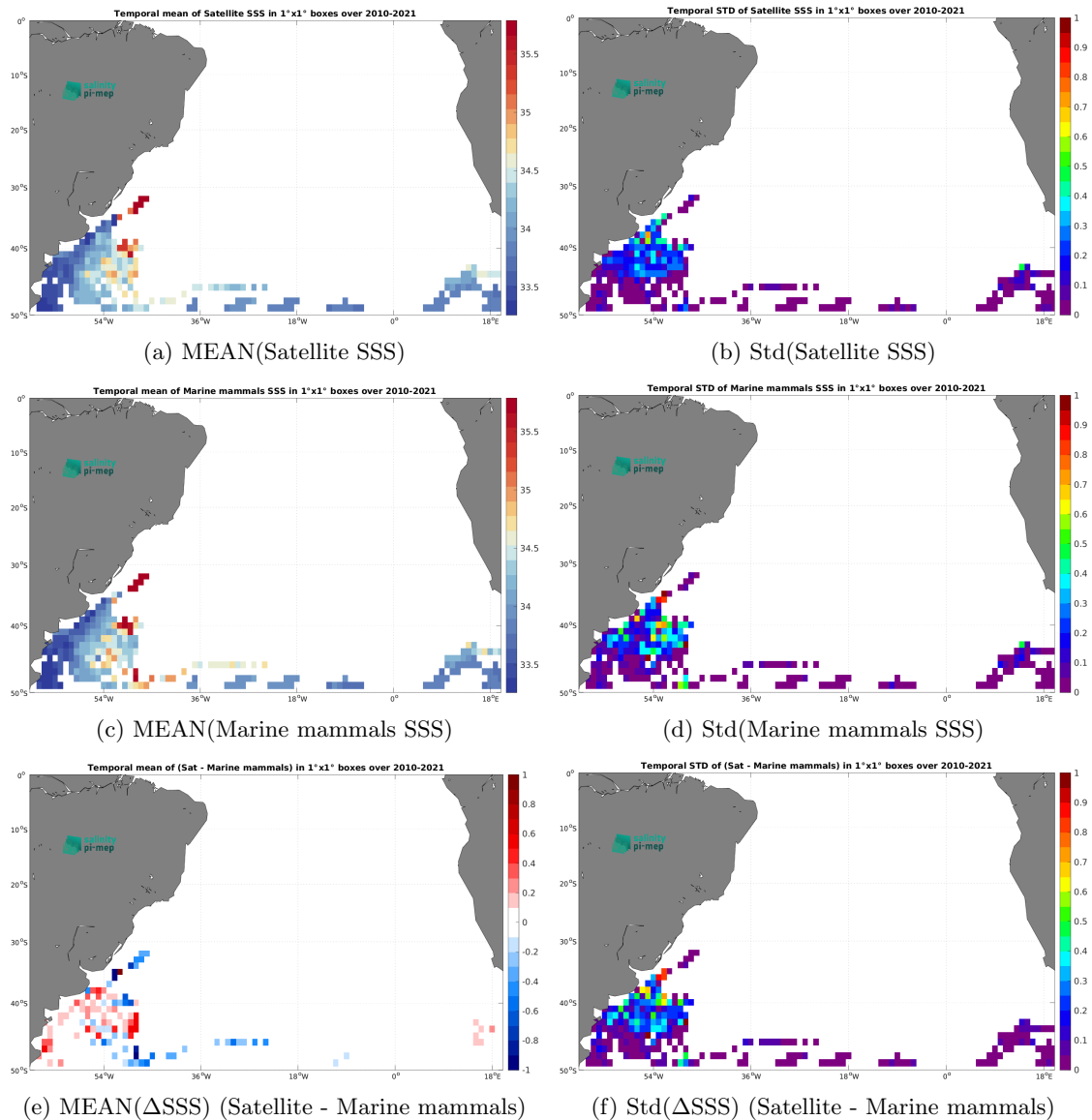
Figure 7: Temporal mean (left) and Std (right) of SSS from SMOS SSS L4 v1 - Daily (CMEMS-CNR) (top), Marine mammals (middle), and of \Delta SSS (Satellite - Marine mammals). Only match-up pairs are used to generate these maps.
