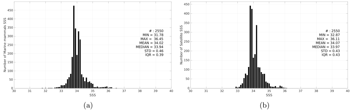
Figure 3: Histograms of SSS from Marine mammals (a) and SMOS SSS L4 v1 - Daily (CMEMS-CNR) (b) considering all match-up pairs per bins of 0.1 over the South Atlantic Ocean Pi-MEP region and for the full satellite product period.
