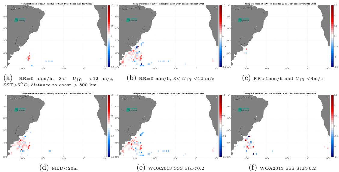
Figure 14: Temporal mean gridded over spatial boxes of size 1^\circ \times 1^\circ of \Delta SSS (SMOS SSS L4 v1 - Daily (CMEMS-CNR) - Marine mammals) for 6 different subdatasets corresponding to:RR=0 mm/h, 3 < U_{10} < 12 m/s, SST>5°C, distance to coast > 800 km (a), RR=0 mm/h, 3 < U_{10} < 12 m/s (b), RR>1mm/h and U_{10} < 4 m/s (c),MLD<20m (d),WOA2013 SSS Std<0.2 (e),WOA2013 SSS Std>0.2 (f).
