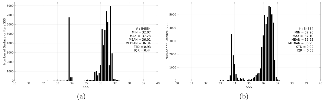
Figure 3: Histograms of SSS from Surface drifters (a) and SMOS SSS L4 v1 - Daily (CMEMS-CNR) (b) considering all match-up pairs per bins of 0.1 over the South Atlantic Ocean Pi-MEP region and for the full satellite product period.
