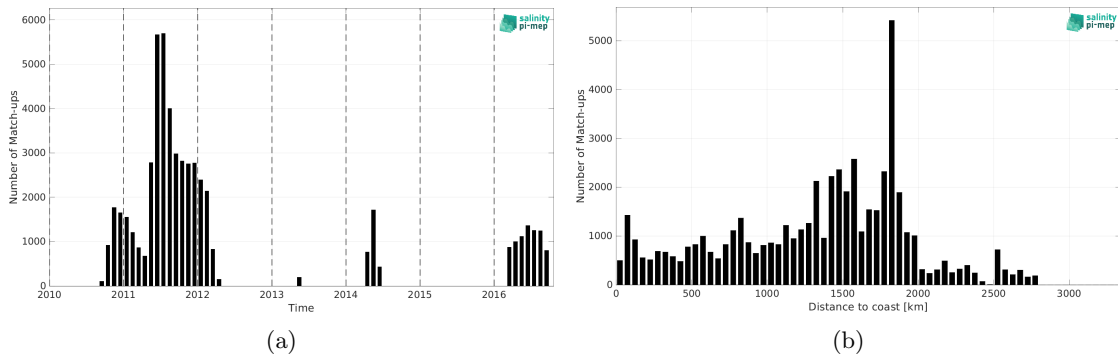
Figure 2: Number of match-ups between Surface drifters and SMOS SSS L4 v1 - Daily (CMEMS-CNR) SSS as a function of time (a) and as function of the distance to coast (b) over the South Atlantic Ocean Pi-MEP region and for the full satellite product period.
