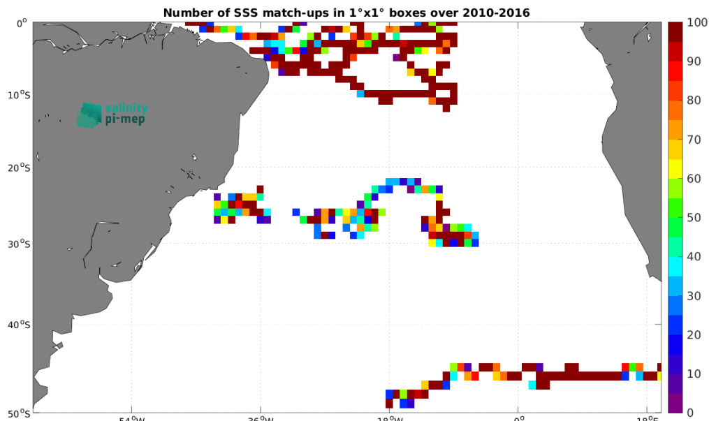
Figure 4: Number of SSS match-ups between Surface drifters SSS and the SMOS SSS L4 v1 - Daily (CMEMS-CNR) SSS product for the South Atlantic Ocean Pi-MEP region over 1^\circ \times 1^\circ boxes and for the full satellite product period.
