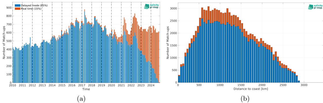
Figure 2: Number of match-ups between Argo and SMOS SSS L4 v1 - Daily (CMEMS-CNR) SSS as a function of time (a) and as function of the distance to coast (b) over the South Atlantic Ocean Pi-MEP region and for the full satellite product period.
