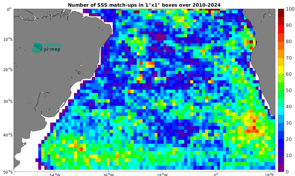
Figure 5: Number of SSS match-ups between Argo SSS and the SMOS SSS L4 v1 - Daily (CMEMS-CNR) SSS product for the South Atlantic Ocean Pi-MEP region over 1^\circ \times 1^\circ boxes and for the full satellite product period.
