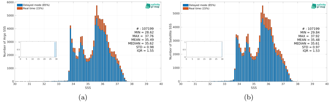
Figure 3: Histograms of SSS from Argo (a) and SMOS SSS L4 v1 - Daily (CMEMS-CNR) (b) considering all match-up pairs per bins of 0.1 over the South Atlantic Ocean Pi-MEP region and for the full satellite product period.
