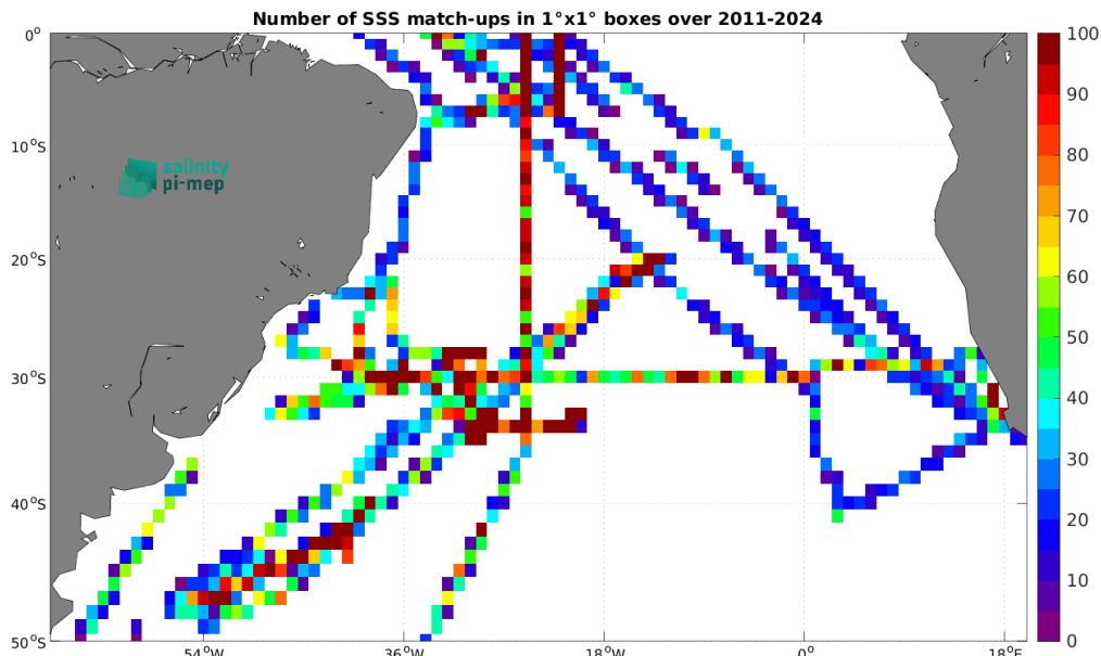
Figure 5: Number of SSS match-ups between TSG (SAMOS) SSS and the SMOS SSS L4 OI v346 - Weekly (CMEMS-CATDS-LOPS) SSS product for the South Atlantic Ocean Pi-MEP region over 1^\circ \times 1^\circ boxes and for the full satellite product period.
