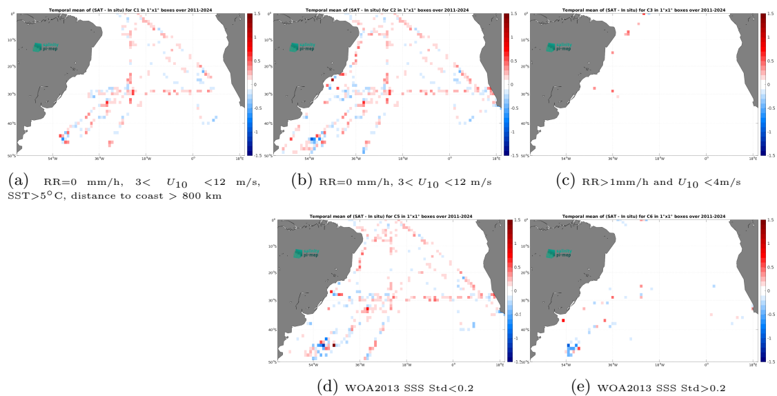
Figure 14: Temporal mean gridded over spatial boxes of size 1^\circ \times 1^\circ of \Delta\text{SSS} (SMOS SSS L4 OI v346 - Weekly (CMEMS-CATDS-LOPS) - TSG (SAMOS)) for 5 different subdatasets corresponding to:RR=0 mm/h, 3 < U_{10} < 12 m/s, SST >5^\circ\text{C} , distance to coast > 800 km (a), RR=0 mm/h, 3 < U_{10} < 12 m/s (b), RR >1 mm/h and U_{10} < 4 m/s (c), WOA2013 SSS Std <0.2 (d), WOA2013 SSS Std >0.2 (e).
