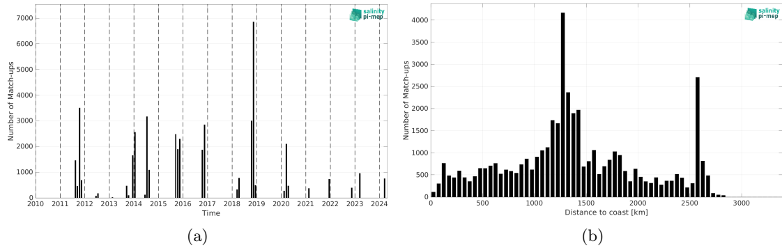
Figure 2: Number of match-ups between TSG (SAMOS) and SMOS SSS L4 OI v346 - Weekly (CMEMS-CATDS-LOPS) SSS as a function of time (a) and as function of the distance to coast (b) over the South Atlantic Ocean Pi-MEP region and for the full satellite product period.
