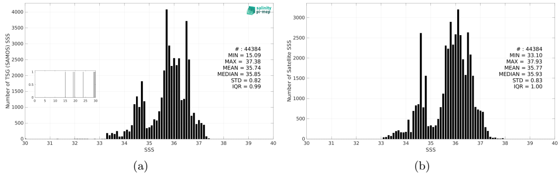
Figure 3: Histograms of SSS from TSG (SAMOS) (a) and SMOS SSS L4 OI v346 - Weekly (CMEMS-CATDS-LOPS) (b) considering all match-up pairs per bins of 0.1 over the South Atlantic Ocean Pi-MEP region and for the full satellite product period.
