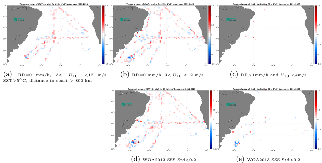
Figure 14: Temporal mean gridded over spatial boxes of size 1^\circ \times 1^\circ of \Delta\text{SSS} (SMOS SSS L4 OI v346 - Weekly (CMEMS-CATDS-LOPS) - TSG (SAMOS)) for 5 different subdatasets corresponding to:RR=0 mm/h, 3 < U_{10} < 12 m/s, SST >5^\circ\text{C} , distance to coast > 800 km (a), RR=0 mm/h, 3 < U_{10} < 12 m/s (b), RR >1 mm/h and U_{10} < 4 m/s (c), WOA2013 SSS Std <0.2 (d), WOA2013 SSS Std >0.2 (e).
