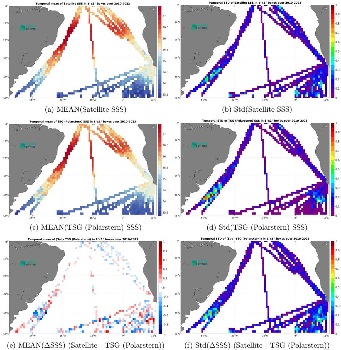
Figure 7: Temporal mean (left) and Std (right) of SSS from SMOS SSS L4 OI v346 - Weekly (CMEMS-CATDS-LOPS) (top), TSG (Polarstern) (middle), and of \Delta SSS (Satellite - TSG (Polarstern)). Only match-up pairs are used to generate these maps.
