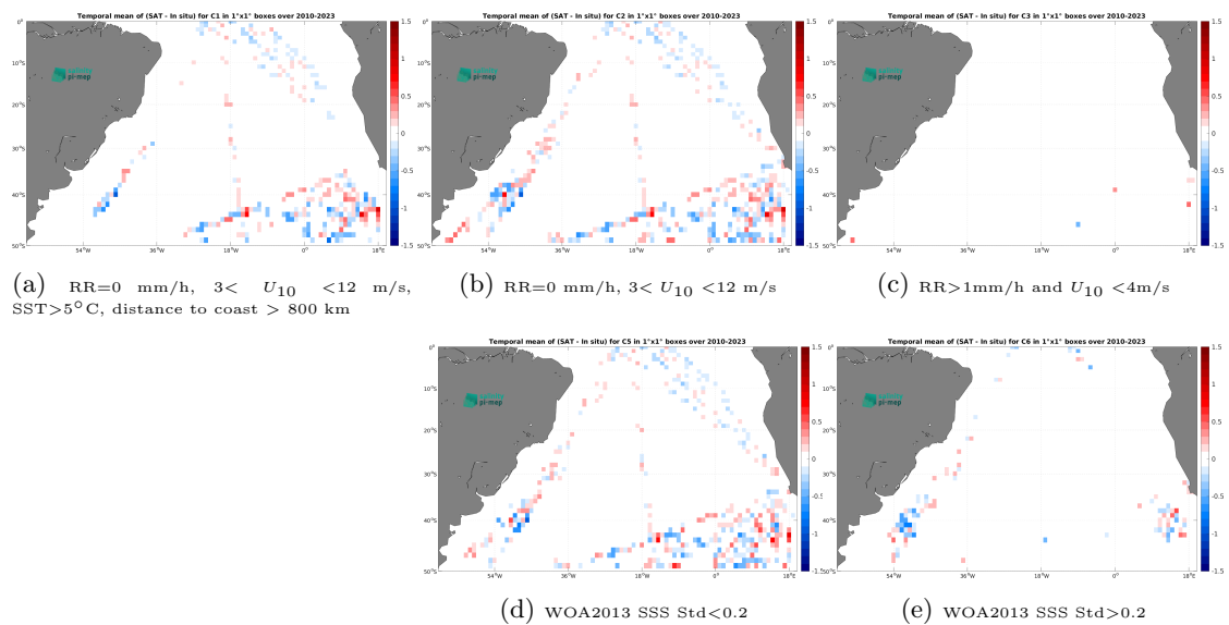
Figure 14: Temporal mean gridded over spatial boxes of size 1^\circ \times 1^\circ of \Delta SSS (SMOS SSS L4 OI v346 - Weekly (CMEMS-CATDS-LOPS) - TSG (Polarstern)) for 5 different subdatasets corresponding to:RR=0 mm/h, 3 < U_{10} < 12 m/s, SST >5^\circ\text{C} , distance to coast > 800 km (a), RR=0 mm/h, 3 < U_{10} < 12 m/s (b), RR >1 mm/h and U_{10} < 4 m/s (c), WOA2013 SSS Std <0.2 (d), WOA2013 SSS Std >0.2 (e).
