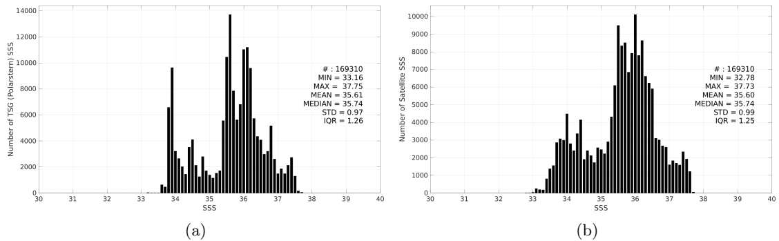
Figure 3: Histograms of SSS from TSG (Polarstern) (a) and SMOS SSS L4 OI v346 - Weekly (CMEMS-CATDS-LOPS) (b) considering all match-up pairs per bins of 0.1 over the South Atlantic Ocean Pi-MEP region and for the full satellite product period.
