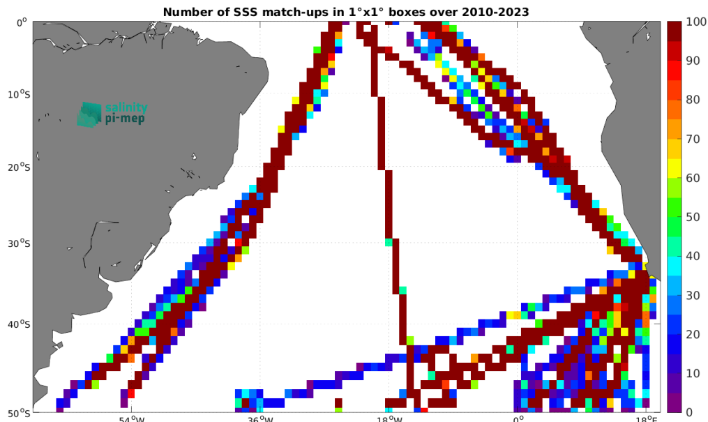
Figure 5: Number of SSS match-ups between TSG (Polarstern) SSS and the SMOS SSS L4 OI v346 - Weekly (CMEMS-CATDS-LOPS) SSS product for the South Atlantic Ocean Pi-MEP region over 1^\circ \times 1^\circ boxes and for the full satellite product period.
