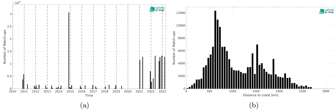
Figure 2: Number of match-ups between TSG (Polarstern) and SMOS SSS L4 OI v346 - Weekly (CMEMS-CATDS-LOPS) SSS as a function of time (a) and as function of the distance to coast (b) over the South Atlantic Ocean Pi-MEP region and for the full satellite product period.
