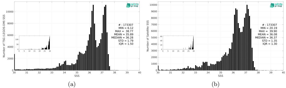
Figure 3: Histograms of SSS from TSG (LEGOS-DM) (a) and SMOS SSS L4 OI v346 - Weekly (CMEMS-CATDS-LOPS) (b) considering all match-up pairs per bins of 0.1 over the South Atlantic Ocean Pi-MEP region and for the full satellite product period.
