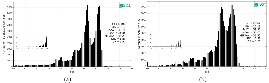
Figure 3: Histograms of SSS from TSG (LEGOS-DM) (a) and SMOS SSS L4 OI v346 - Weekly (CMEMS-CATDS-LOPS) (b) considering all match-up pairs per bins of 0.1 over the South Atlantic Ocean Pi-MEP region and for the full satellite product period.
