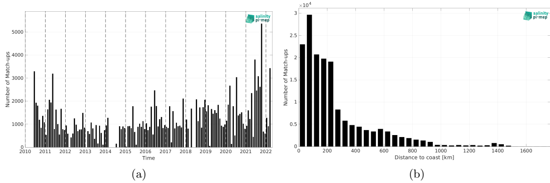
Figure 2: Number of match-ups between TSG (LEGOS-DM) and SMOS SSS L4 OI v346 - Weekly (CMEMS-CATDS-LOPS) SSS as a function of time (a) and as function of the distance to coast (b) over the South Atlantic Ocean Pi-MEP region and for the full satellite product period.
