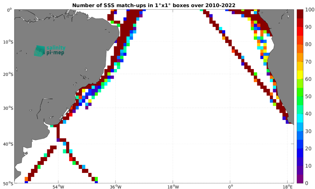
Figure 5: Number of SSS match-ups between TSG (LEGOS-DM) SSS and the SMOS SSS L4 OI v346 - Weekly (CMEMS-CATDS-LOPS) SSS product for the South Atlantic Ocean Pi-MEP region over 1^\circ \times 1^\circ boxes and for the full satellite product period.
