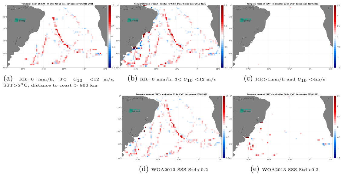
Figure 14: Temporal mean gridded over spatial boxes of size 1^\circ \times 1^\circ of \Delta\text{SSS} (SMOS SSS L4 OI v346 - Weekly (CMEMS-CATDS-LOPS) - TSG (GOSUD-Sailing-ship)) for 5 different sub-datasets corresponding to:RR=0 mm/h, 3 < U_{10} < 12 m/s, SST >5^\circ\text{C} , distance to coast > 800 km (a), RR=0 mm/h, 3 < U_{10} < 12 m/s (b), RR >1 mm/h and U_{10} < 4 m/s (c), WOA2013 SSS Std <0.2 (d), WOA2013 SSS Std >0.2 (e).
