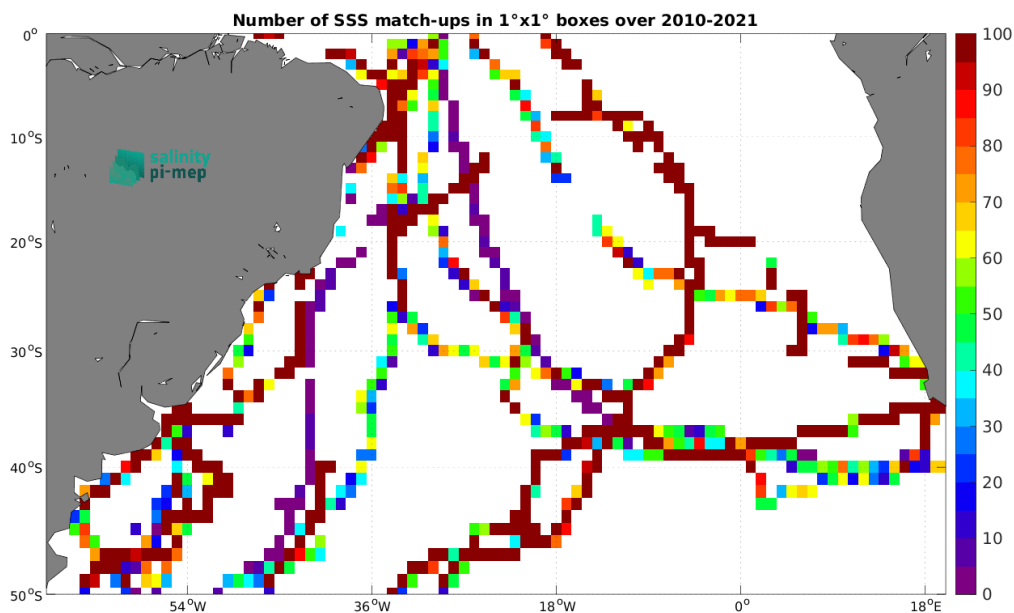
Figure 5: Number of SSS match-ups between TSG (GOSUD-Sailing-ship) SSS and the SMOS SSS L4 OI v346 - Weekly (CMEMS-CATDS-LOPS) SSS product for the South Atlantic Ocean Pi-MEP region over 1^\circ \times 1^\circ boxes and for the full satellite product period.
