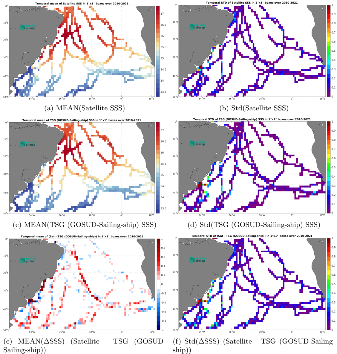
Figure 7: Temporal mean (left) and Std (right) of SSS from SMOS SSS L4 OI v346 - Weekly (CMEMS-CATDS-LOPS) (top), TSG (GOSUD-Sailing-ship) (middle), and of \Delta SSS (Satellite - TSG (GOSUD-Sailing-ship)). Only match-up pairs are used to generate these maps.
