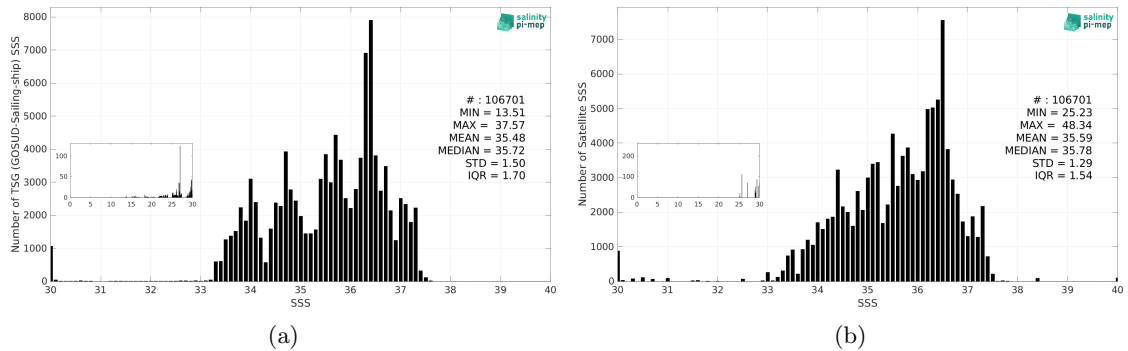
Figure 3: Histograms of SSS from TSG (GOSUD-Sailing-ship) (a) and SMOS SSS L4 OI v346 - Weekly (CMEMS-CATDS-LOPS) (b) considering all match-up pairs per bins of 0.1 over the South Atlantic Ocean Pi-MEP region and for the full satellite product period.
