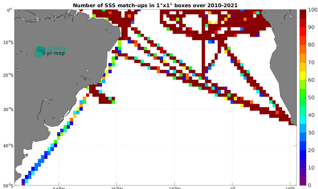
Figure 5: Number of SSS match-ups between TSG (GOSUD-Research-vessel) SSS and the SMOS SSS L4 OI v346 - Weekly (CMEMS-CATDS-LOPS) SSS product for the South Atlantic Ocean Pi-MEP region over 1^\circ \times 1^\circ boxes and for the full satellite product period.
