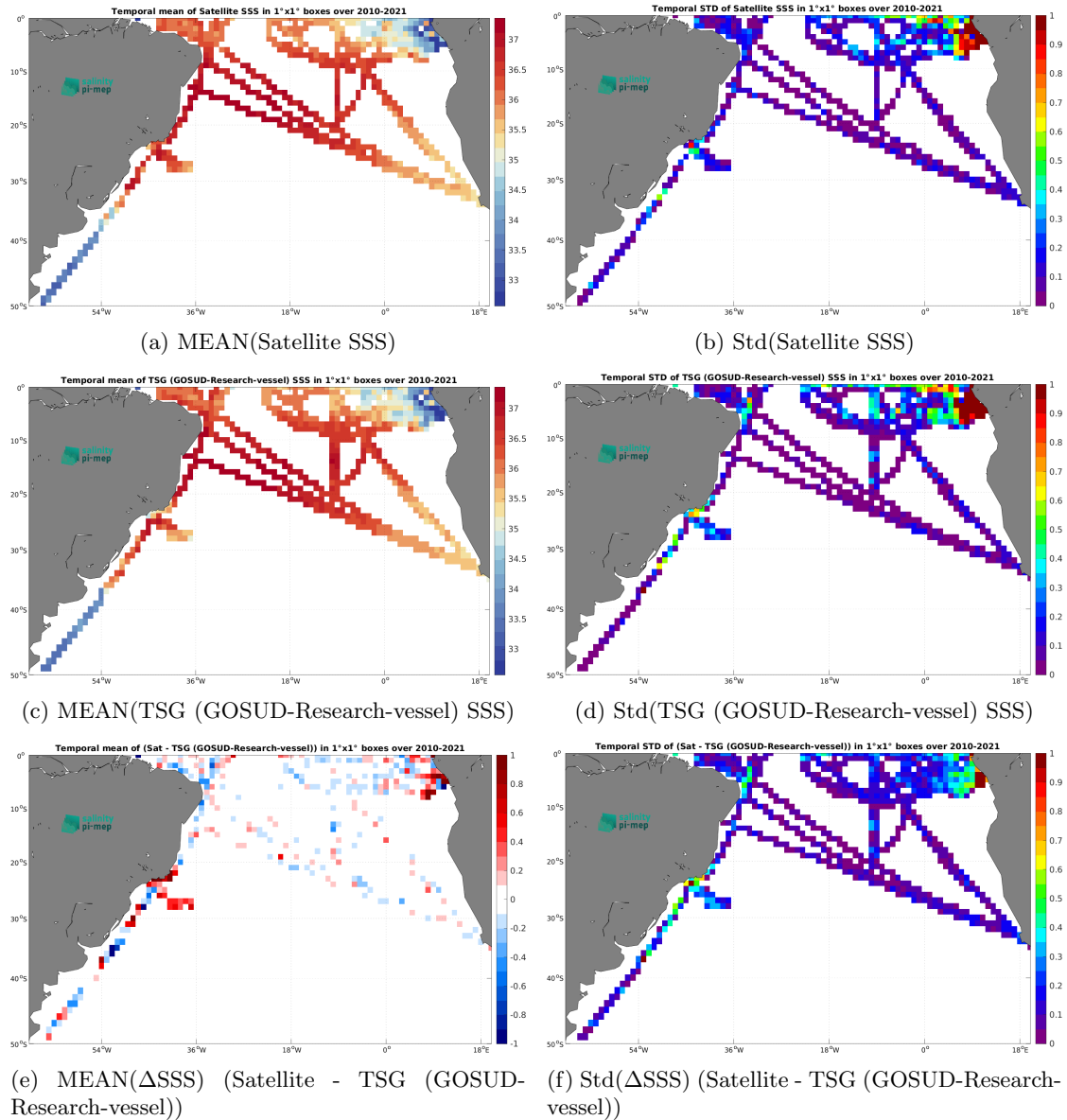
Figure 7: Temporal mean (left) and Std (right) of SSS from SMOS SSS L4 OI v346 - Weekly (CMEMS-CATDS-LOPS) (top), TSG (GOSUD-Research-vessel) (middle), and of \Delta SSS (Satellite - TSG (GOSUD-Research-vessel)). Only match-up pairs are used to generate these maps.
