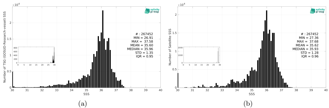
Figure 3: Histograms of SSS from TSG (GOSUD-Research-vessel) (a) and SMOS SSS L4 OI v346 - Weekly (CMEMS-CATDS-LOPS) (b) considering all match-up pairs per bins of 0.1 over the South Atlantic Ocean Pi-MEP region and for the full satellite product period.
