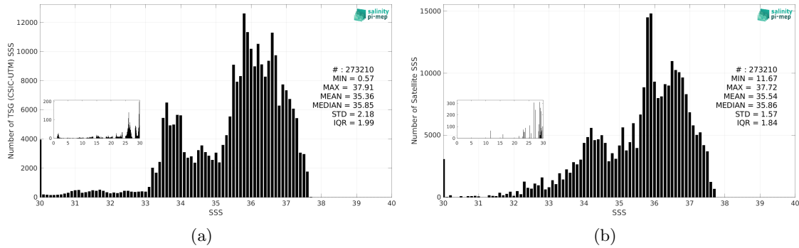
Figure 3: Histograms of SSS from TSG (CSIC-UTM) (a) and SMOS SSS L4 OI v346 - Weekly (CMEMS-CATDS-LOPS) (b) considering all match-up pairs per bins of 0.1 over the South Atlantic Ocean Pi-MEP region and for the full satellite product period.
