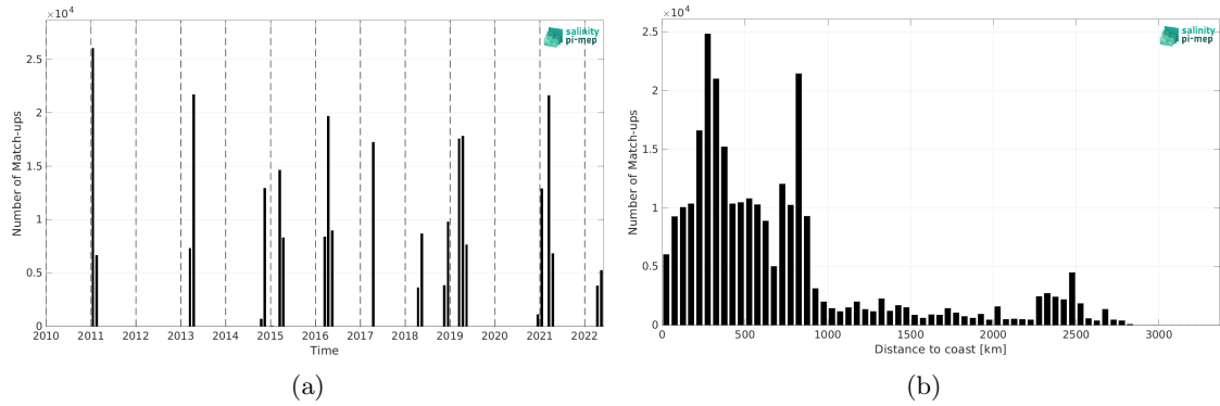
Figure 2: Number of match-ups between TSG (CSIC-UTM) and SMOS SSS L4 OI v346 - Weekly (CMEMS-CATDS-LOPS) SSS as a function of time (a) and as function of the distance to coast (b) over the South Atlantic Ocean Pi-MEP region and for the full satellite product period.
