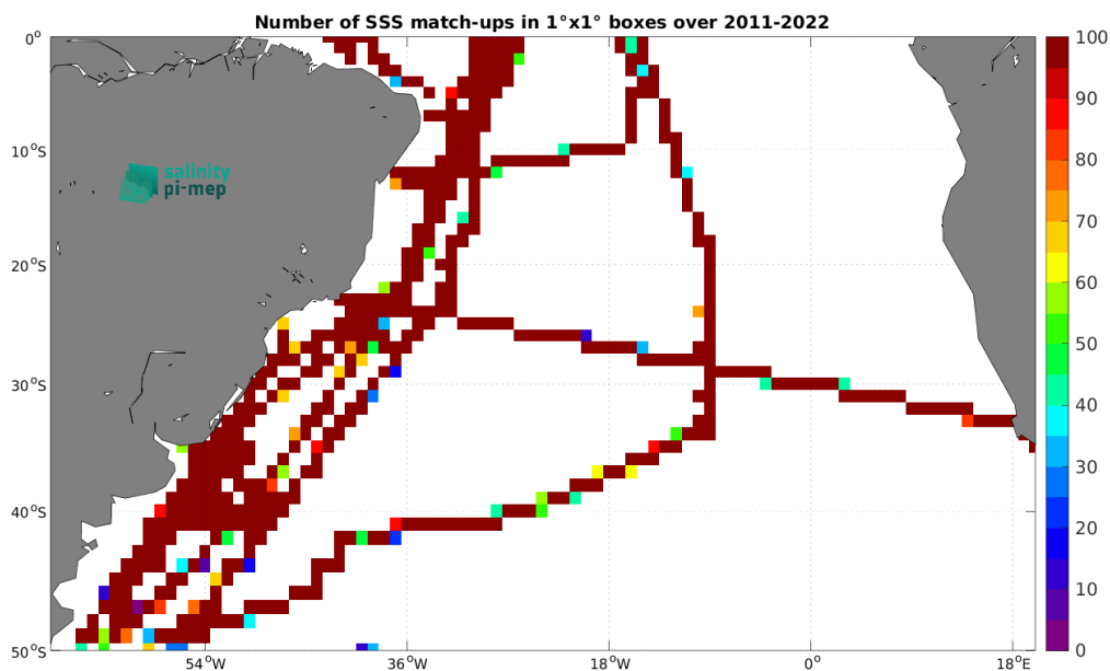
Figure 5: Number of SSS match-ups between TSG (CSIC-UTM) SSS and the SMOS SSS L4 OI v346 - Weekly (CMEMS-CATDS-LOPS) SSS product for the South Atlantic Ocean Pi-MEP region over 1^\circ \times 1^\circ boxes and for the full satellite product period.
