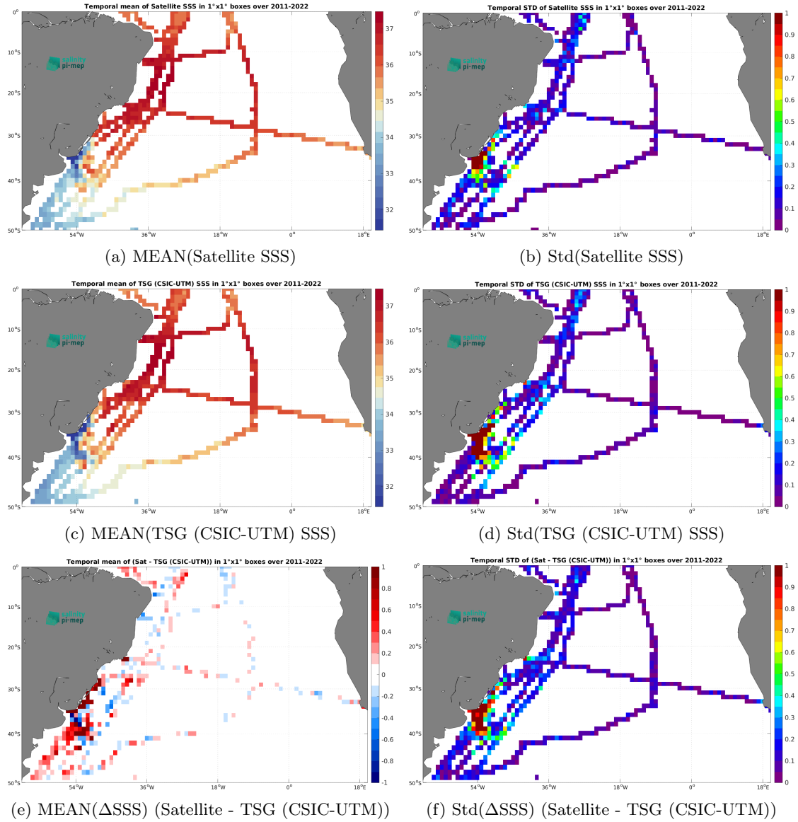
Figure 7: Temporal mean (left) and Std (right) of SSS from SMOS SSS L4 OI v346 - Weekly (CMEMS-CATDS-LOPS) (top), TSG (CSIC-UTM) (middle), and of \Delta SSS (Satellite - TSG (CSIC-UTM)). Only match-up pairs are used to generate these maps.
