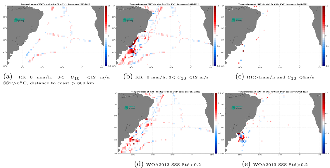
Figure 14: Temporal mean gridded over spatial boxes of size 1^\circ \times 1^\circ of \Delta SSS (SMOS SSS L4 OI v346 - Weekly (CMEMS-CATDS-LOPS) - TSG (CSIC-UTM)) for 5 different subdatasets corresponding to:RR=0 mm/h, 3 < U_{10} < 12 m/s, SST >5^\circ\text{C} , distance to coast > 800 km (a), RR=0 mm/h, 3 < U_{10} < 12 m/s (b), RR >1 mm/h and U_{10} < 4 m/s (c), WOA2013 SSS Std <0.2 (d), WOA2013 SSS Std >0.2 (e).
