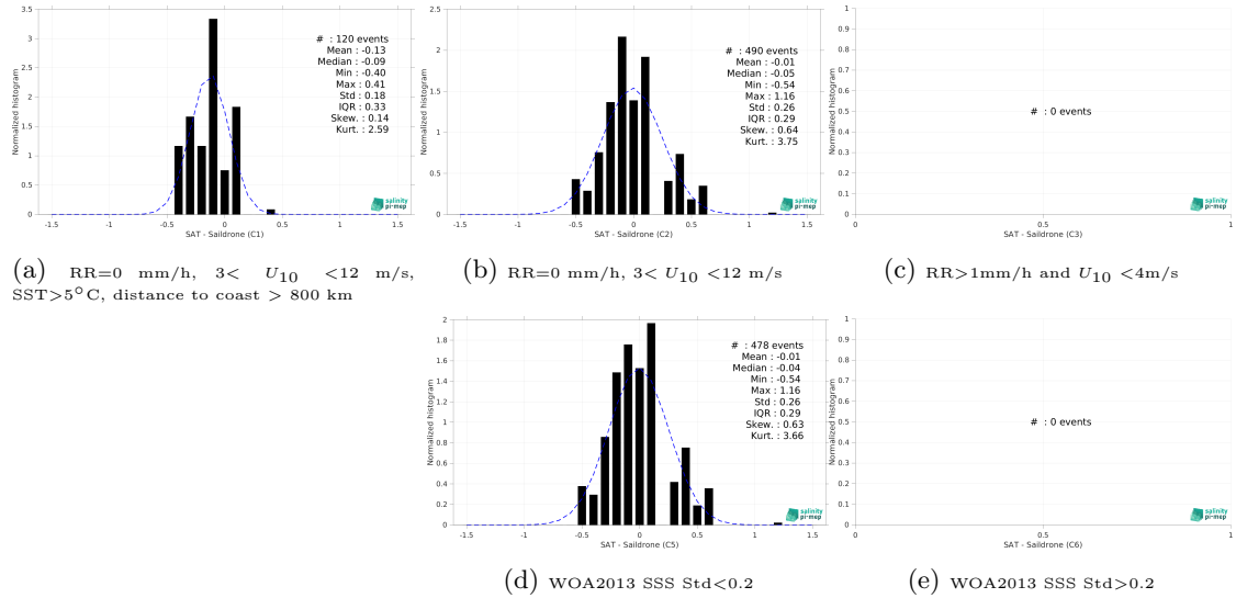
Figure 15: Normalized histogram of \Delta SSS (SMOS SSS L4 OI v346 - Weekly (CMEMS-CATDS-LOPS) - Saldrone) for 5 different subdatasets corresponding to: RR=0 mm/h, 3 < U_{10} < 12 m/s, SST > 5°C, distance to coast > 800 km (a), RR=0 mm/h, 3 < U_{10} < 12 m/s (b), RR > 1mm/h and U_{10} < 4 m/s (c), WOA2013 SSS Std < 0.2 (d), WOA2013 SSS Std > 0.2 (e).
