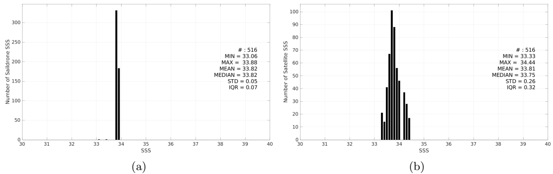
Figure 3: Histograms of SSS from Saildrone (a) and SMOS SSS L4 OI v346 - Weekly (CMEMS-CATDS-LOPS) (b) considering all match-up pairs per bins of 0.1 over the South Atlantic Ocean Pi-MEP region and for the full satellite product period.
