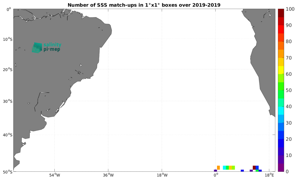
Figure 5: Number of SSS match-ups between Saildrone SSS and the SMOS SSS L4 OI v346 - Weekly (CMEMS-CATDS-LOPS) SSS product for the South Atlantic Ocean Pi-MEP region over 1^\circ \times 1^\circ boxes and for the full satellite product period.
