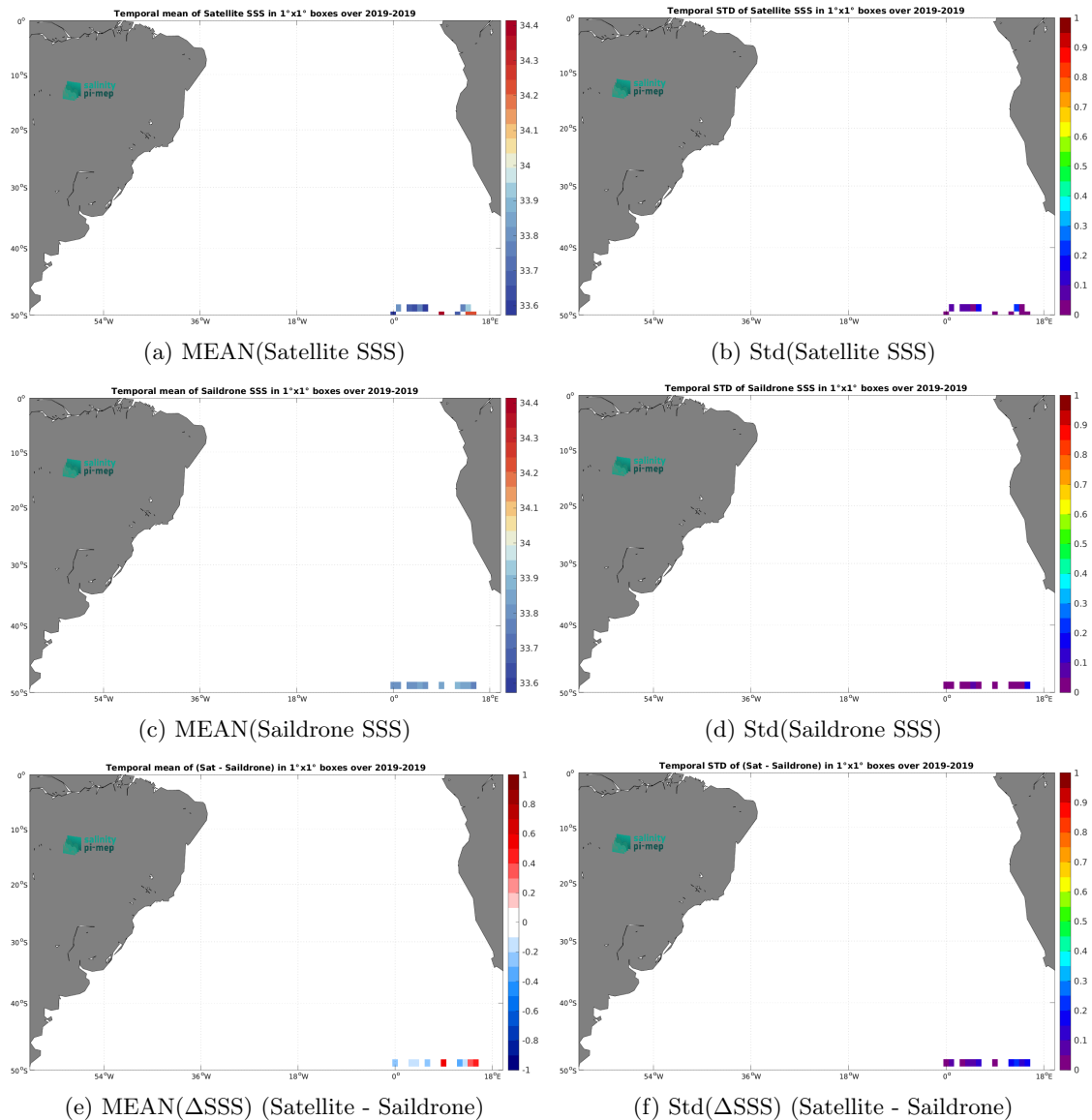
Figure 7: Temporal mean (left) and Std (right) of SSS from SMOS SSS L4 OI v346 - Weekly (CMEMS-CATDS-LOPS) (top), Saildrone (middle), and of \Delta SSS (Satellite - Saildrone). Only match-up pairs are used to generate these maps.
