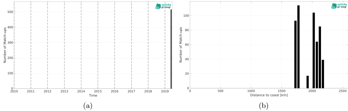
Figure 2: Number of match-ups between Saildrone and SMOS SSS L4 OI v346 - Weekly (CMEMS-CATDS-LOPS) SSS as a function of time (a) and as function of the distance to coast (b) over the South Atlantic Ocean Pi-MEP region and for the full satellite product period.
