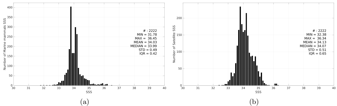
Figure 3: Histograms of SSS from Marine mammals (a) and SMOS SSS L4 OI v346 - Weekly (CMEMS-CATDS-LOPS) (b) considering all match-up pairs per bins of 0.1 over the South Atlantic Ocean Pi-MEP region and for the full satellite product period.
