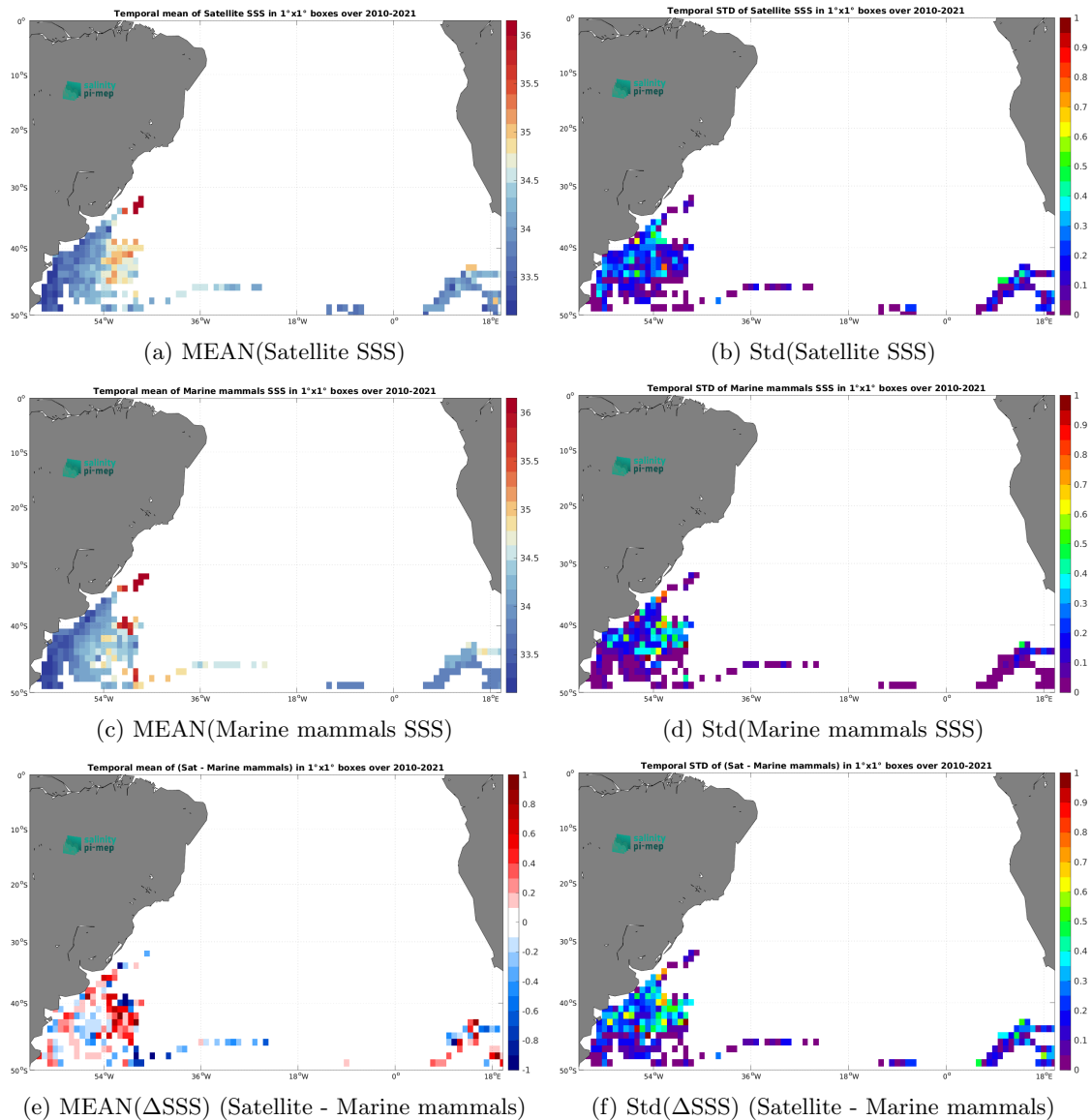
Figure 7: Temporal mean (left) and Std (right) of SSS from SMOS SSS L4 OI v346 - Weekly (CMEMS-CATDS-LOPS) (top), Marine mammals (middle), and of \Delta SSS (Satellite - Marine mammals). Only match-up pairs are used to generate these maps.
