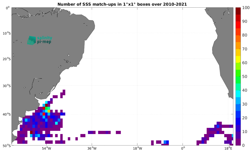
Figure 5: Number of SSS match-ups between Marine mammals SSS and the SMOS SSS L4 OI v346 - Weekly (CMEMS-CATDS-LOPS) SSS product for the South Atlantic Ocean Pi-MEP region over 1^{\circ} \times 1^{\circ} boxes and for the full satellite product period.
