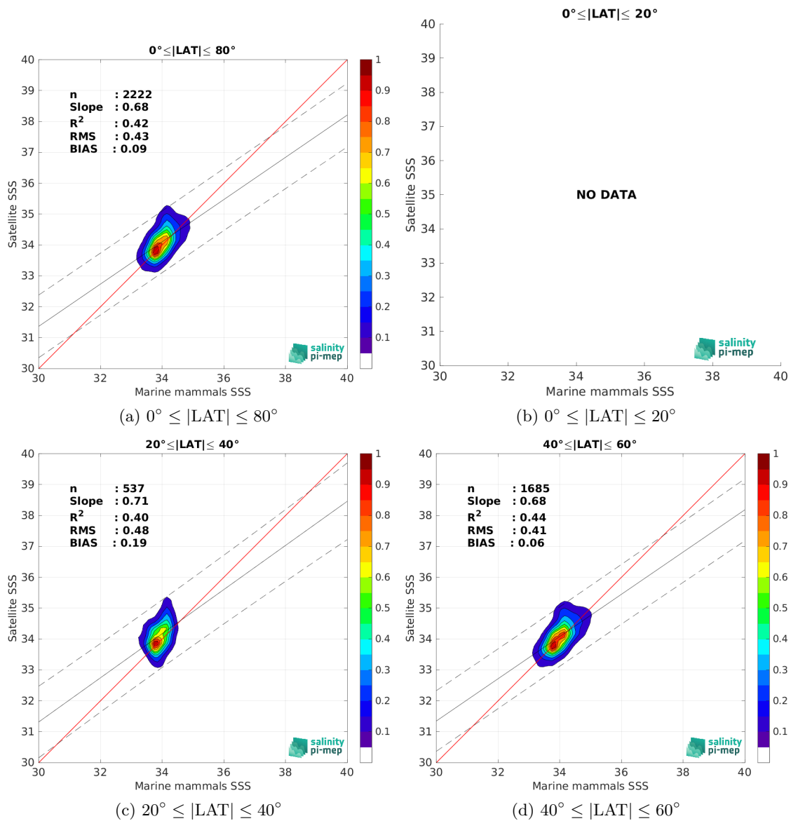
Figure 10: Contour maps of the concentration of SMOS SSS L4 OI v346 - Weekly (CMEMS-CATDS-LOPS) SSS (y-axis) versus Marine mammals SSS (x-axis) at match-up pairs for different latitude bands. For each plot, the red line shows x=y . The black thin and dashed lines indicate a linear fit through the data cloud and the \pm 95\% confidence levels, respectively. The number match-up pairs n , the slope and R^2 coefficient of the linear fit, the root mean square (RMS) and the mean bias between satellite and in situ data are indicated for each latitude band in each plots.
