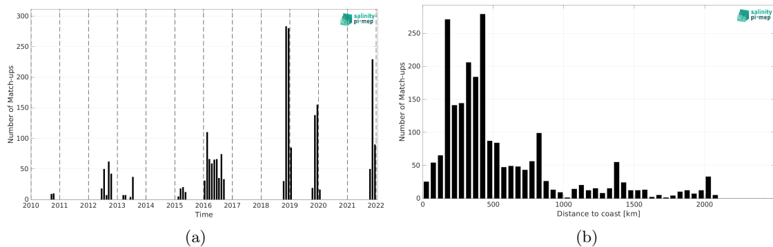
Figure 2: Number of match-ups between Marine mammals and SMOS SSS L4 OI v346 - Weekly (CMEMS-CATDS-LOPS) SSS as a function of time (a) and as function of the distance to coast (b) over the South Atlantic Ocean Pi-MEP region and for the full satellite product period.
