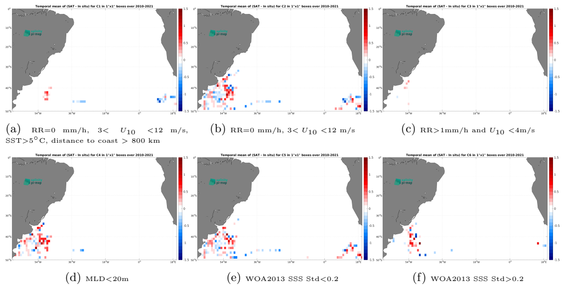
Figure 14: Temporal mean gridded over spatial boxes of size 1^\circ \times 1^\circ of \Delta SSS (SMOS SSS L4 OI v346 - Weekly (CMEMS-CATDS-LOPS) - Marine mammals) for 6 different subdatasets corresponding to:RR=0 mm/h, 3 < U_{10} < 12 m/s, SST >5^\circ\text{C} , distance to coast > 800 km (a), RR=0 mm/h, 3 < U_{10} < 12 m/s (b), RR >1 mm/h and U_{10} < 4 m/s (c),MLD <20 m (d),WOA2013 SSS Std <0.2 (e),WOA2013 SSS Std >0.2 (f).
