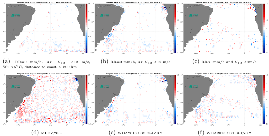
Figure 14: Temporal mean gridded over spatial boxes of size 1^\circ \times 1^\circ of \Delta SSS (SMOS SSS L4 OI v346 - Weekly (CMEMS-CATDS-LOPS) - Argo) for 6 different subdatasets corresponding to:RR=0 mm/h, 3 < U_{10} < 12 m/s, SST>5°C, distance to coast > 800 km (a), RR=0 mm/h, 3 < U_{10} < 12 m/s (b), RR>1mm/h and U_{10} < 4 m/s (c),MLD<20m (d),WOA2013 SSS Std<0.2 (e),WOA2013 SSS Std>0.2 (f).
