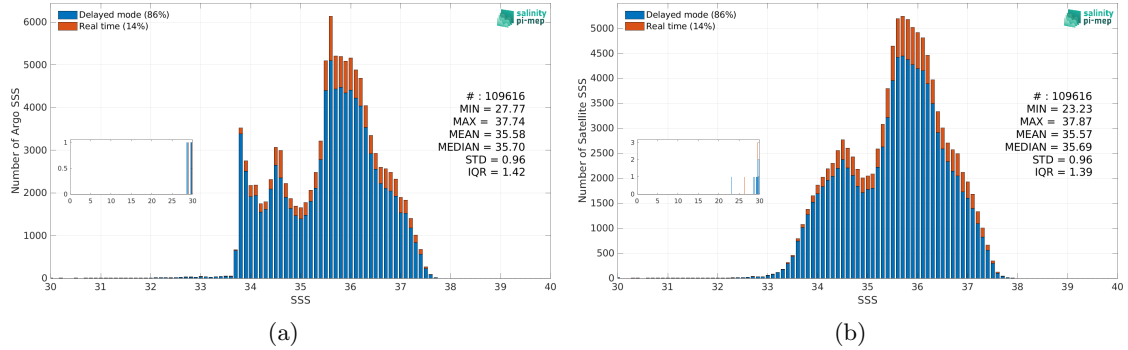
Figure 3: Histograms of SSS from Argo (a) and SMOS SSS L4 OI v346 - Weekly (CMEMS-CATDS-LOPS) (b) considering all match-up pairs per bins of 0.1 over the South Atlantic Ocean Pi-MEP region and for the full satellite product period.
