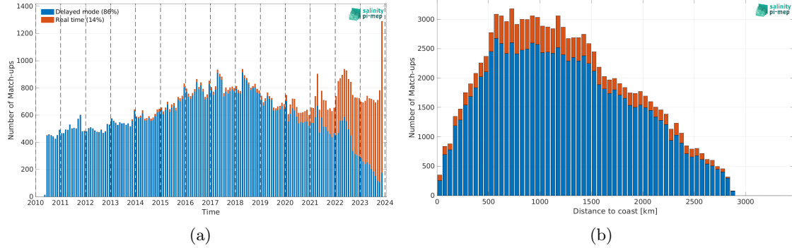
Figure 2: Number of match-ups between Argo and SMOS SSS L4 OI v346 - Weekly (CMEMS-CATDS-LOPS) SSS as a function of time (a) and as function of the distance to coast (b) over the South Atlantic Ocean Pi-MEP region and for the full satellite product period.
