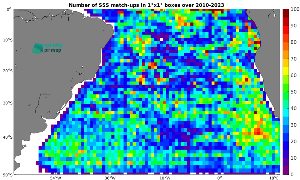
Figure 5: Number of SSS match-ups between Argo SSS and the SMOS SSS L4 OI v346 - Weekly (CMEMS-CATDS-LOPS) SSS product for the South Atlantic Ocean Pi-MEP region over 1^\circ \times 1^\circ boxes and for the full satellite product period.
