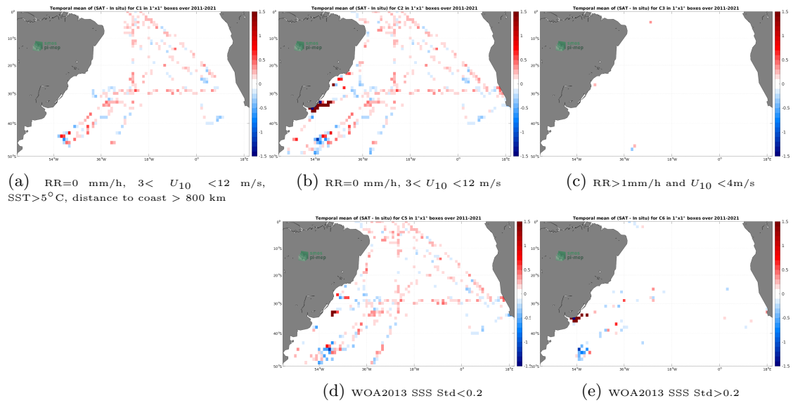
Figure 12: Temporal mean gridded over spatial boxes of size 1^\circ \times 1^\circ of \Delta\text{SSS} (SMOS SSS L4 OI v342 - Weekly (CMEMS-CATDS-LOPS) - TSG (SAMOS)) for 5 different subdatasets corresponding to:RR=0 mm/h, 3 < U_{10} < 12 m/s, SST >5^\circ\text{C} , distance to coast > 800 km (a), RR=0 mm/h, 3 < U_{10} < 12 m/s (b), RR >1 mm/h and U_{10} < 4 m/s (c), WOA2013 SSS Std <0.2 (d), WOA2013 SSS Std >0.2 (e).
