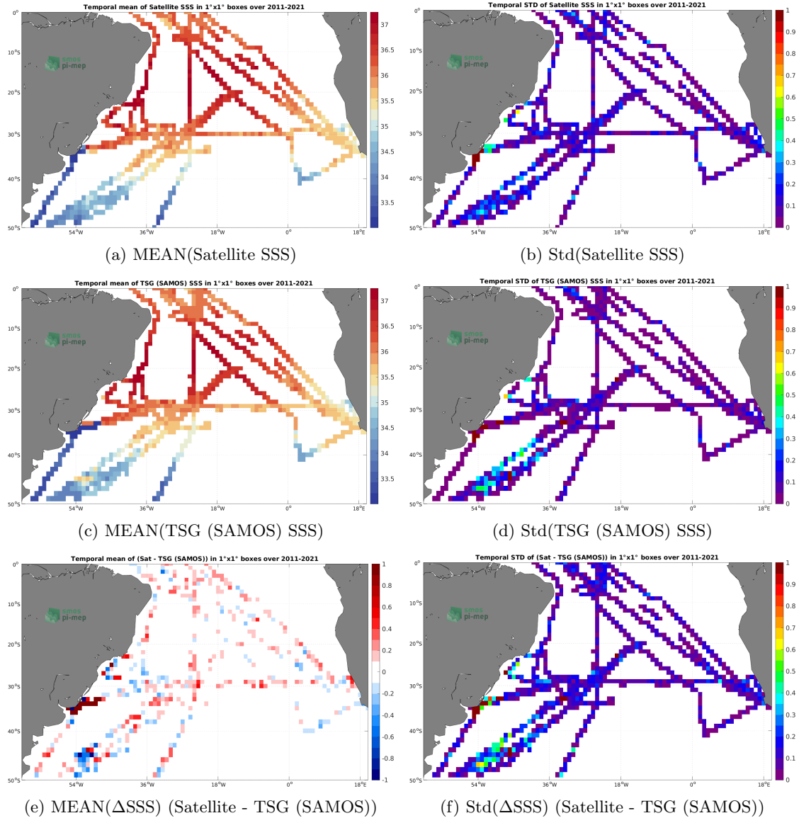
Figure 6: Temporal mean (left) and Std (right) of SSS from SMOS SSS L4 OI v342 - Weekly (CMEMS-CATDS-LOPS) (top), TSG (SAMOS) (middle), and of \Delta SSS (Satellite - TSG (SAMOS)). Only match-up pairs are used to generate these maps.
