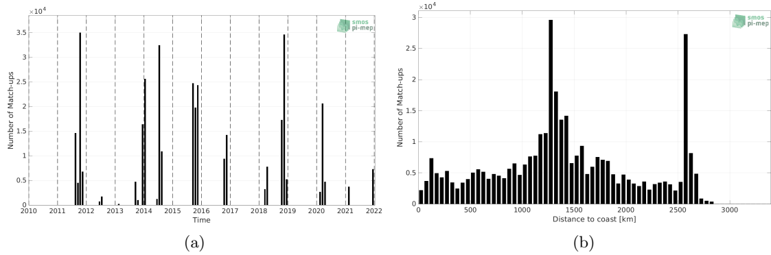
Figure 1: Number of match-ups between TSG (SAMOS) and SMOS SSS L4 OI v342 - Weekly (CMEMS-CATDS-LOPS) SSS as a function of time (a) and as function of the distance to coast (b) over the South Atlantic Ocean Pi-MEP region and for the full satellite product period.
