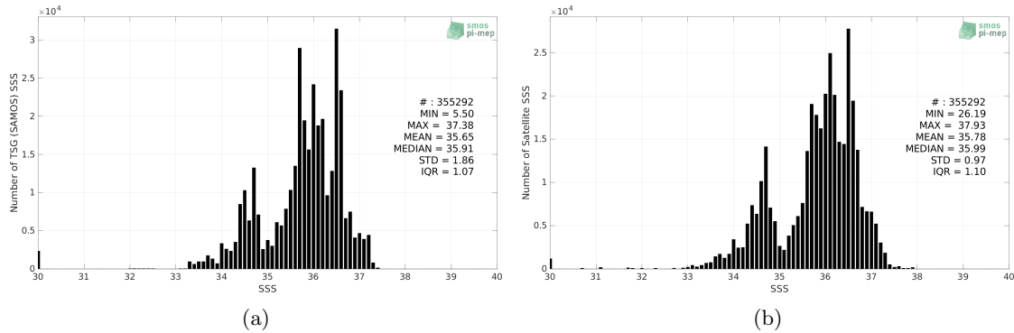
Figure 2: Histograms of SSS from TSG (SAMOS) (a) and SMOS SSS L4 OI v342 - Weekly (CMEMS-CATDS-LOPS) (b) considering all match-up pairs per bins of 0.1 over the South Atlantic Ocean Pi-MEP region and for the full satellite product period.
