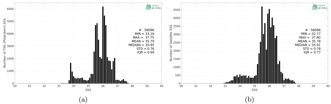
Figure 2: Histograms of SSS from TSG (Polarstern) (a) and SMOS SSS L4 OI v342 - Weekly (CMEMS-CATDS-LOPS) (b) considering all match-up pairs per bins of 0.1 over the South Atlantic Ocean Pi-MEP region and for the full satellite product period.
