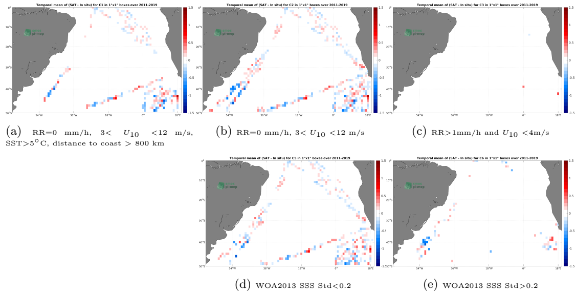
Figure 12: Temporal mean gridded over spatial boxes of size 1^\circ \times 1^\circ of \Delta\text{SSS} (SMOS SSS L4 OI v342 - Weekly (CMEMS-CATDS-LOPS) - TSG (Polarstern)) for 5 different subdatasets corresponding to:RR=0 mm/h, 3 < U_{10} < 12 m/s, SST >5^\circ\text{C} , distance to coast > 800 km (a), RR=0 mm/h, 3 < U_{10} < 12 m/s (b), RR >1 mm/h and U_{10} < 4 m/s (c), WOA2013 SSS Std <0.2 (d), WOA2013 SSS Std >0.2 (e).
