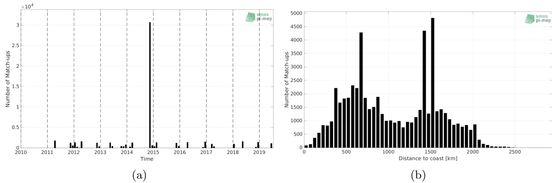
Figure 1: Number of match-ups between TSG (Polarstern) and SMOS SSS L4 OI v342 - Weekly (CMEMS-CATDS-LOPS) SSS as a function of time (a) and as function of the distance to coast (b) over the South Atlantic Ocean Pi-MEP region and for the full satellite product period.
