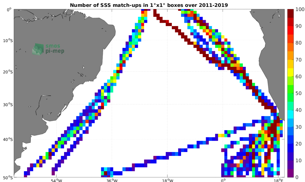
Figure 4: Number of SSS match-ups between TSG (Polarstern) SSS and the SMOS SSS L4 OI v342 - Weekly (CMEMS-CATDS-LOPS) SSS product for the South Atlantic Ocean Pi-MEP region over 1^\circ \times 1^\circ boxes and for the full satellite product period.
