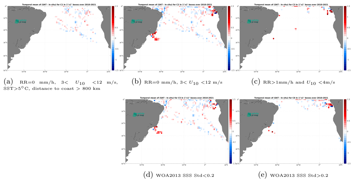
Figure 12: Temporal mean gridded over spatial boxes of size 1^\circ \times 1^\circ of \Delta SSS (SMOS SSS L4 OI v342 - Weekly (CMEMS-CATDS-LOPS) - TSG (GOSUD-Research-vessel)) for 5 different subdatasets corresponding to:RR=0 mm/h, 3 < U_{10} < 12 m/s, SST>5°C, distance to coast > 800 km (a), RR=0 mm/h, 3 < U_{10} < 12 m/s (b), RR>1mm/h and U_{10} < 4 m/s (c), WOA2013 SSS Std<0.2 (d), WOA2013 SSS Std>0.2 (e).
