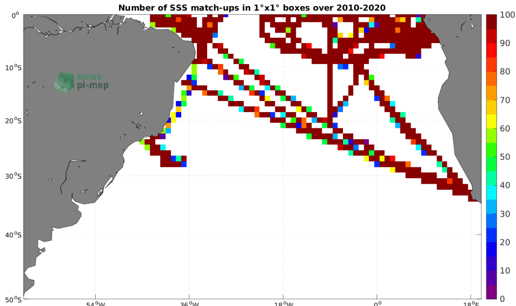
Figure 4: Number of SSS match-ups between TSG (GOSUD-Research-vessel) SSS and the SMOS SSS L4 OI v342 - Weekly (CMEMS-CATDS-LOPS) SSS product for the South Atlantic Ocean Pi-MEP region over 1^\circ \times 1^\circ boxes and for the full satellite product period.
