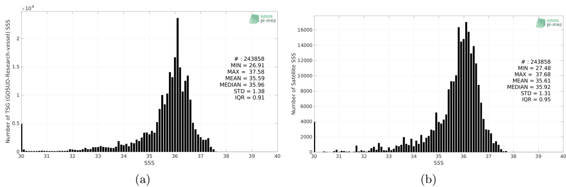
Figure 2: Histograms of SSS from TSG (GOSUD-Research-vessel) (a) and SMOS SSS L4 OI v342 - Weekly (CMEMS-CATDS-LOPS) (b) considering all match-up pairs per bins of 0.1 over the South Atlantic Ocean Pi-MEP region and for the full satellite product period.
