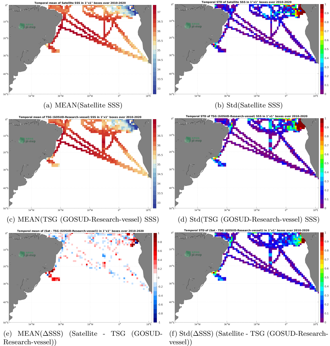
Figure 6: Temporal mean (left) and Std (right) of SSS from SMOS SSS L4 OI v342 - Weekly (CMEMS-CATDS-LOPS) (top), TSG (GOSUD-Research-vessel) (middle), and of \Delta SSS (Satellite - TSG (GOSUD-Research-vessel)). Only match-up pairs are used to generate these maps.
