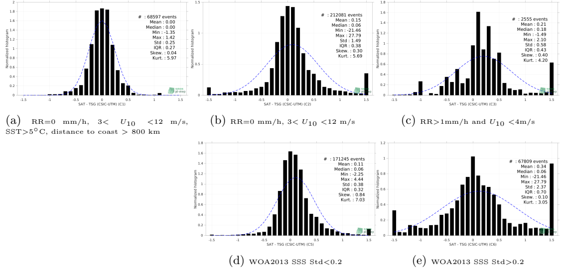
Figure 13: Normalized histogram of \Delta SSS (SMOS SSS L4 OI v342 - Weekly (CMEMS-CATDS-LOPS) - TSG (CSIC-UTM)) for 5 different subdatasets corresponding to: RR=0 mm/h, 3 < U_{10} < 12 m/s, SST > 5°C, distance to coast > 800 km (a), RR=0 mm/h, 3 < U_{10} < 12 m/s (b), RR > 1mm/h and U_{10} < 4 m/s (c), WOA2013 SSS Std < 0.2 (d), WOA2013 SSS Std > 0.2 (e).
