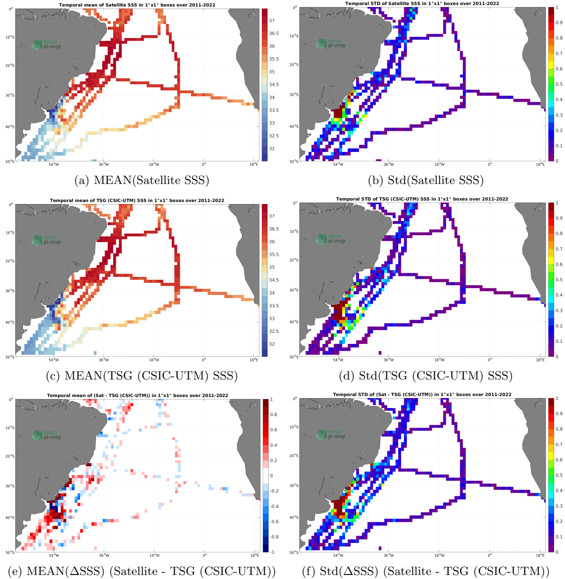
Figure 6: Temporal mean (left) and Std (right) of SSS from SMOS SSS L4 OI v342 - Weekly (CMEMS-CATDS-LOPS) (top), TSG (CSIC-UTM) (middle), and of \Delta SSS (Satellite - TSG (CSIC-UTM)). Only match-up pairs are used to generate these maps.
