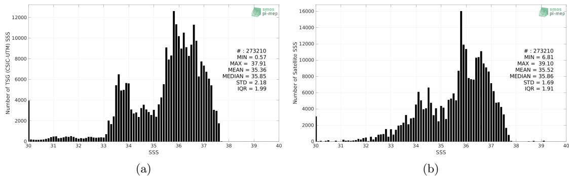
Figure 2: Histograms of SSS from TSG (CSIC-UTM) (a) and SMOS SSS L4 OI v342 - Weekly (CMEMS-CATDS-LOPS) (b) considering all match-up pairs per bins of 0.1 over the South Atlantic Ocean Pi-MEP region and for the full satellite product period.
