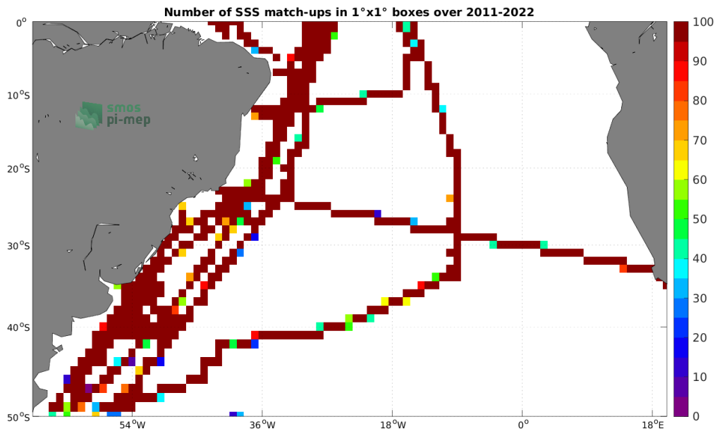
Figure 4: Number of SSS match-ups between TSG (CSIC-UTM) SSS and the SMOS SSS L4 OI v342 - Weekly (CMEMS-CATDS-LOPS) SSS product for the South Atlantic Ocean Pi-MEP region over 1^\circ \times 1^\circ boxes and for the full satellite product period.
