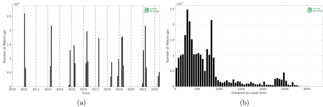
Figure 1: Number of match-ups between TSG (CSIC-UTM) and SMOS SSS L4 OI v342 - Weekly (CMEMS-CATDS-LOPS) SSS as a function of time (a) and as function of the distance to coast (b) over the South Atlantic Ocean Pi-MEP region and for the full satellite product period.
