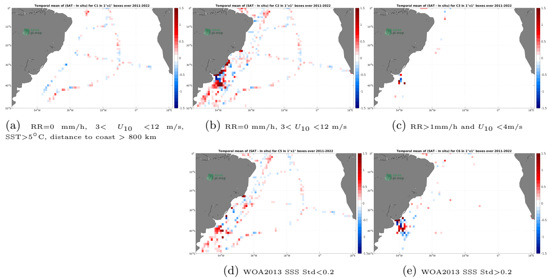
Figure 12: Temporal mean gridded over spatial boxes of size 1^\circ \times 1^\circ of \Delta\text{SSS} (SMOS SSS L4 OI v342 - Weekly (CMEMS-CATDS-LOPS) - TSG (CSIC-UTM)) for 5 different subdatasets corresponding to:RR=0 mm/h, 3 < U_{10} < 12 m/s, SST >5^\circ\text{C} , distance to coast > 800 km (a), RR=0 mm/h, 3 < U_{10} < 12 m/s (b), RR >1 mm/h and U_{10} < 4 m/s (c), WOA2013 SSS Std <0.2 (d), WOA2013 SSS Std >0.2 (e).
