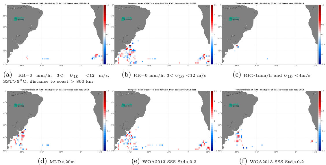
Figure 12: Temporal mean gridded over spatial boxes of size 1^{\circ}\times 1^{\circ} of \Delta\text{SSS} (SMOS SSS L4 OI v342 - Weekly (CMEMS-CATDS-LOPS) - Marine mammals) for 6 different subdatasets corresponding to:RR=0 mm/h, 3 < U_{10} < 12 m/s, SST > 5^{\circ}\text{C} , distance to coast > 800 km (a), RR=0 mm/h, 3 < U_{10} < 12 m/s (b), RR > 1\text{mm/h} and U_{10} < 4\text{m/s} (c),MLD < 20\text{m} (d),WOA2013 SSS Std < 0.2 (e),WOA2013 SSS Std > 0.2 (f).
