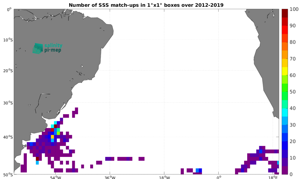
Figure 4: Number of SSS match-ups between Marine mammals SSS and the SMOS SSS L4 OI v342 - Weekly (CMEMS-CATDS-LOPS) SSS product for the South Atlantic Ocean Pi-MEP region over 1^\circ \times 1^\circ boxes and for the full satellite product period.
