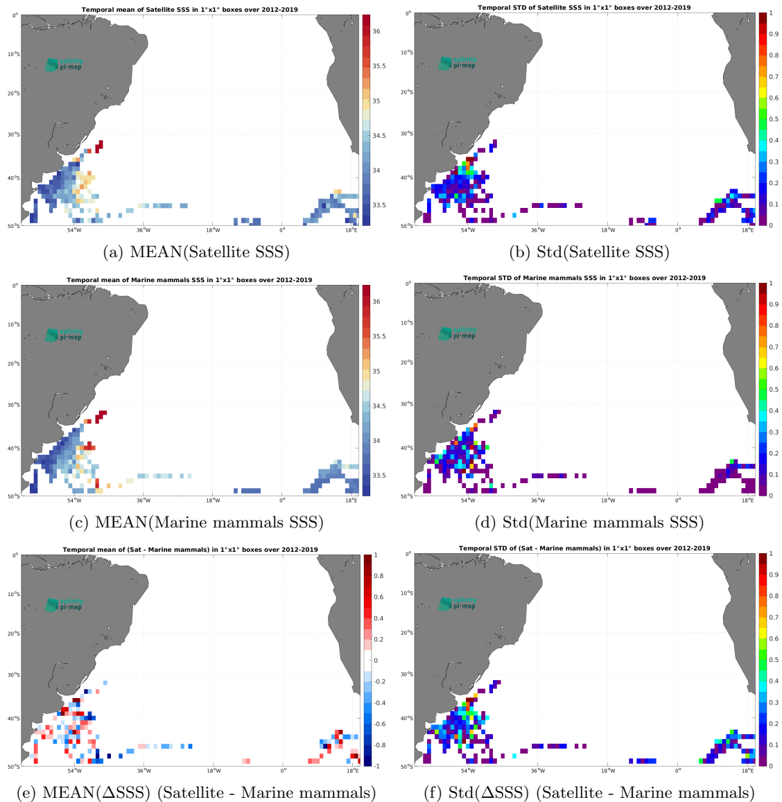
Figure 6: Temporal mean (left) and Std (right) of SSS from SMOS SSS L4 OI v342 - Weekly (CMEMS-CATDS-LOPS) (top), Marine mammals (middle), and of \Delta SSS (Satellite - Marine mammals). Only match-up pairs are used to generate these maps.
