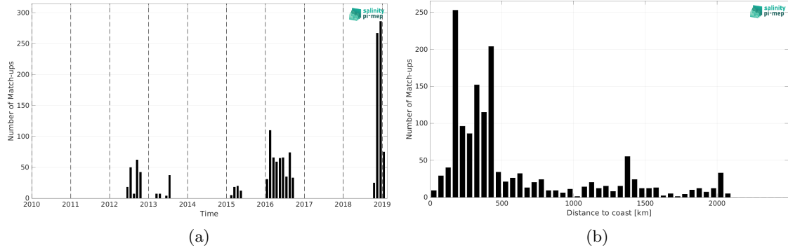
Figure 1: Number of match-ups between Marine mammals and SMOS SSS L4 OI v342 - Weekly (CMEMS-CATDS-LOPS) SSS as a function of time (a) and as function of the distance to coast (b) over the South Atlantic Ocean Pi-MEP region and for the full satellite product period.
