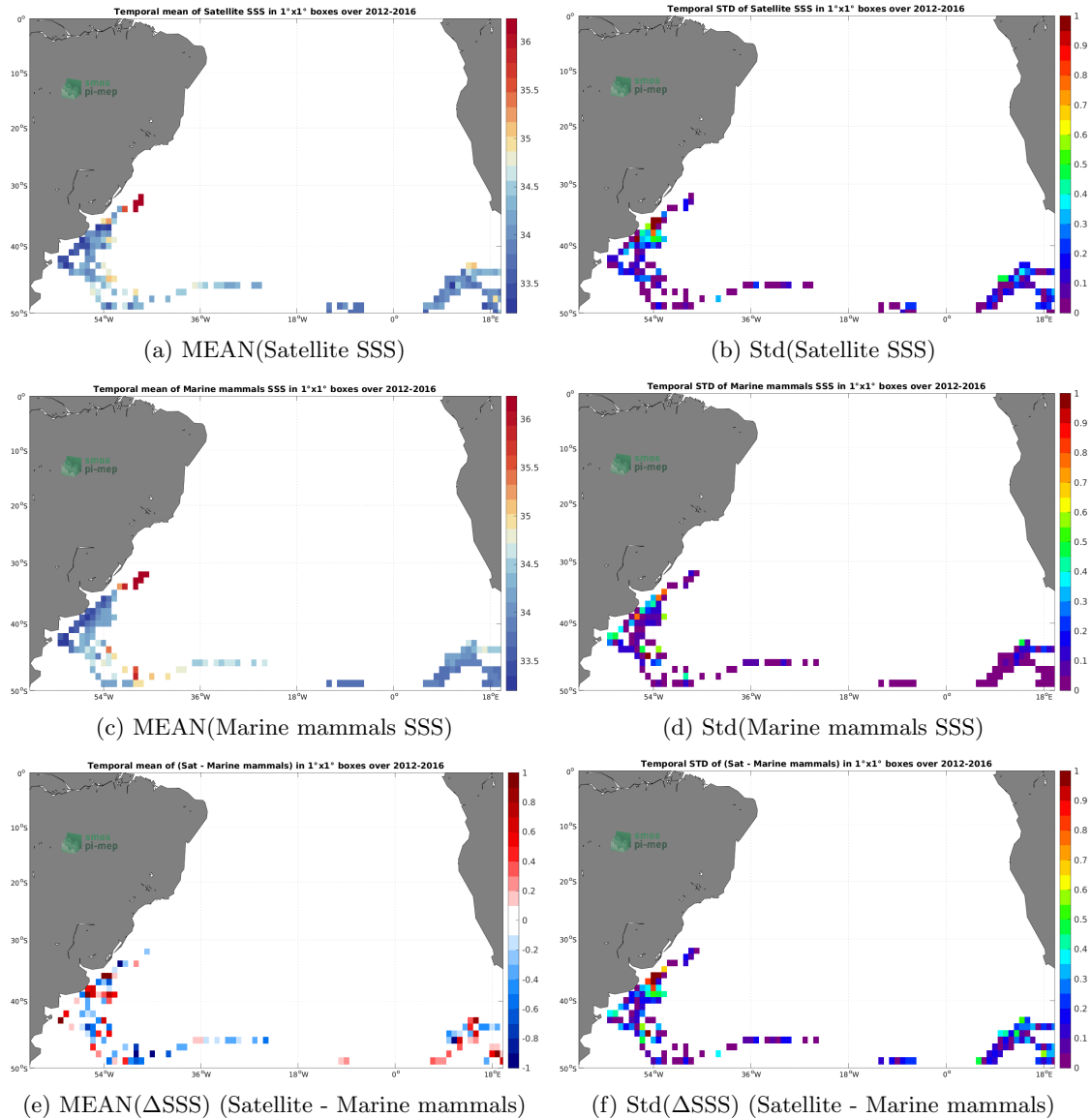
Figure 6: Temporal mean (left) and Std (right) of SSS from SMOS SSS L4 OI v342 - Weekly (CMEMS-CATDS-LOPS) (top), Marine mammals (middle), and of \Delta SSS (Satellite - Marine mammals). Only match-up pairs are used to generate these maps.
