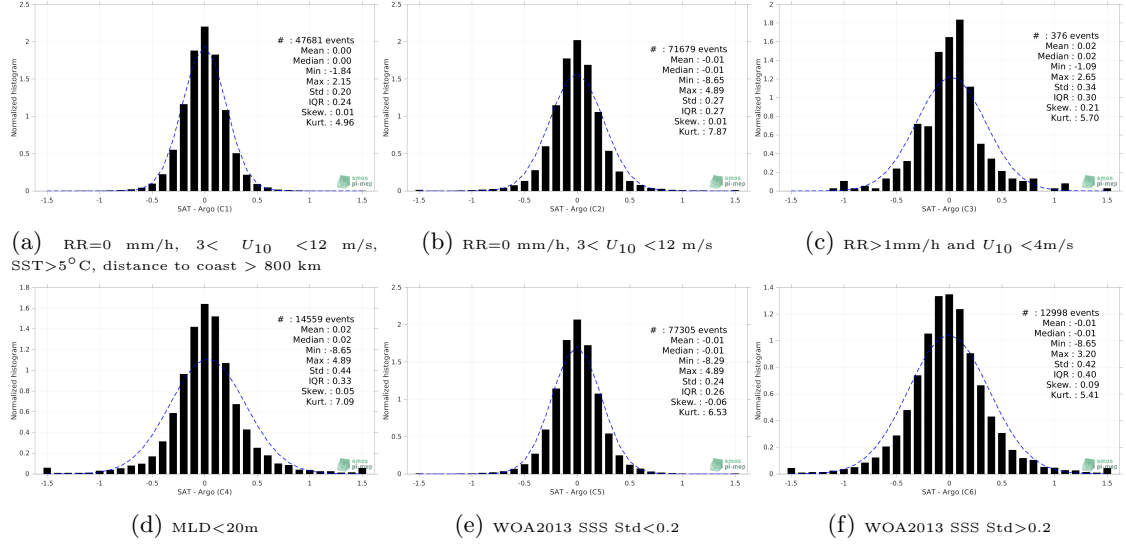
Figure 13: Normalized histogram of \Delta SSS (SMOS SSS L4 OI v342 - Weekly (CMEMS-CATDS-LOPS) - Argo) for 6 different subdatasets corresponding to: RR=0 mm/h, 3 < U_{10} < 12 m/s, SST>5°C, distance to coast > 800 km (a), RR=0 mm/h, 3 < U_{10} < 12 m/s (b), RR>1mm/h and U_{10} < 4 m/s (c), MLD<20m (d), WOA2013 SSS Std<0.2 (e), WOA2013 SSS Std>0.2 (f).
