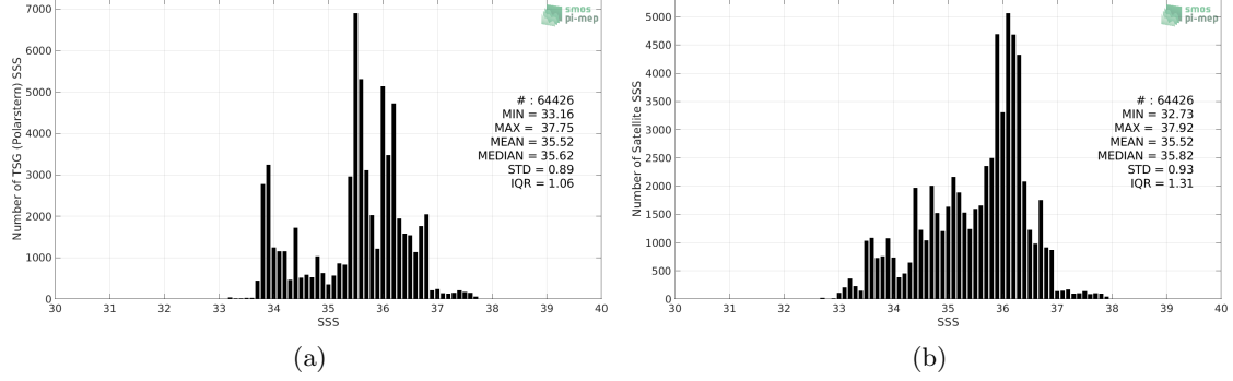
Figure 2: Histograms of SSS from TSG (Polarstern) (a) and SMOS L4 v2 Weekly (CATDS-CECOS-IFREMER) (b) considering all match-up pairs per bins of 0.1 over the South Atlantic Ocean Pi-MEP region and for the full satellite product period.
