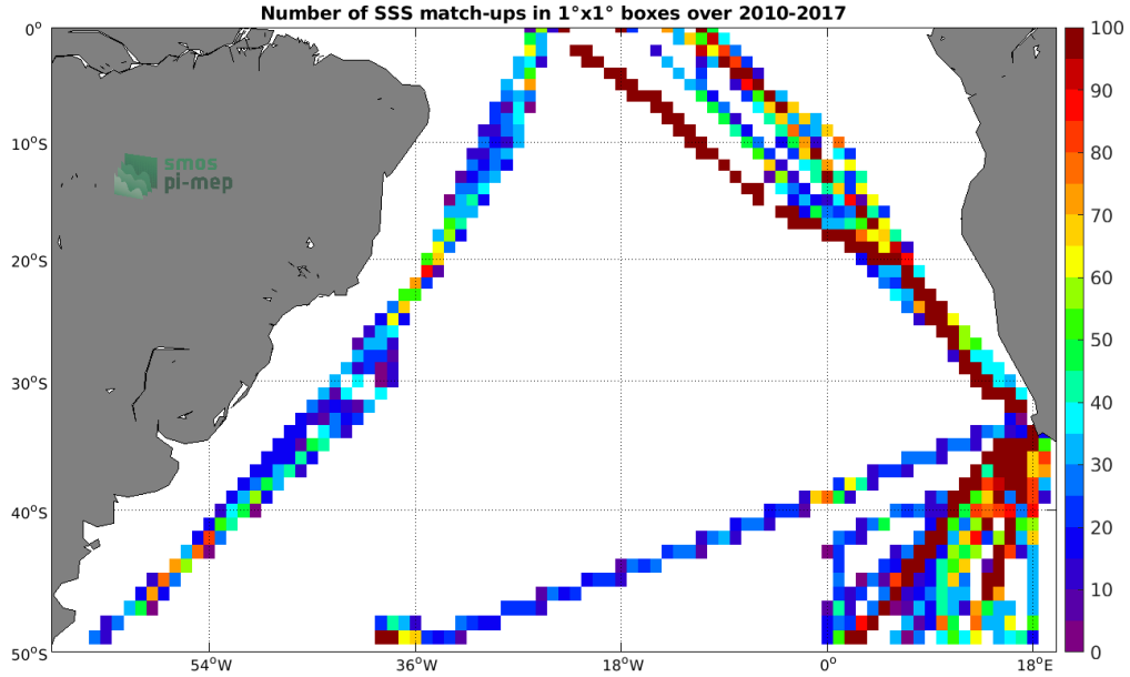
Figure 4: Number of SSS match-ups between TSG (Polarstern) SSS and the SMOS L4 v2 Weekly (CATDS-CECOS-IFREMER) SSS product for the South Atlantic Ocean Pi-MEP region over 1^\circ \times 1^\circ boxes and for the full satellite product period.
