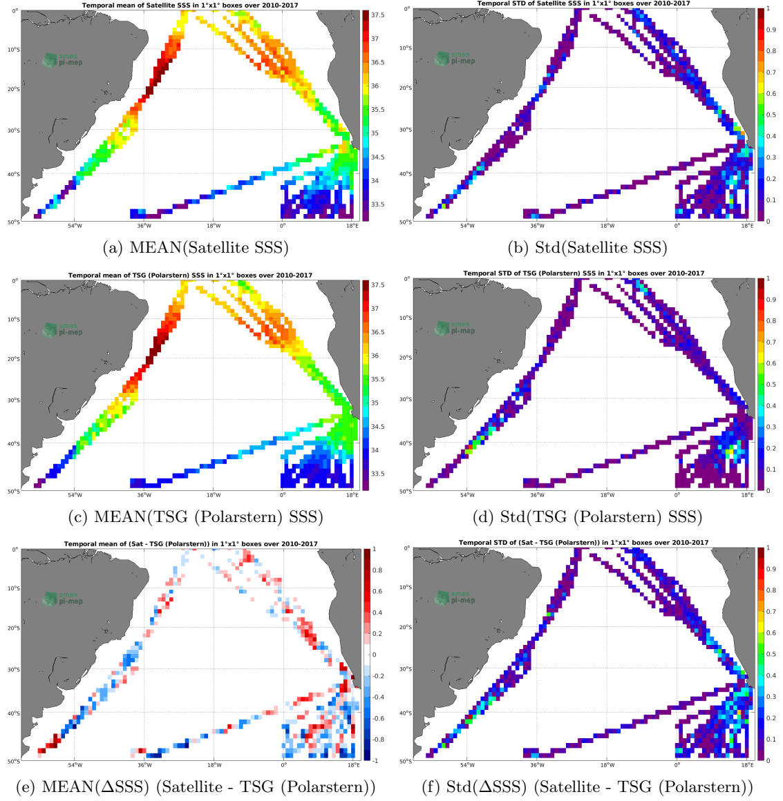
Figure 6: Temporal mean (left) and Std (right) of SSS from SMOS L4 v2 Weekly (CATDS-CECOS-IFREMER) (top), TSG (Polarstern) (middle), and of \Delta SSS (Satellite - TSG (Polarstern)). Only match-up pairs are used to generate these maps.
