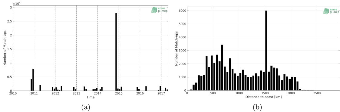
Figure 1: Number of match-ups between TSG (Polarstern) and SMOS L4 v2 Weekly (CATDS-CECOS-IFREMER) SSS as a function of time (a) and as function of the distance to coast (b) over the South Atlantic Ocean Pi-MEP region and for the full satellite product period.
