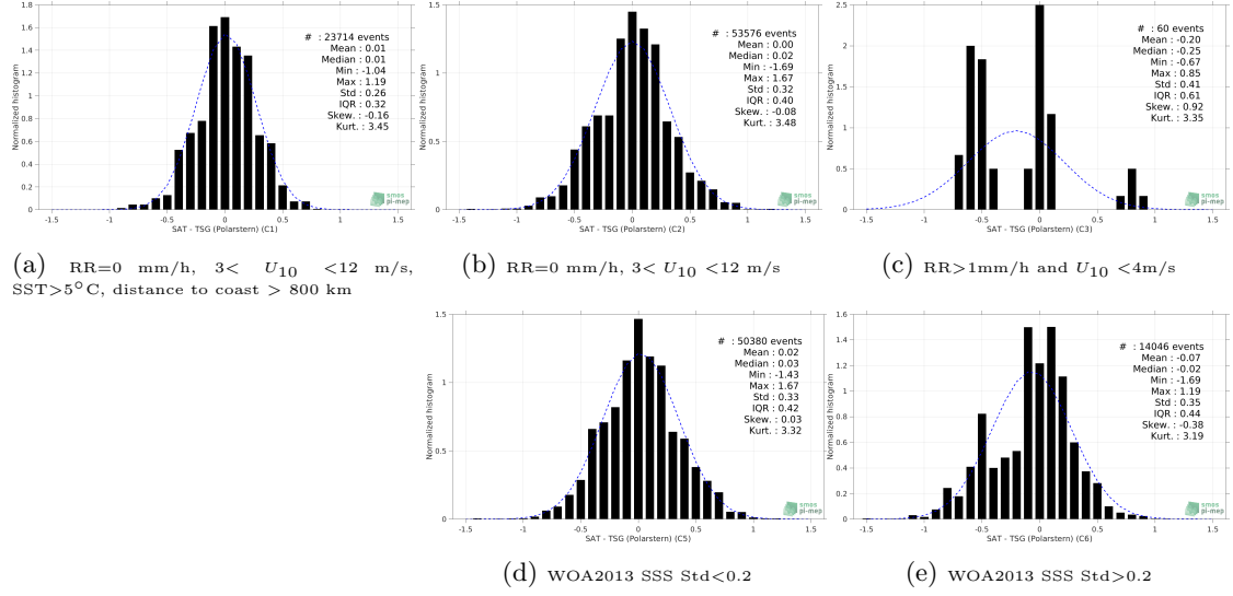
Figure 13: Normalized histogram of \Delta SSS (SMOS L4 v2 Weekly (CATDS-CECOS-IFREMER) - TSG (Polarstern)) for 5 different subdatasets corresponding to: RR=0 mm/h, 3 < U_{10} < 12 m/s, SST > 5°C, distance to coast > 800 km (a), RR=0 mm/h, 3 < U_{10} < 12 m/s (b), RR > 1 mm/h and U_{10} < 4 m/s (c), WOA2013 SSS Std < 0.2 (d), WOA2013 SSS Std > 0.2 (e).
