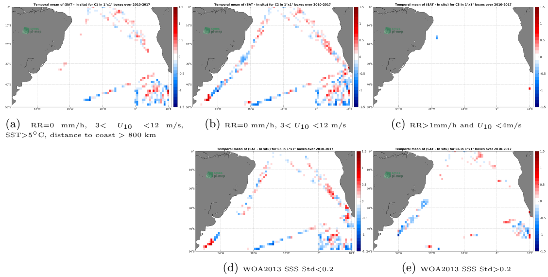
Figure 12: Temporal mean gridded over spatial boxes of size 1^\circ \times 1^\circ of \Delta SSS (SMOS L4 v2 Weekly (CATDS-CECOS-IFREMER) - TSG (Polarstern)) for 5 different subdatasets corresponding to: RR=0 mm/h, 3 < U_{10} < 12 m/s, SST > 5^\circ C , distance to coast > 800 km (a), RR=0 mm/h, 3 < U_{10} < 12 m/s (b), RR > 1 mm/h and U_{10} < 4 m/s (c), WOA2013 SSS Std < 0.2 (d), WOA2013 SSS Std > 0.2 (e).
