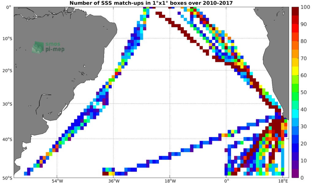
Figure 4: Number of SSS match-ups between TSG (Polarstern) SSS and the SMOS L4 v2 Weekly (CATDS-CECOS-IFREMER) SSS product for the South Atlantic Ocean Pi-MEP region over 1°x1° boxes and for the full satellite product period.
