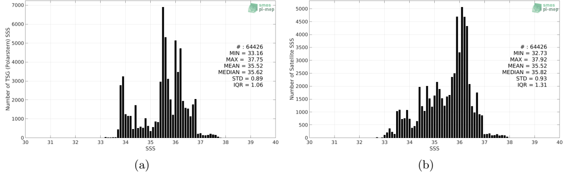
Figure 2: Histograms of SSS from TSG (Polarstern) (a) and SMOS L4 v2 Weekly (CATDS-CECOS-IFREMER) (b) considering all match-up pairs per bins of 0.1 over the South Atlantic Ocean Pi-MEP region and for the full satellite product period.
