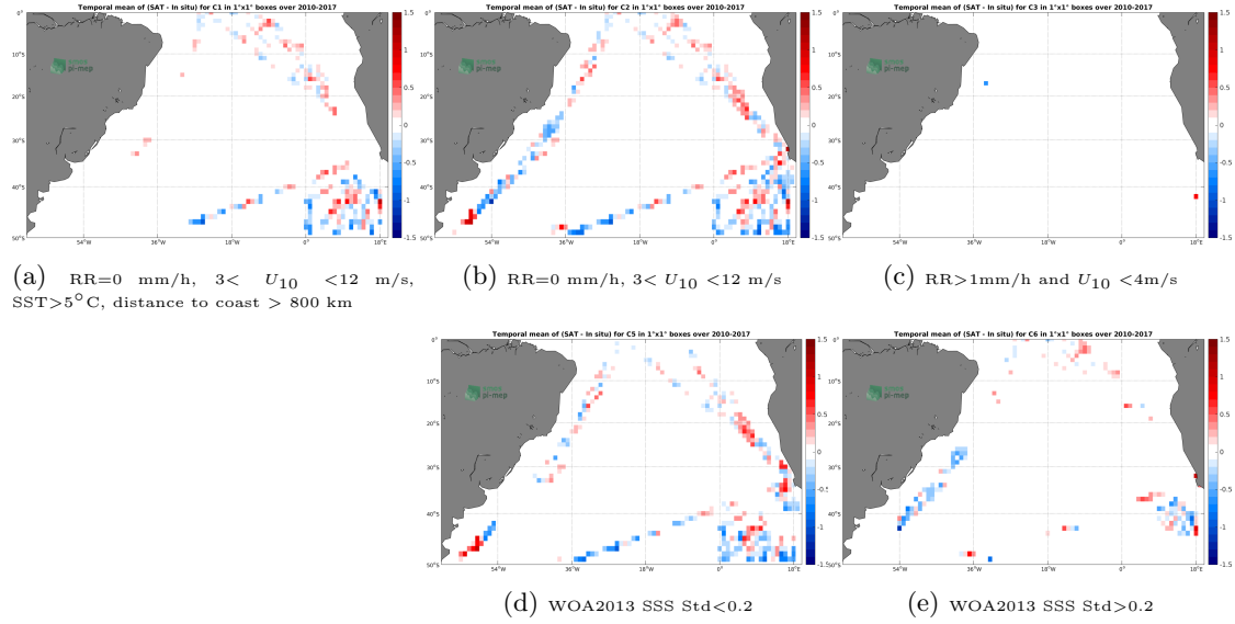
Figure 12: Temporal mean gridded over spatial boxes of size 1^\circ \times 1^\circ of \Delta SSS (SMOS-L4-CATDS-CECOS-IFREMER-V2-WEEKLY-0.5DEG - TSG-POLARSTERN) for 5 different subdatasets corresponding to: RR=0 mm/h, 3 < U_{10} < 12 m/s, SST > 5^\circ C , distance to coast > 800 km (a), RR=0 mm/h, 3 < U_{10} < 12 m/s (b), RR > 1 mm/h and U_{10} < 4 m/s (c), WOA2013 SSS Std < 0.2 (d), WOA2013 SSS Std > 0.2 (e).
