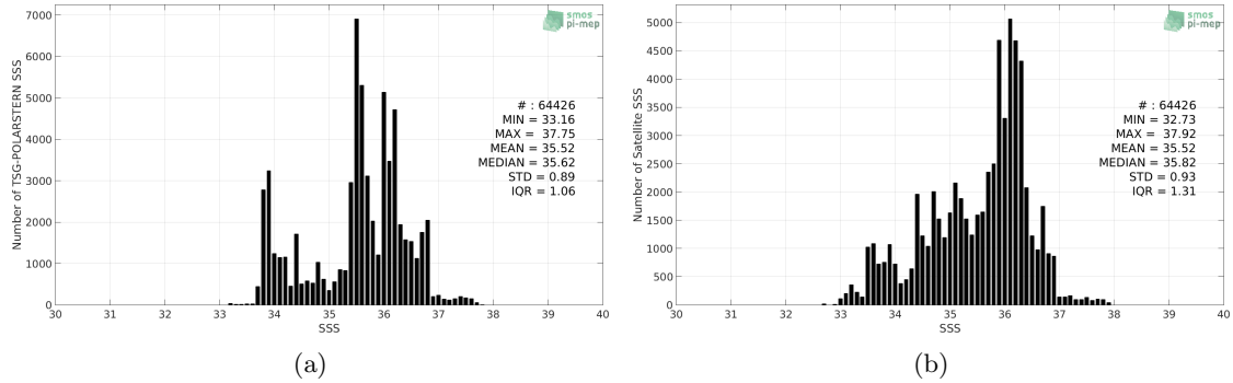
Figure 2: Histograms of SSS from TSG-POLARSTERN (a) and SMOS-L4-CATDS-CECOS-IFREMER-V2-WEEKLY-0.5DEG (b) considering all match-up pairs per bins of 0.1 over the South Atlantic Ocean Pi-MEP region and for the full satellite product period.
