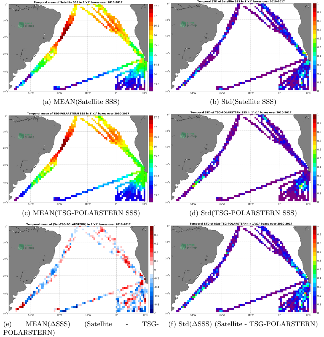
Figure 6: Temporal mean (left) and Std (right) of SSS from SMOS-L4-CATDS-CECOS-IFREMER-V2-WEEKLY-0.5DEG (top), TSG-POLARSTERN (middle), and of \Delta SSS (Satellite - TSG-POLARSTERN). Only match-up pairs are used to generate these maps.
