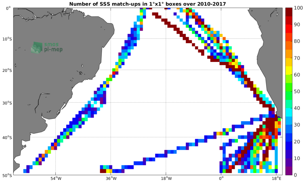
Figure 4: Number of SSS match-ups between TSG-POLARSTERN SSS and the SMOS-L4-CATDS-CECOS-IFREMER-V2-WEEKLY-0.5DEG SSS product for the South Atlantic Ocean Pi-MEP region over 1^\circ \times 1^\circ boxes and for the full satellite product period.
