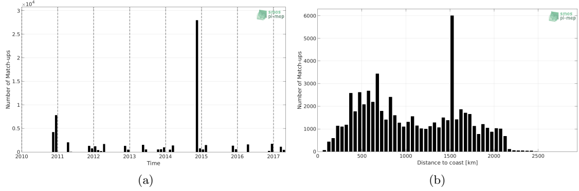
Figure 1: Number of match-ups between TSG-POLARSTERN and SMOS-L4-CATDS-CECOS-IFREMER-V2-WEEKLY-0.5DEG SSS as a function of time (a) and as function of the distance to coast (b) over the South Atlantic Ocean Pi-MEP region and for the full satellite product period.
