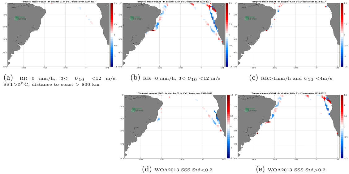
Figure 12: Temporal mean gridded over spatial boxes of size 1^{\circ}\times 1^{\circ} of \Delta\text{SSS} (SMOS L4 v2 Weekly (CATDS-CECOS-IFREMER) - TSG (LEGOS-DM)) for 5 different subdatasets corresponding to: \text{RR}=0 mm/h, 3 < U_{10} < 12 m/s, \text{SST} > 5^{\circ}\text{C} , distance to coast > 800 km (a), \text{RR}=0 mm/h, 3 < U_{10} < 12 m/s (b), \text{RR} > 1 mm/h and U_{10} < 4 m/s (c), WOA2013 SSS Std < 0.2 (d), WOA2013 SSS Std > 0.2 (e).
