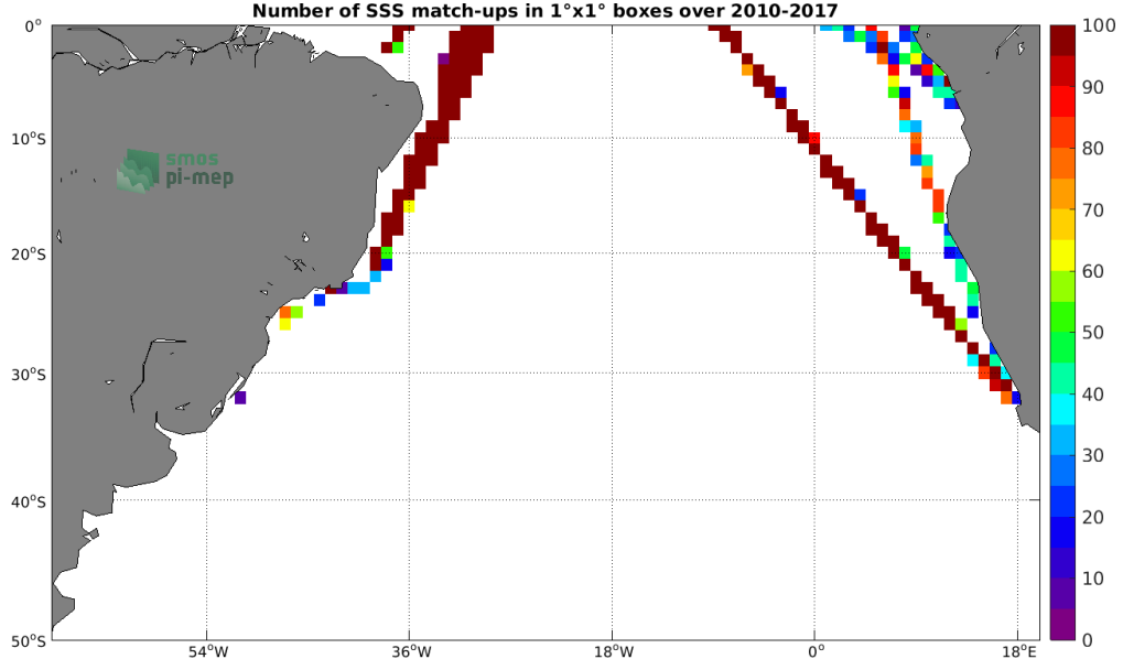
Figure 4: Number of SSS match-ups between TSG (LEGOS-DM) SSS and the SMOS L4 v2 Weekly (CATDS-CECOS-IFREMER) SSS product for the South Atlantic Ocean Pi-MEP region over 1^\circ \times 1^\circ boxes and for the full satellite product period.
