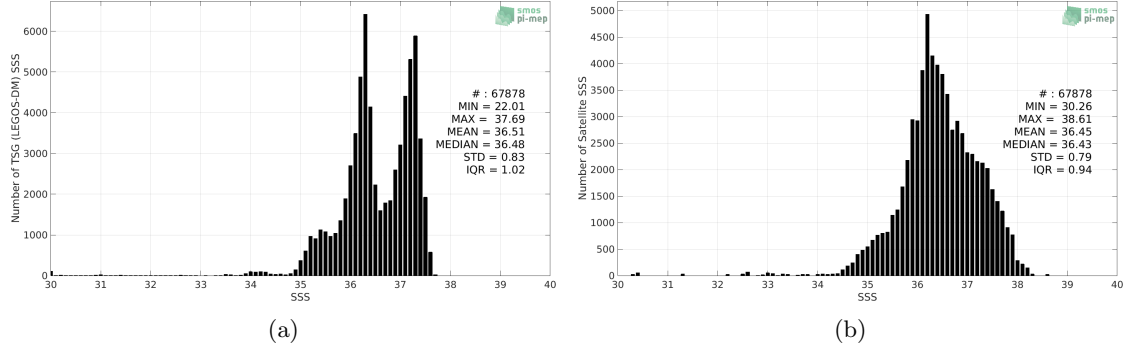
Figure 2: Histograms of SSS from TSG (LEGOS-DM) (a) and SMOS L4 v2 Weekly (CATDS-CECOS-IFREMER) (b) considering all match-up pairs per bins of 0.1 over the South Atlantic Ocean Pi-MEP region and for the full satellite product period.
