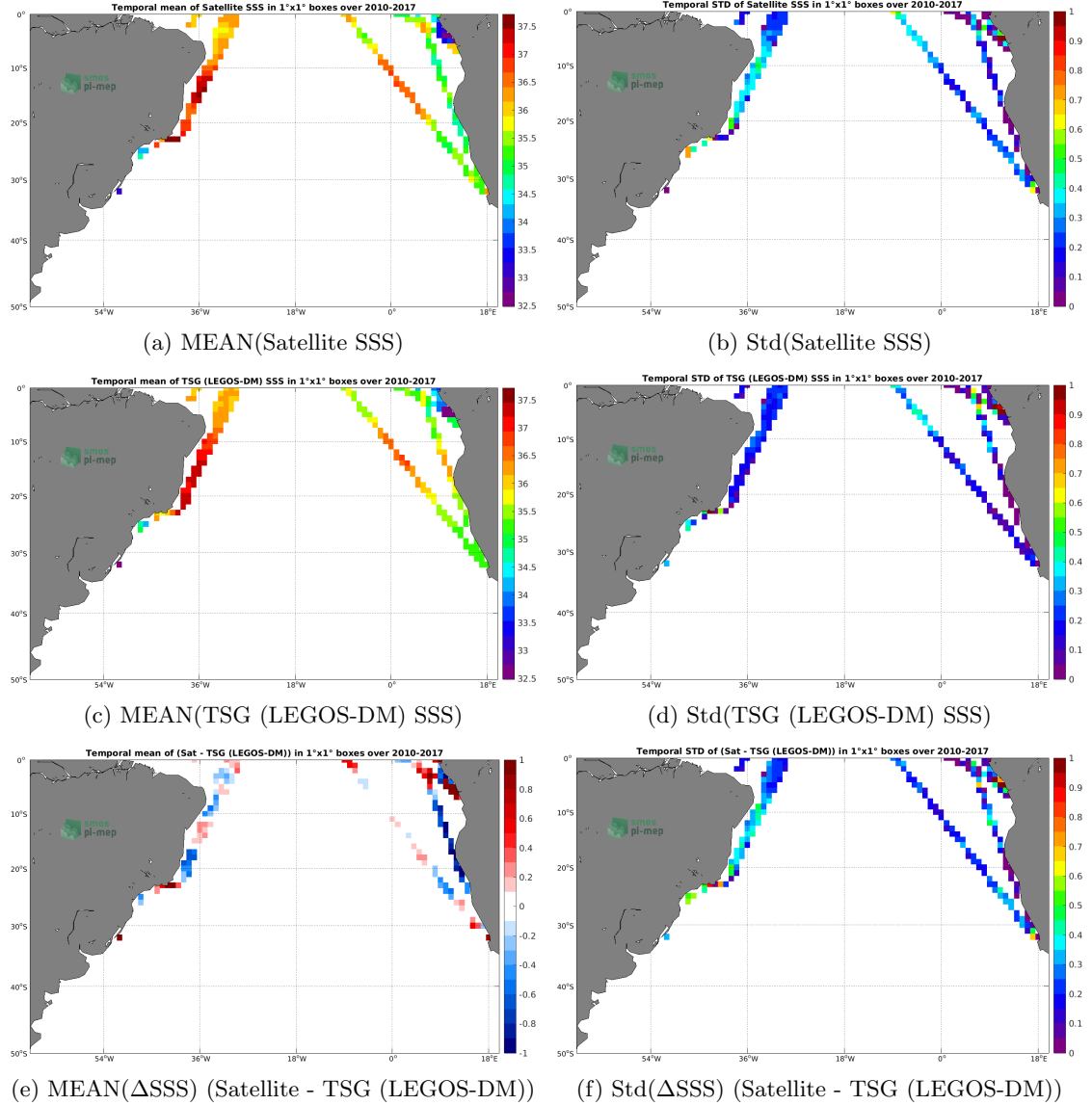
Figure 6: Temporal mean (left) and Std (right) of SSS from SMOS L4 v2 Weekly (CATDS-CECOS-IFREMER) (top), TSG (LEGOS-DM) (middle), and of \Delta SSS (Satellite - TSG (LEGOS-DM)). Only match-up pairs are used to generate these maps.
