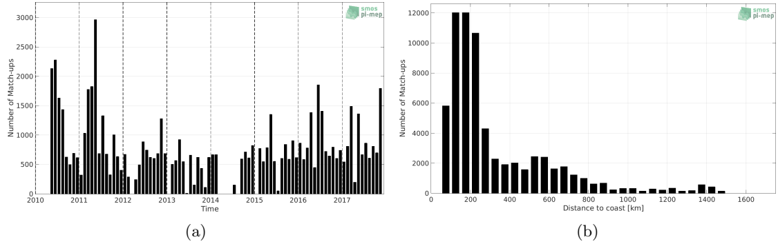
Figure 1: Number of match-ups between TSG (LEGOS-DM) and SMOS L4 v2 Weekly (CATDS-CECOS-IFREMER) SSS as a function of time (a) and as function of the distance to coast (b) over the South Atlantic Ocean Pi-MEP region and for the full satellite product period.
