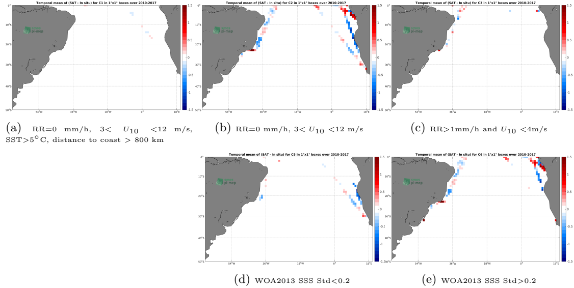
Figure 12: Temporal mean gridded over spatial boxes of size 1^{\circ}\times 1^{\circ} of \Delta\text{SSS} (SMOS-L4-CATDS-CECOS-IFREMER-V2-WEEKLY-0.5DEG - TSG-LEGOS-DM) for 5 different subdatasets corresponding to: \text{RR}=0 mm/h, 3 < U_{10} < 12 m/s, \text{SST} > 5^{\circ}\text{C} , distance to coast > 800 km (a), \text{RR}=0 mm/h, 3 < U_{10} < 12 m/s (b), \text{RR} > 1 mm/h and U_{10} < 4 m/s (c), WOA2013 SSS Std < 0.2 (d), WOA2013 SSS Std > 0.2 (e).
