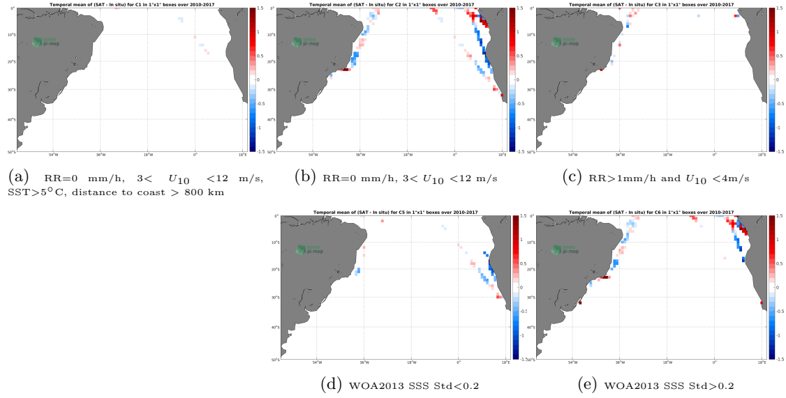
Figure 12: Temporal mean gridded over spatial boxes of size 1^\circ \times 1^\circ of \Delta SSS (SMOS-L4-CATDS-CECOS-IFREMER-V2-WEEKLY-0.5DEG - TSG-LEGOS-DM) for 5 different subdatasets corresponding to: RR=0 mm/h, 3 < U_{10} < 12 m/s, SST > 5^\circ\text{C} , distance to coast > 800 km (a), RR=0 mm/h, 3 < U_{10} < 12 m/s (b), RR > 1 mm/h and U_{10} < 4 m/s (c), WOA2013 SSS Std < 0.2 (d), WOA2013 SSS Std > 0.2 (e).
