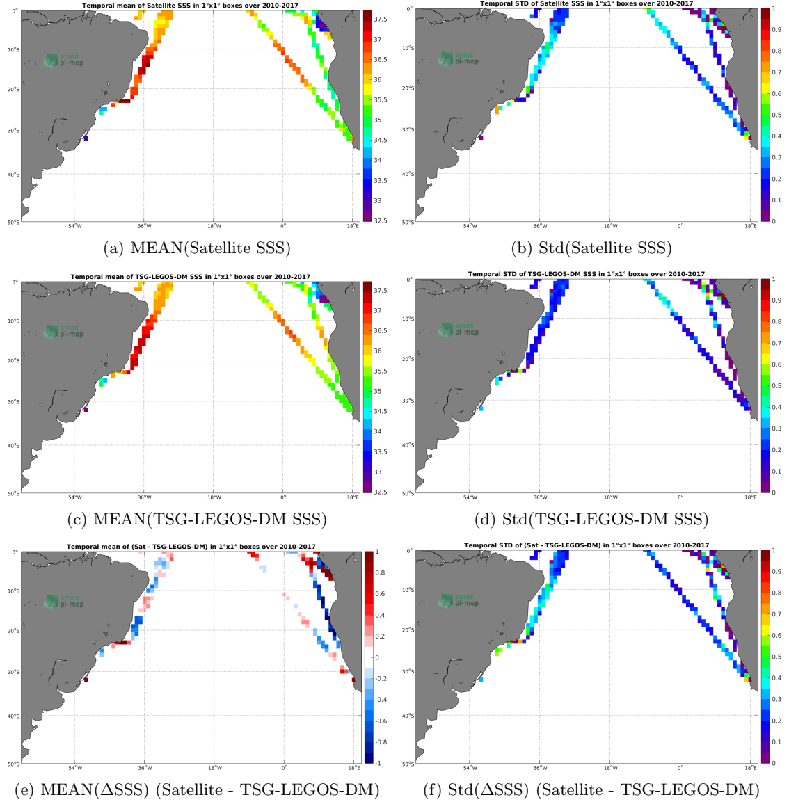
Figure 6: Temporal mean (left) and Std (right) of SSS from SMOS-L4-CATDS-CECOS-IFREMER-V2-WEEKLY-0.5DEG (top), TSG-LEGOS-DM (middle), and of \Delta SSS (Satellite - TSG-LEGOS-DM). Only match-up pairs are used to generate these maps.
