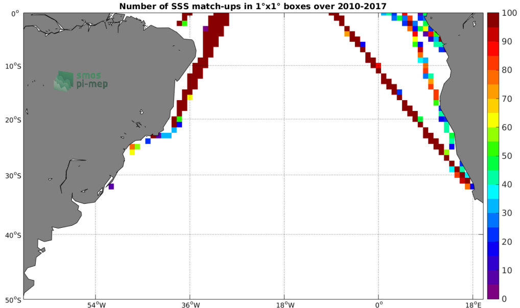
Figure 4: Number of SSS match-ups between TSG-LEGOS-DM SSS and the SMOS-L4-CATDS-CECOS-IFREMER-V2-WEEKLY-0.5DEG SSS product for the South Atlantic Ocean Pi-MEP region over 1^\circ \times 1^\circ boxes and for the full satellite product period.
