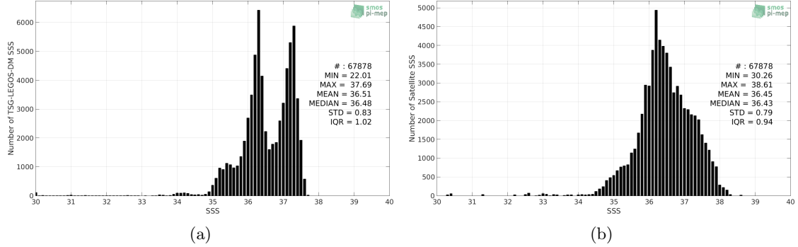
Figure 2: Histograms of SSS from TSG-LEGOS-DM (a) and SMOS-L4-CATDS-CECOS-IFREMER-V2-WEEKLY-0.5DEG (b) considering all match-up pairs per bins of 0.1 over the South Atlantic Ocean Pi-MEP region and for the full satellite product period.
