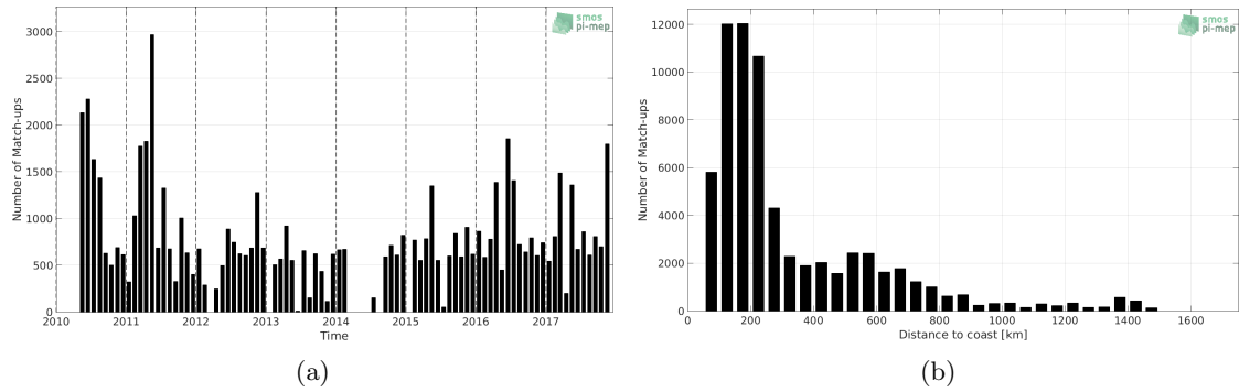
Figure 1: Number of match-ups between TSG-LEGOS-DM and SMOS-L4-CATDS-CECOS-IFREMER-V2-WEEKLY-0.5DEG SSS as a function of time (a) and as function of the distance to coast (b) over the South Atlantic Ocean Pi-MEP region and for the full satellite product period.
