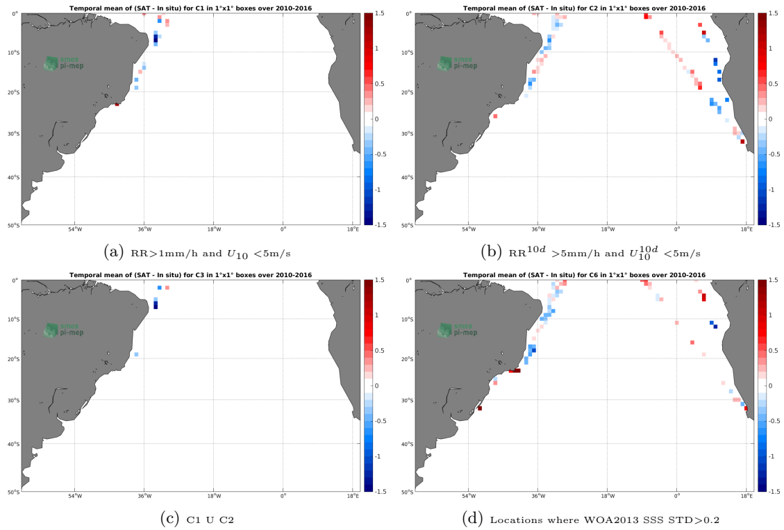
Figure 12: Temporal mean gridded over spatial boxes of size 1^\circ \times 1^\circ of \Delta SSS (SMOS-L4-CATDS-CECOS-IFREMER-V2-WEEKLY-0.5DEG - TSG-LEGOS-DM) for 4 different subdatasets corresponding to: RR > 1mm/h and U_{10} < 5\text{m/s} (a), RR^{10d} > 5\text{mm/h} and U_{10}^{10d} < 5\text{m/s} (b), C1 U C2 (c), Locations where WOA2013 SSS STD > 0.2 (d).
