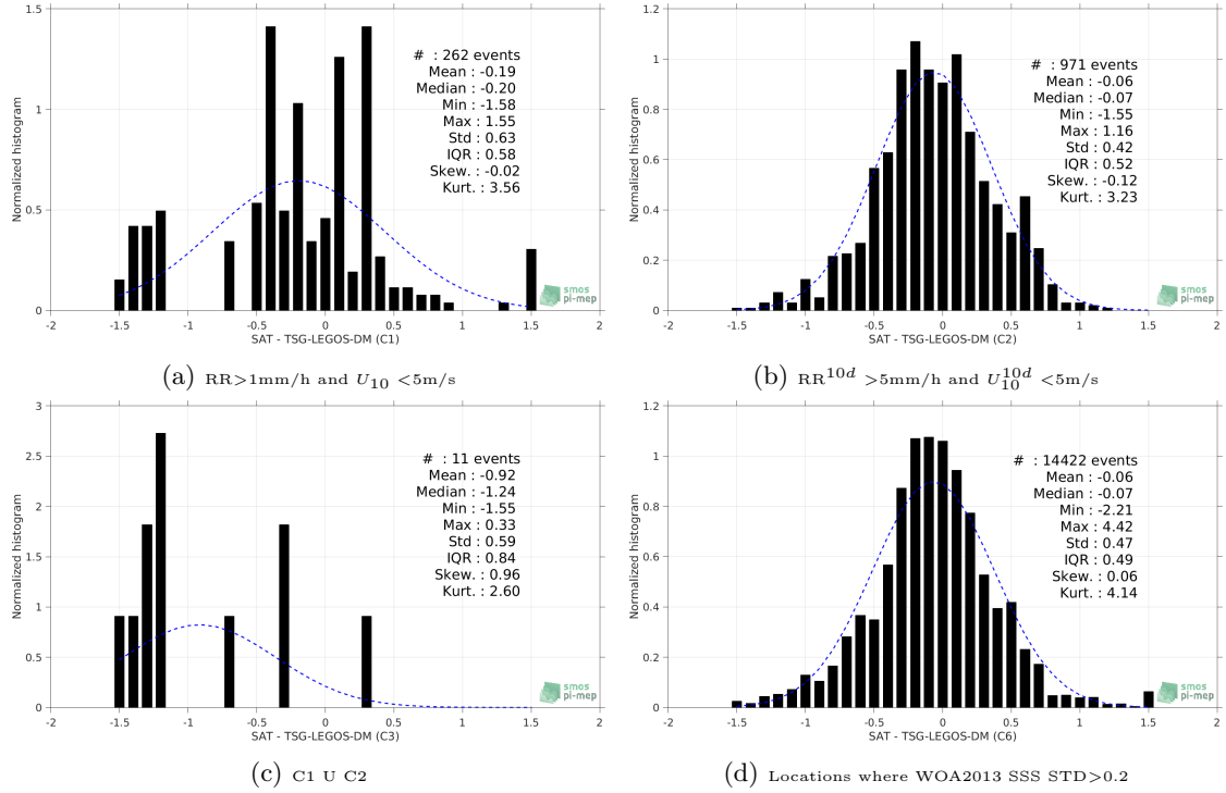
Figure 13: Normalized histogram of \Delta SSS (SMOS-L4-CATDS-CECOS-IFREMER-V2-WEEKLY-0.5DEG - TSG-LEGOS-DM) for 6 different subdatasets corresponding to: RR > 1\text{mm/h} and U_{10} < 5\text{m/s} (a), RR^{10d} > 5\text{mm/h} and U_{10}^{10d} < 5\text{m/s} (b), C1 U C2 (c), Locations where WOA2013 SSS STD > 0.2 (d).
