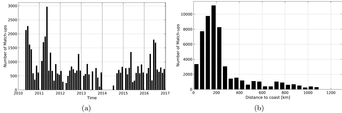
Figure 1: Number of match-ups between TSG-LEGOS-DM and SMOS-L4-CATDS-CECOS-IFREMER-V2-WEEKLY-0.5DEG SSS as a function of time (a) and as function of the distance to coast (b) over the South Atlantic Ocean Pi-MEP region and for the full satellite product period.
