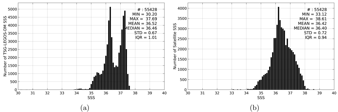
Figure 2: Histograms of SSS from TSG-LEGOS-DM (a) and SMOS-L4-CATDS-CECOS-IFREMER-V2-WEEKLY-0.5DEG (b) considering all match-up pairs per bins of 0.1 over the South Atlantic Ocean Pi-MEP region and for the full satellite product period.
