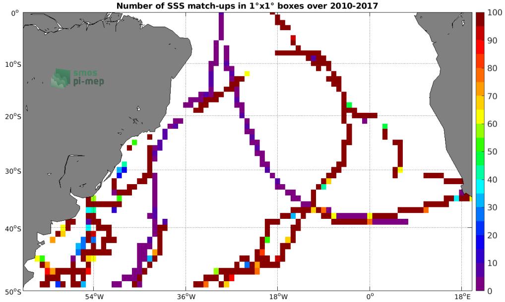
Figure 4: Number of SSS match-ups between TSG (GOSUD-Sailing-ship) SSS and the SMOS L4 v2 Weekly (CATDS-CECOS-IFREMER) SSS product for the South Atlantic Ocean Pi-MEP region over 1^\circ \times 1^\circ boxes and for the full satellite product period.
