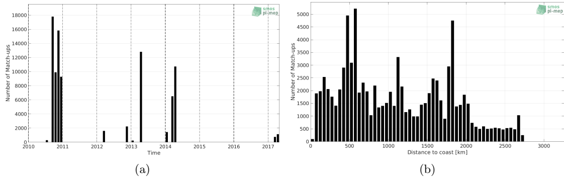
Figure 1: Number of match-ups between TSG (GOSUD-Sailing-ship) and SMOS L4 v2 Weekly (CATDS-CECOS-IFREMER) SSS as a function of time (a) and as function of the distance to coast (b) over the South Atlantic Ocean Pi-MEP region and for the full satellite product period.
