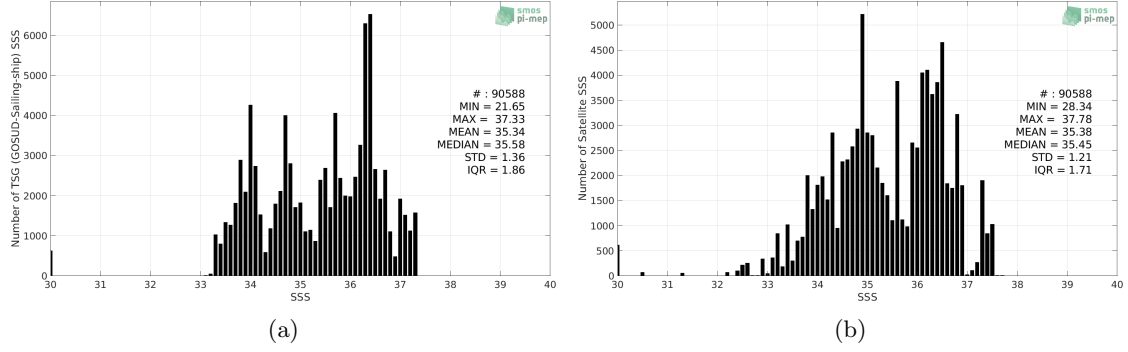
Figure 2: Histograms of SSS from TSG (GOSUD-Sailing-ship) (a) and SMOS L4 v2 Weekly (CATDS-CECOS-IFREMER) (b) considering all match-up pairs per bins of 0.1 over the South Atlantic Ocean Pi-MEP region and for the full satellite product period.
