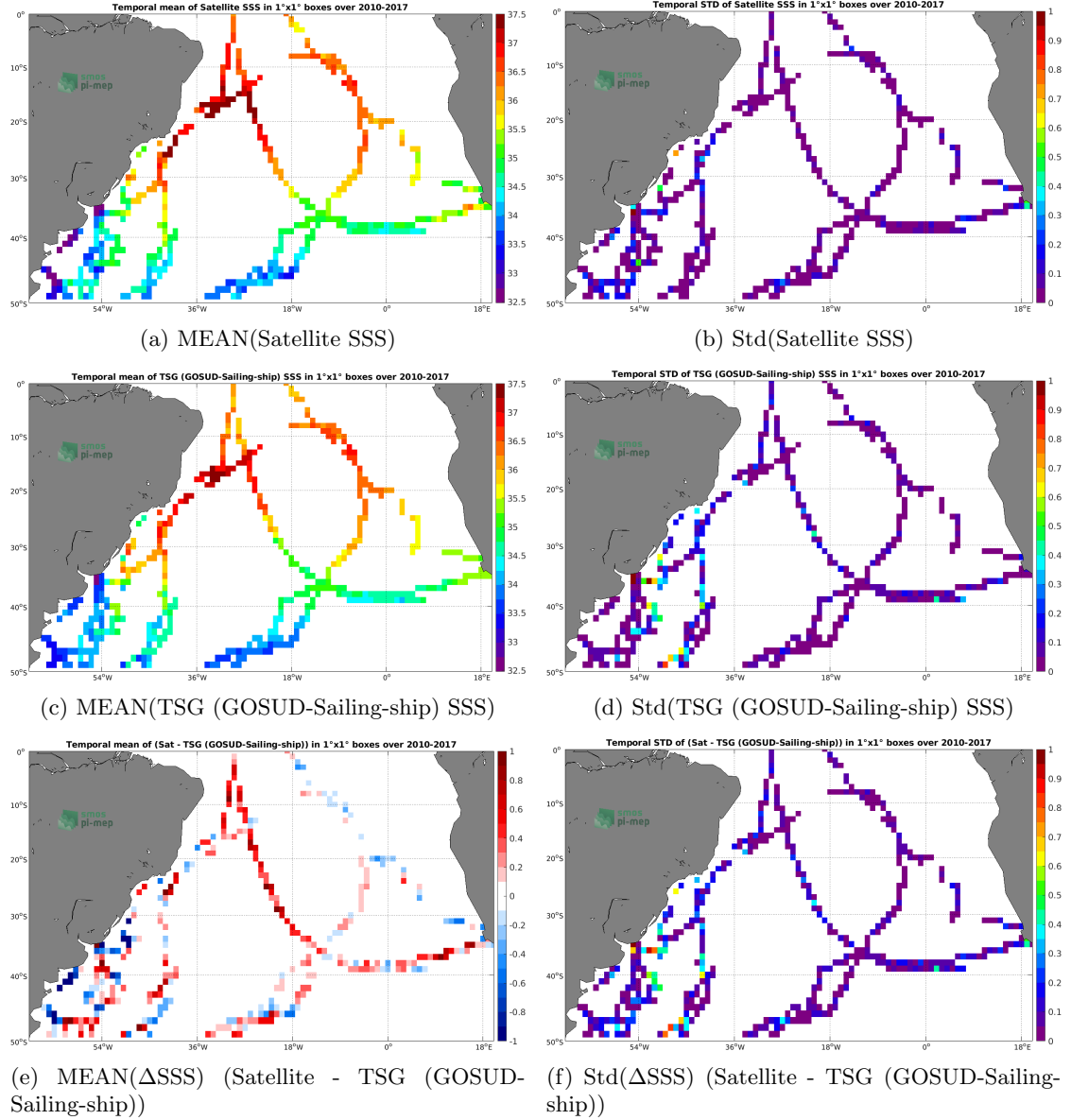
Figure 6: Temporal mean (left) and Std (right) of SSS from SMOS L4 v2 Weekly (CATDS-CECOS-IFREMER) (top), TSG (GOSUD-Sailing-ship) (middle), and of \Delta SSS (Satellite - TSG (GOSUD-Sailing-ship)). Only match-up pairs are used to generate these maps.
