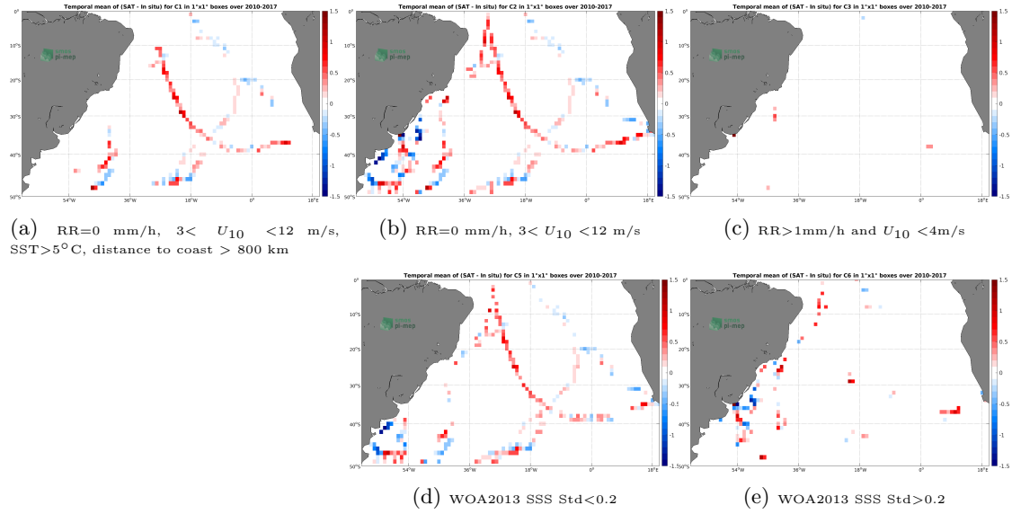
Figure 12: Temporal mean gridded over spatial boxes of size 1^\circ \times 1^\circ of \Delta SSS (SMOS L4 v2 Weekly (CATDS-CECOS-IFREMER) - TSG (GOSUD-Sailing-ship)) for 5 different subdatasets corresponding to:RR=0 mm/h, 3 < U_{10} < 12 m/s, SST >5^\circ\text{C} , distance to coast > 800 km (a), RR=0 mm/h, 3 < U_{10} < 12 m/s (b), RR >1 mm/h and U_{10} < 4 m/s (c), WOA2013 SSS Std <0.2 (d), WOA2013 SSS Std >0.2 (e).
