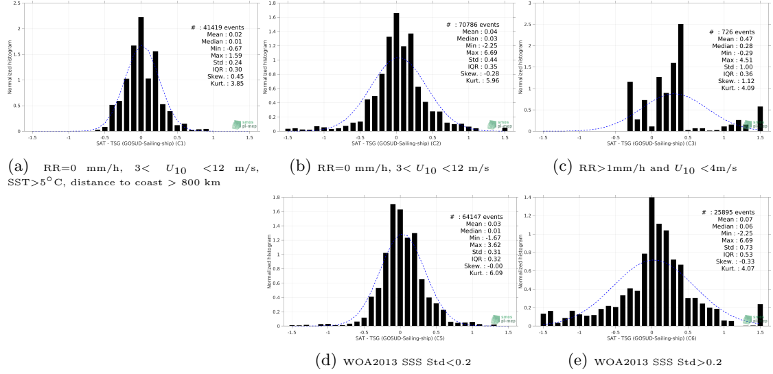
Figure 13: Normalized histogram of \Delta\text{SSS} (SMOS L4 v2 Weekly (CATDS-CECOS-IFREMER) - TSG (GOSUD-Sailing-ship)) for 5 different subdatasets corresponding to: RR=0 mm/h, 3 < U_{10} < 12 m/s, SST > 5^{\circ}\text{C} , distance to coast > 800 km (a), RR=0 mm/h, 3 < U_{10} < 12 m/s (b), RR > 1\text{mm/h} and U_{10} < 4\text{m/s} (c), WOA2013 SSS Std < 0.2 (d), WOA2013 SSS Std > 0.2 (e).
