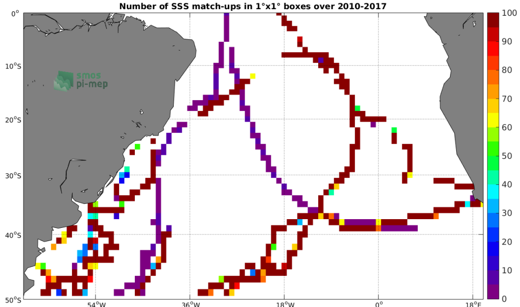
Figure 4: Number of SSS match-ups between TSG-GOSUD-Sailing-ship SSS and the SMOS-L4-CATDS-CECOS-IFREMER-V2-WEEKLY-0.5DEG SSS product for the South Atlantic Ocean Pi-MEP region over 1^\circ \times 1^\circ boxes and for the full satellite product period.
