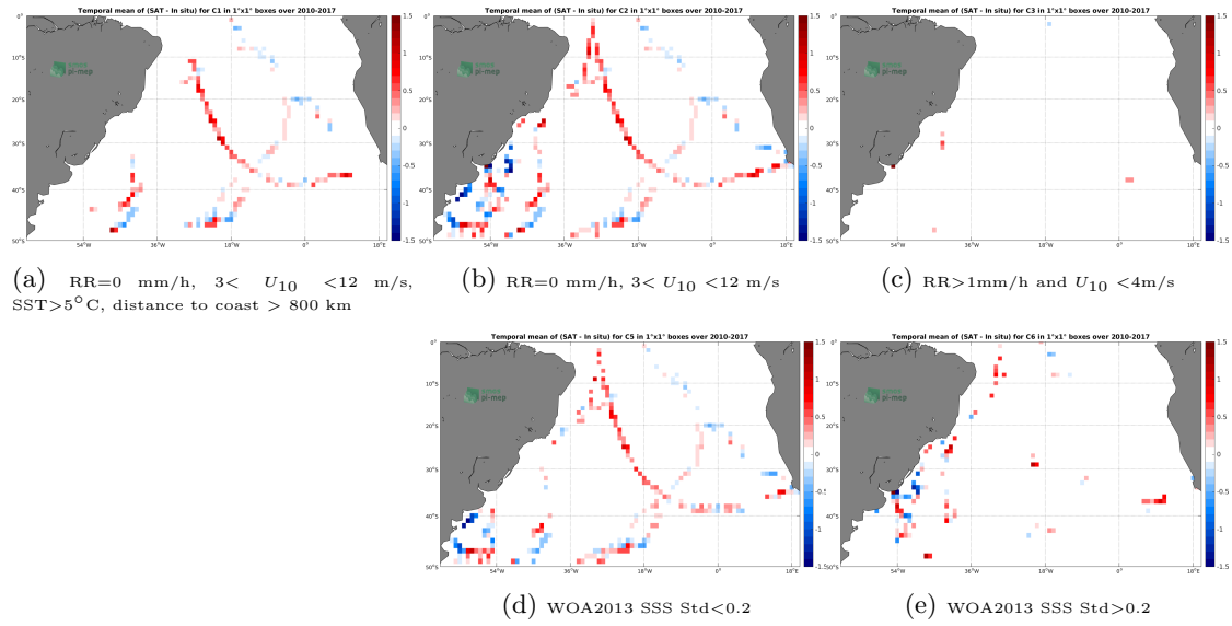
Figure 12: Temporal mean gridded over spatial boxes of size 1^\circ \times 1^\circ of \Delta SSS (SMOS-L4-CATDS-CECOS-IFREMER-V2-WEEKLY-0.5DEG - TSG-GOSUD-Sailing-ship) for 5 different subdatasets corresponding to: RR=0 mm/h, 3 < U_{10} < 12 m/s, SST > 5^\circ C , distance to coast > 800 km (a), RR=0 mm/h, 3 < U_{10} < 12 m/s (b), RR > 1 mm/h and U_{10} < 4 m/s (c), WOA2013 SSS Std < 0.2 (d), WOA2013 SSS Std > 0.2 (e).
