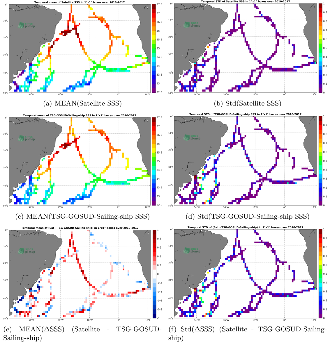
Figure 6: Temporal mean (left) and Std (right) of SSS from SMOS-L4-CATDS-CECOS-IFREMER-V2-WEEKLY-0.5DEG (top), TSG-GOSUD-Sailing-ship (middle), and of \Delta SSS (Satellite - TSG-GOSUD-Sailing-ship). Only match-up pairs are used to generate these maps.
