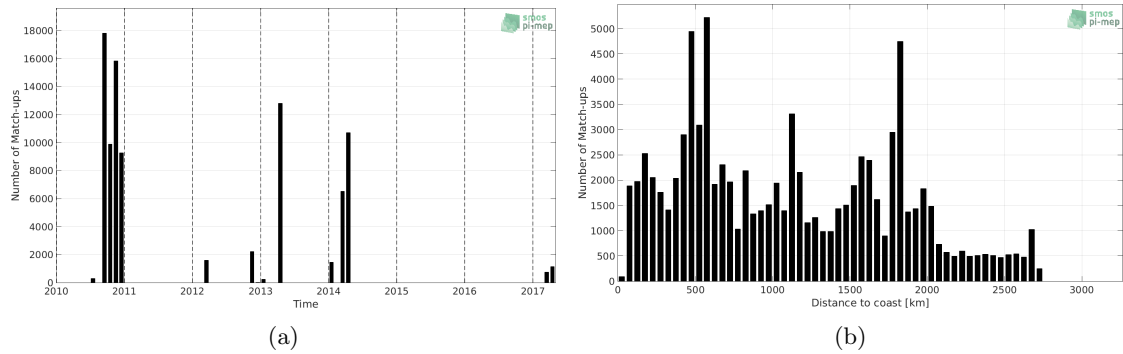
Figure 1: Number of match-ups between TSG-GOSUD-Sailing-ship and SMOS-L4-CATDS-CECOS-IFREMER-V2-WEEKLY-0.5DEG SSS as a function of time (a) and as function of the distance to coast (b) over the South Atlantic Ocean Pi-MEP region and for the full satellite product period.
