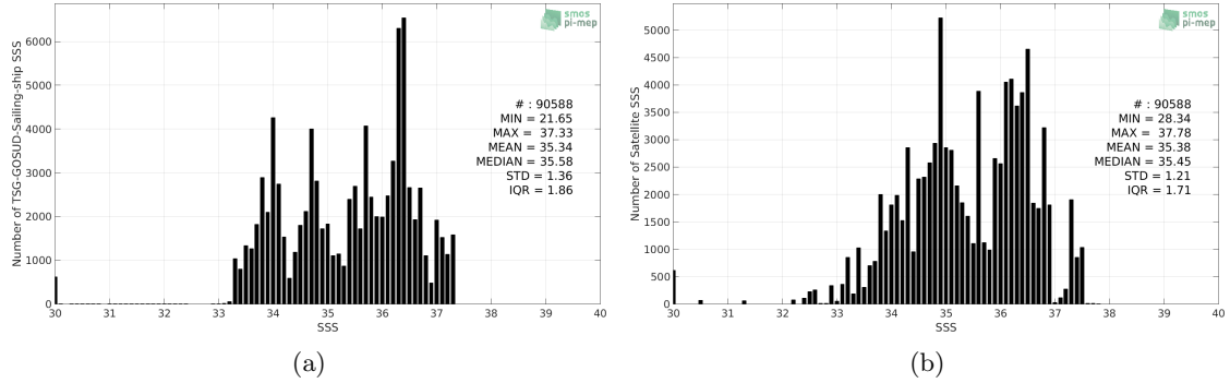
Figure 2: Histograms of SSS from TSG-GOSUD-Sailing-ship (a) and SMOS-L4-CATDS-CECOS-IFREMER-V2-WEEKLY-0.5DEG (b) considering all match-up pairs per bins of 0.1 over the South Atlantic Ocean Pi-MEP region and for the full satellite product period.
