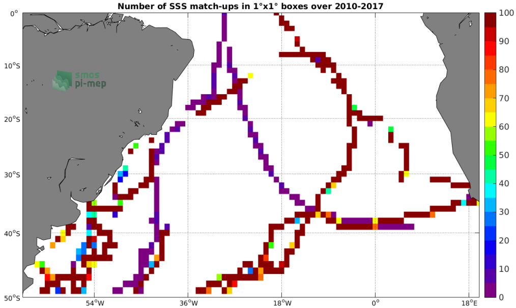
Figure 4: Number of SSS match-ups between TSG-GOSUD-Sailing-ship SSS and the SMOS-L4-CATDS-CECOS-IFREMER-V2-WEEKLY-0.5DEG SSS product for the South Atlantic Ocean Pi-MEP region over 1^\circ \times 1^\circ boxes and for the full satellite product period.
